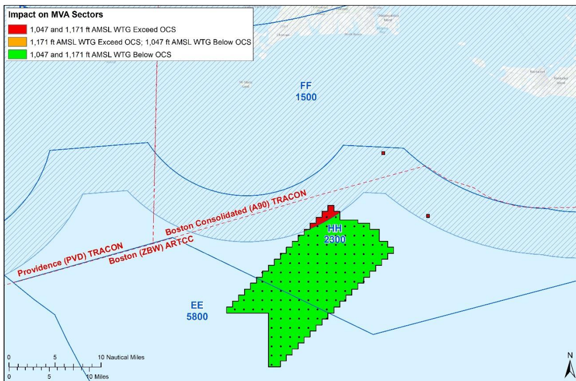
Figure 10: Boston Consolidated (A90) TRACON FUSION 5 MVA sectors (blue outline) with Sector FF obstacle evaluation area (hatched blue)
