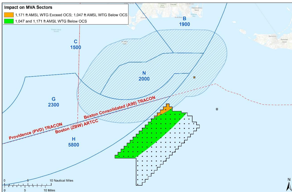
Figure 12: Providence (PVD) TRACON FUSION 5 MVA Sectors (blue outline) with Sector N obstacle evaluation area (hatched blue)
