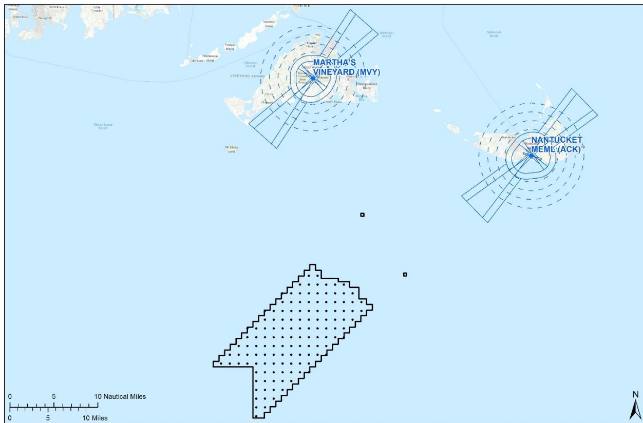
Figure 3: 77.17(a)(2) obstruction standard (dashed blue) and 77.19 imaginary surfaces (blue) in proximity to the SWDA
