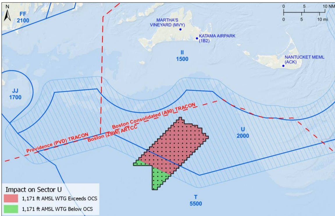
Figure 3: Boston Consolidated (A90) TRACON FUSION 3 MVA sectors (blue) with Sector U obstacle evaluation area (hatched blue)
