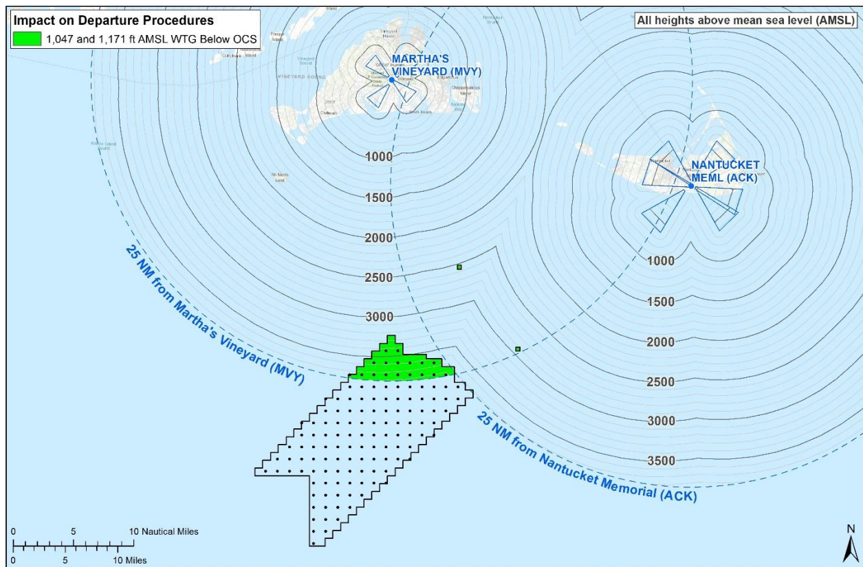
Figure 6: Martha's Vineyard (MVY) and Nantucket Memorial (ACK) obstacle departure procedure assessment (gray contours)
