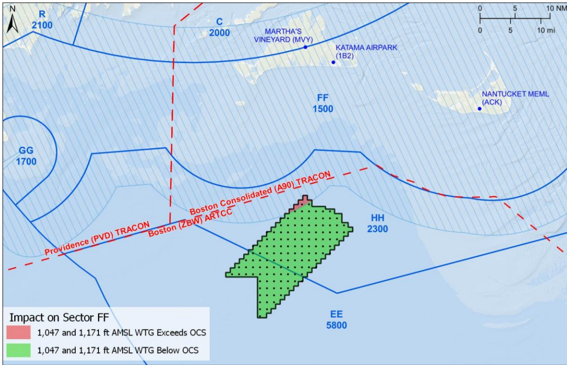
Figure 2: Boston Consolidated (A90) TRACON FUSION 5 MVA sectors (blue) with Sector FF obstacle evaluation area (hatched blue)
