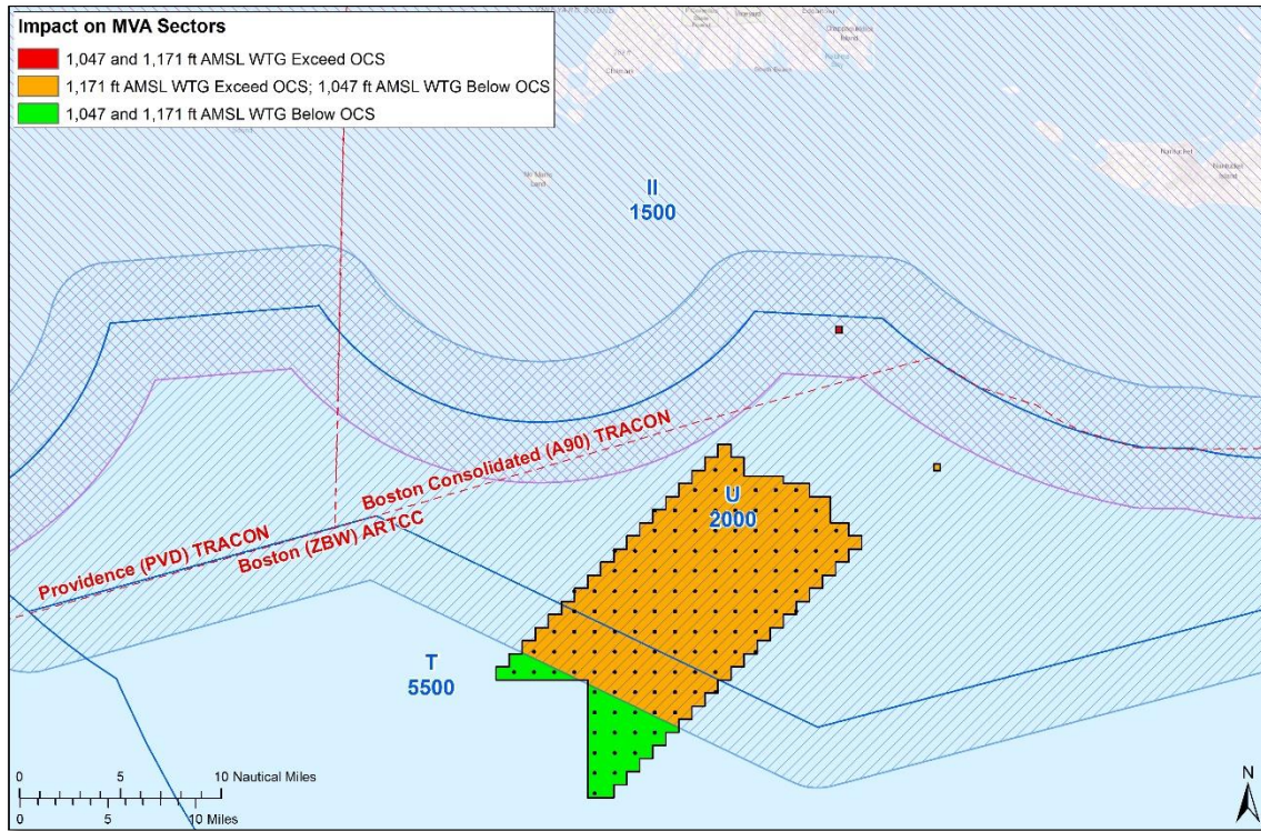
Figure 9: Boston Consolidated (A90) TRACON FUSION 3 MVA Sectors (blue outline) with Sector II (hatched purple) and Sector U (hatched blue) obstacle evaluation areas
