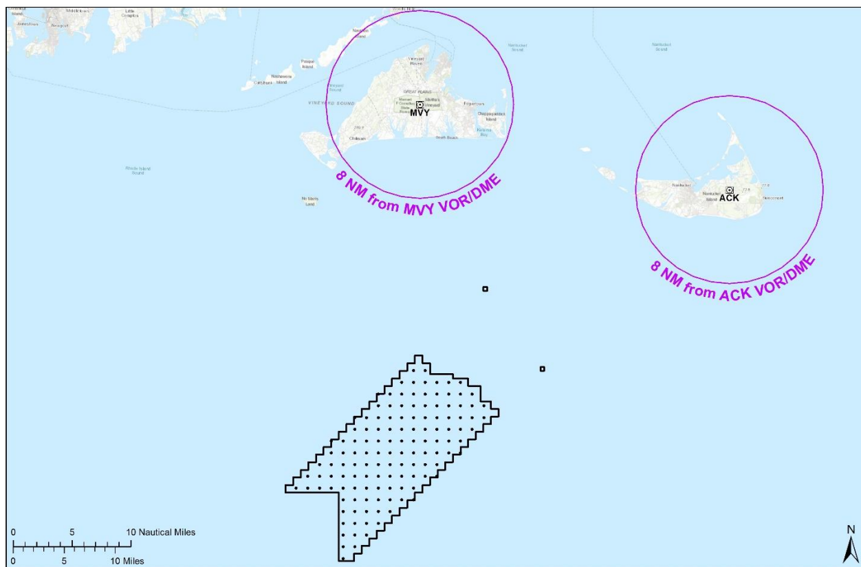
Figure 14: Martha's Vineyard (MVY) VOR/DME and Nantucket (ACK) VOR/DME protection areas (purple outline)
