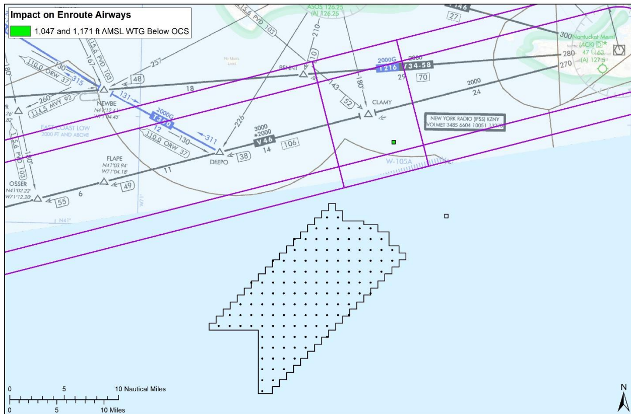
Figure 8: Low altitude enroute chart with V46 obstacle evaluation areas (purple outline)
