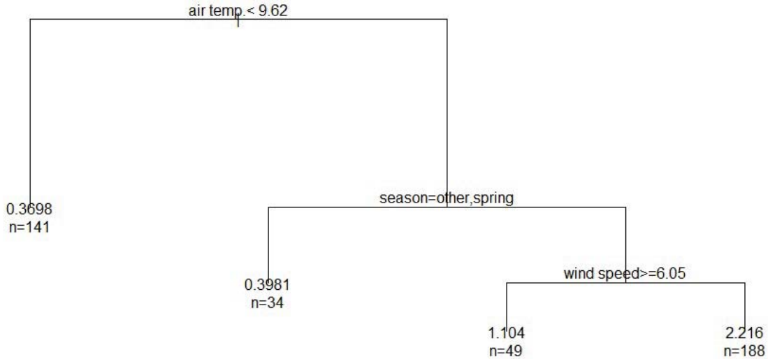
Figure 44. Regression tree for total nightly bat activity in Myotis bats ( Myotis spp. ). The numbers at the terminal nodes represent mean nightly bat activity (n=number of nights).
