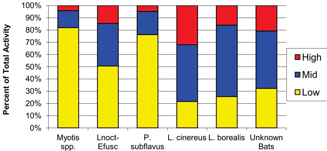
Figure 12. Distribution of Bat Activity by Species at Flat Rock Site (2007 and 2008 combined)
