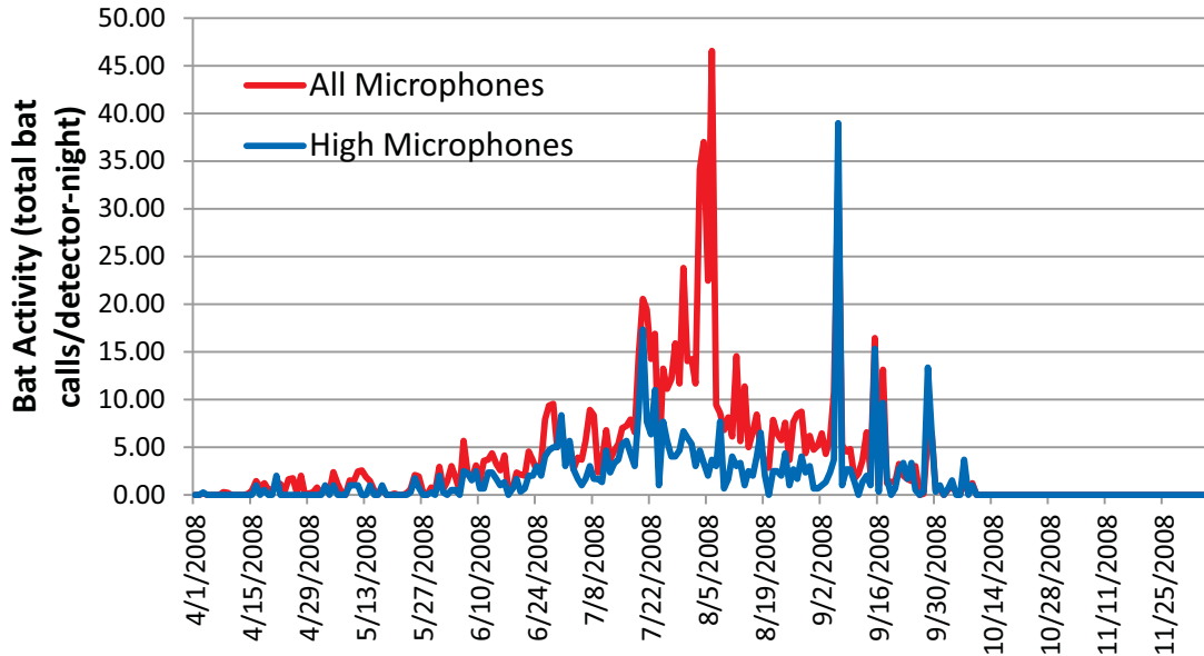
Figure 3. Seasonal Distribution in Bat Activity Across the MRWP Site, 2008
