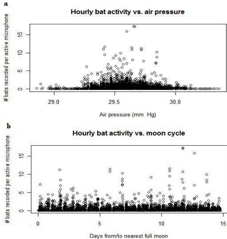
Figure 40. Interaction between hourly bat activity and (a) barometric pressure and (b) moon cycle.
