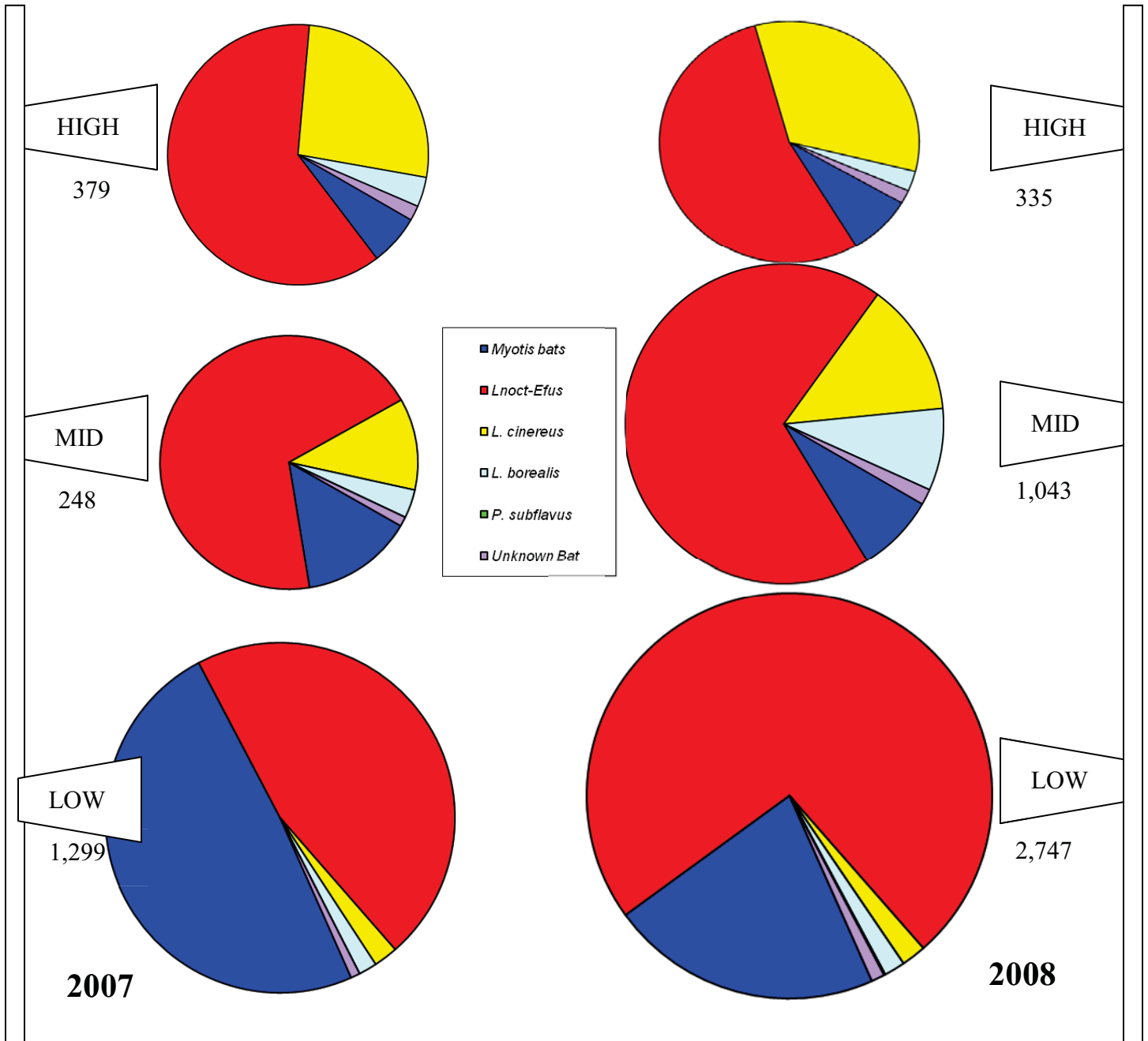
Figure 19. Distribution of Bat Activity across Microphone Heights at Cobb Site
