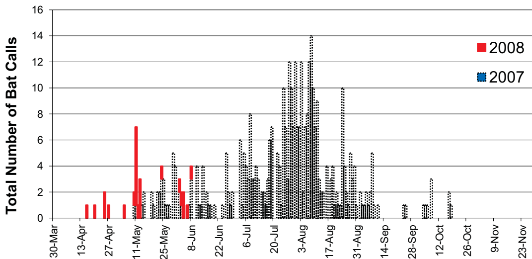
Figure 35. Temporal Distribution in Bat Activity at the Porter LOW Microphone
