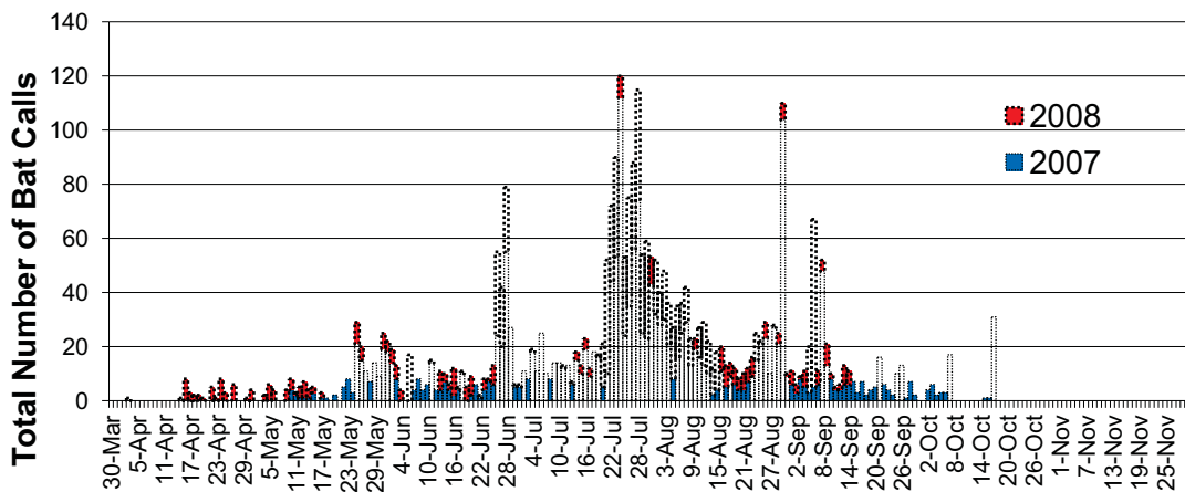
Figure 16. Temporal Distribution in Bat Activity at the Flat Rock MID Microphone (yellow bar represent high activity night where data bar was truncated to maintain overall pattern)
