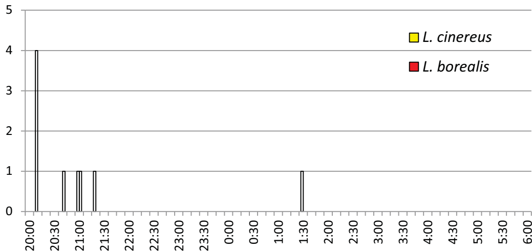
Figure 46. Temporal Distribution in Bat Activity from the Tethered Dirigible
