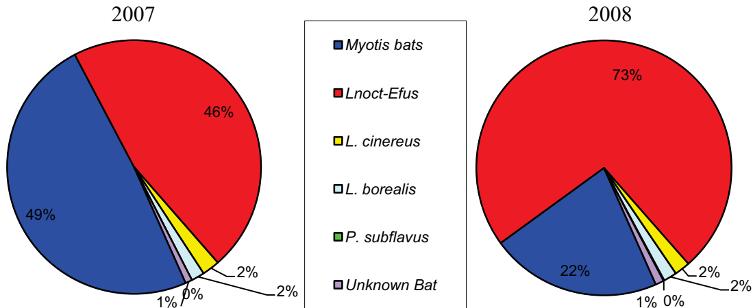
Figure 20. Distribution of Bat Activity by Species at the Cobb LOW Microphone
