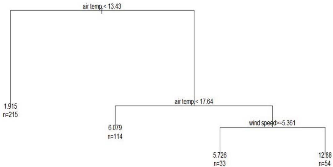
Figure 42. Regression tree for nightly bat activity. The numbers at the terminal nodes represent mean nightly bat activity (n=number of nights).
