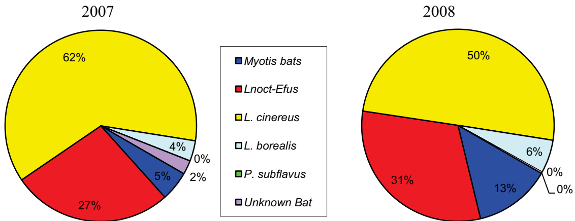
Figure 31. Distribution of Bat Activity by Species at the Gardner HIGH Microphone
