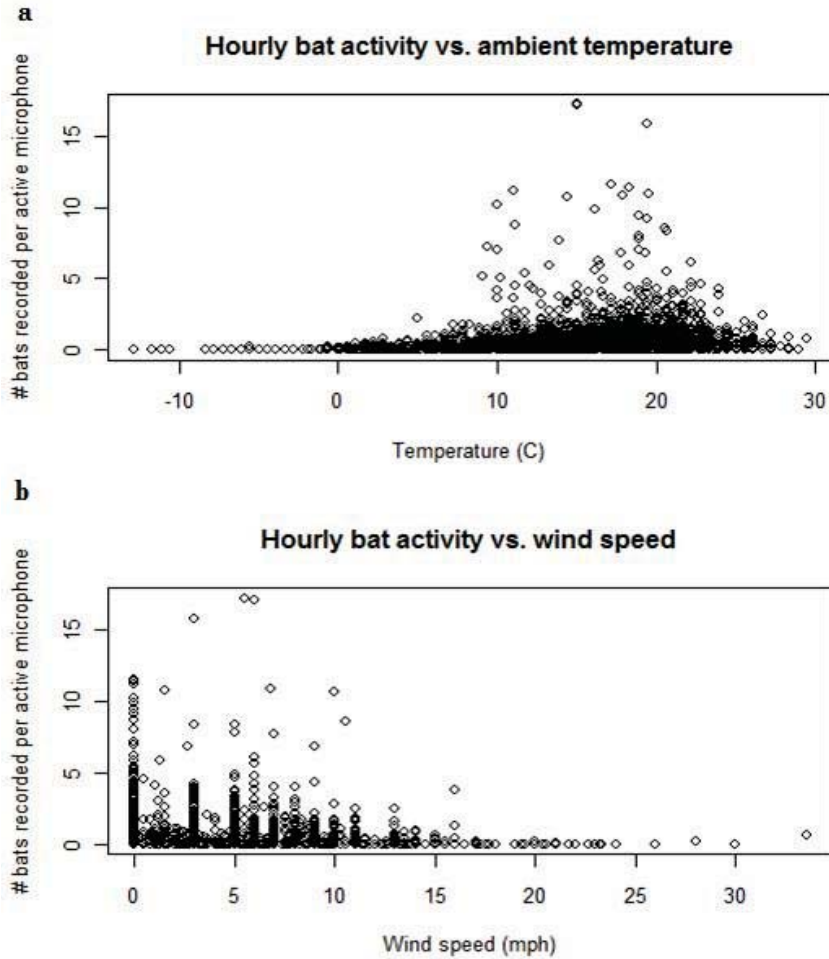
Figure 41. Interaction between hourly bat activity and (a) ambient temperature and (b) wind speed
