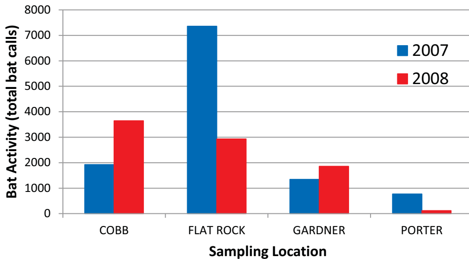
Figure 8. Spatial Variation in Bat Activity Relative to Sampling Location
