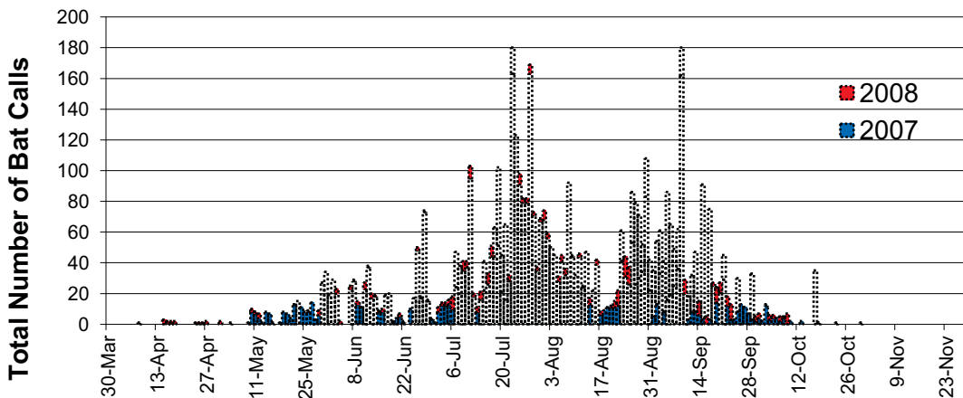
Figure 14. Temporal Distribution in Bat Activity at the Flat Rock LOW Microphone (yellow bars represent high activity nights where data bars were truncated to maintain overall patterns)
