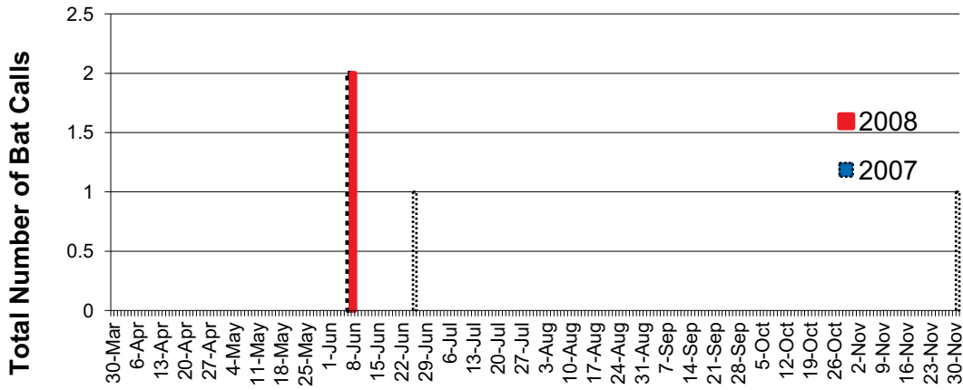
Figure 38. Temporal Distribution in Bat Activity at the Porter HIGH Microphone
