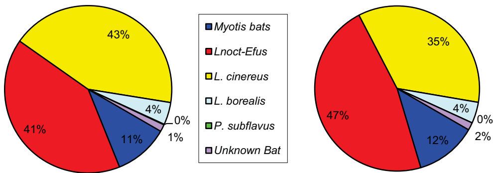
Figure 17. Distribution of Bat Activity by Species at the Flat Rock HIGH Microphone
