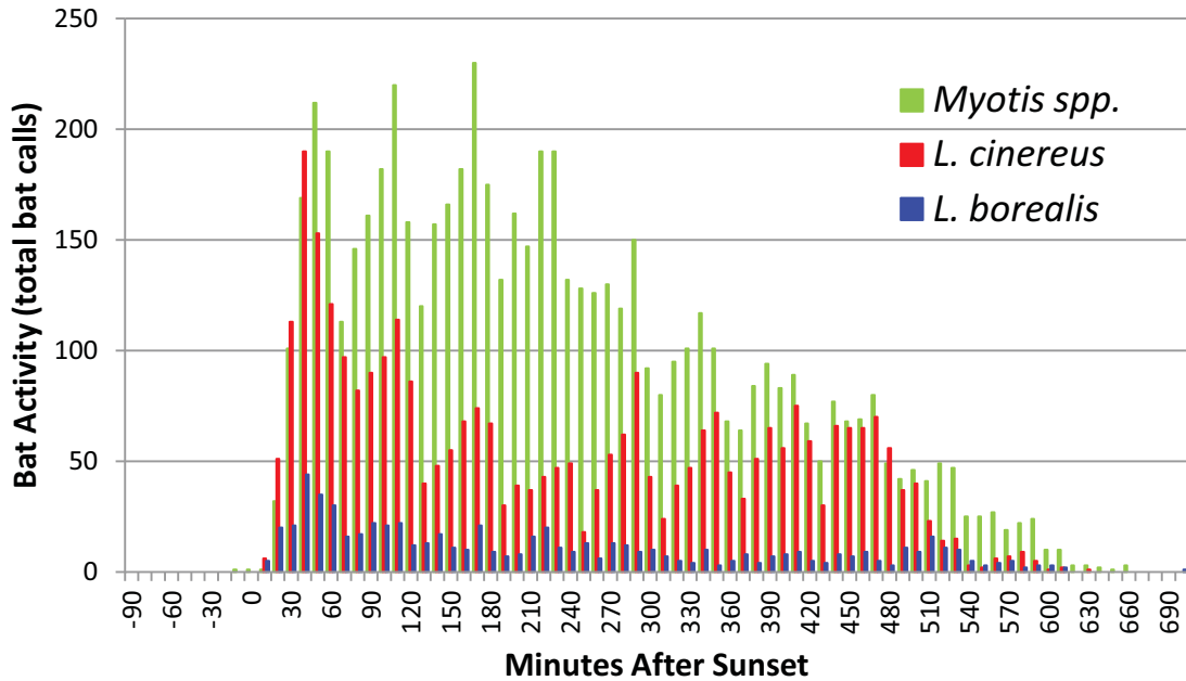
Figure 7. Temporal Variation in Bat Activity Relative to Sunset (both years combined)
