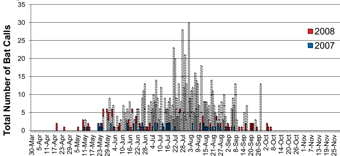
Figure 23. Temporal Distribution in Bat Activity at the Cobb MID Microphone
