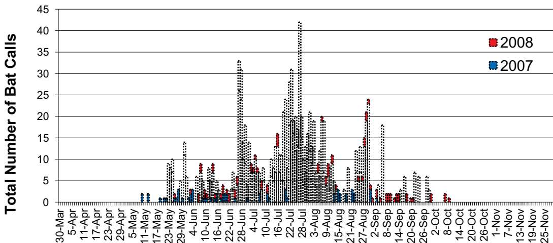
Figure 32. Temporal Distribution in Bat Activity at the Gardner HIGH Microphone
