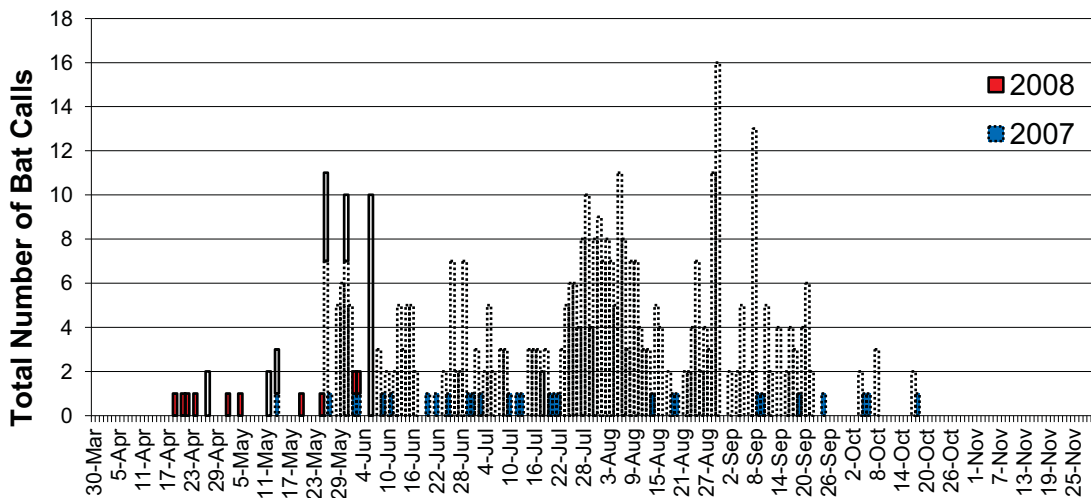
Figure 37. Temporal Distribution in Bat Activity at the Porter MID Microphone
