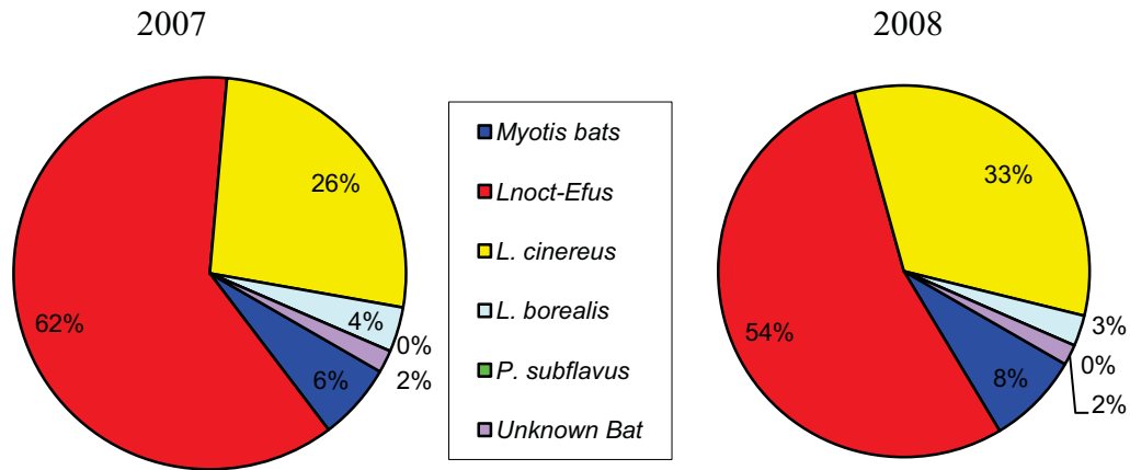
Figure 24. Distribution of Bat Activity by Species at the Cobb HIGH Microphone
