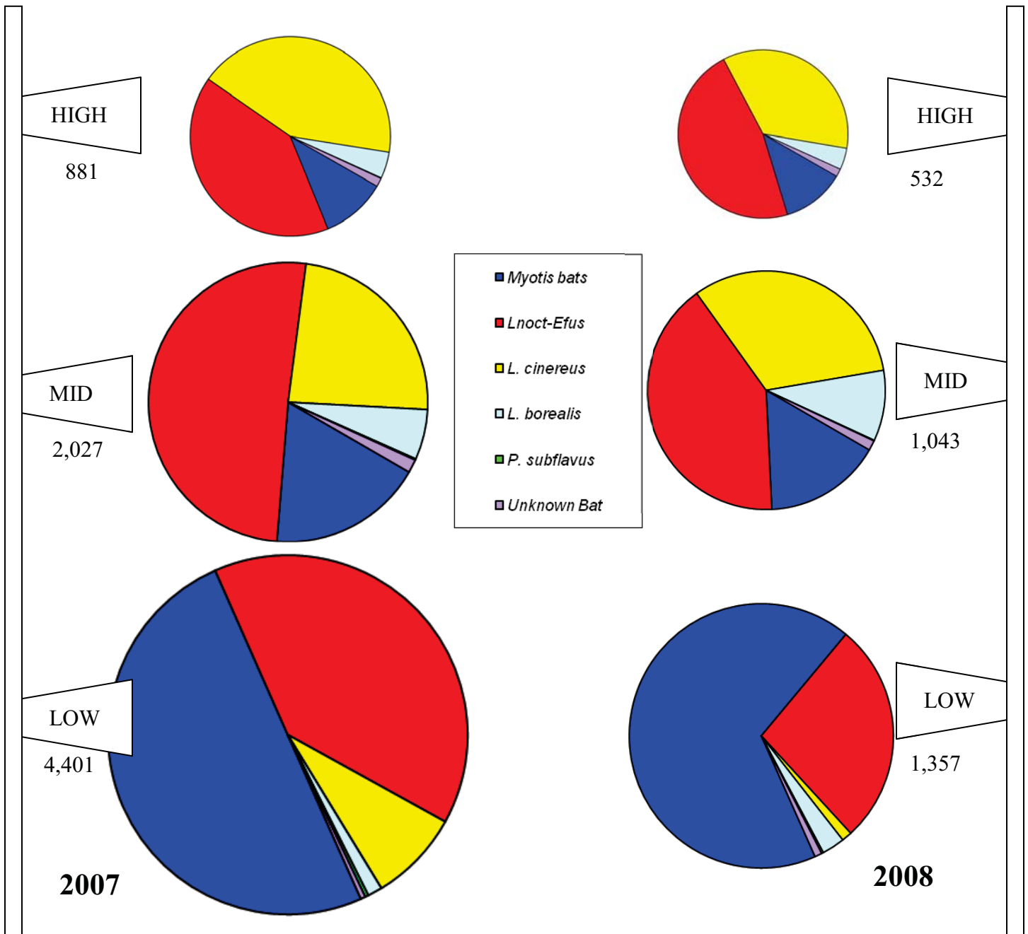
Figure 10. Distribution of Bat Activity across Microphone Heights at Flat Rock Site
