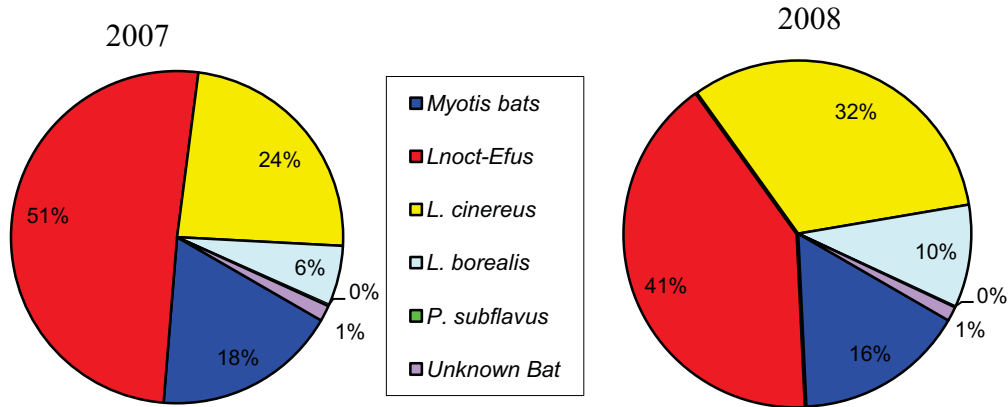
Figure 15. Distribution of Bat Activity by Species at the Flat Rock MID Microphone
