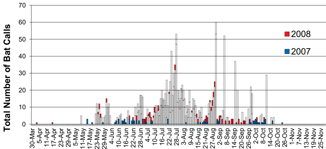
Figure 18. Temporal Distribution in Bat Activity at the Flat Rock HIGH Microphone
