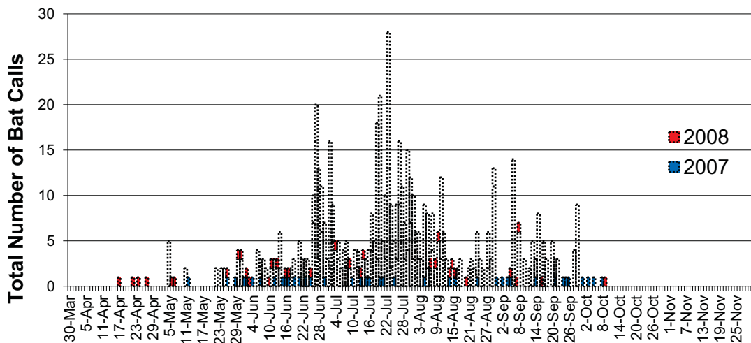
Figure 30. Temporal Distribution in Bat Activity at the Gardner MID Microphone
