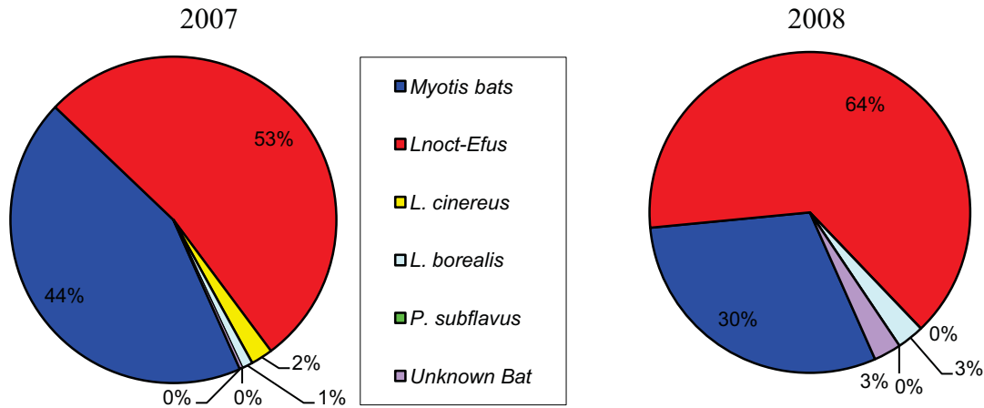
Figure 34. Distribution of Bat Activity by Species at the Porter LOW Microphone
