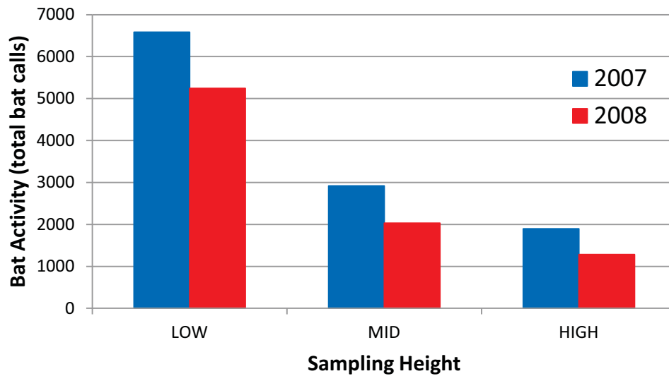
Figure 9. Spatial Variation in Bat Activity Relative to Sampling Height (all towers combined)
