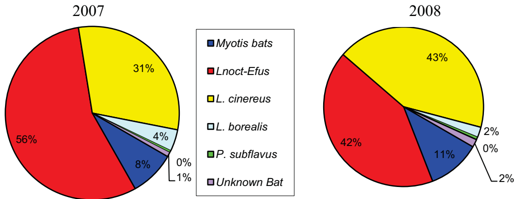
Figure 29. Distribution of Bat Activity by Species at the Gardner MID Microphone
