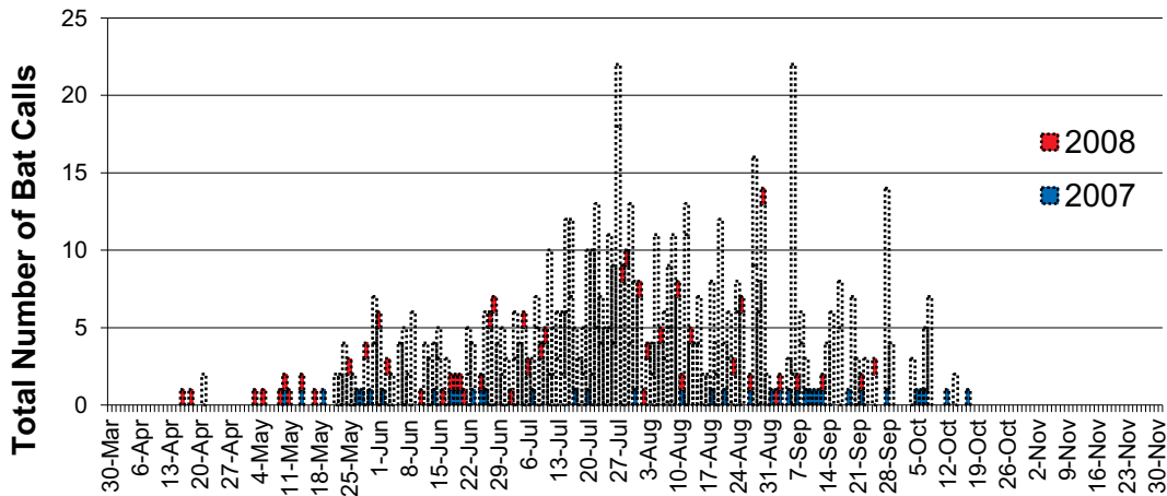
Figure 25. Temporal Distribution in Bat Activity at the Cobb HIGH Microphone (yellow bar represent high activity night where data bar was truncated to maintain overall pattern)
