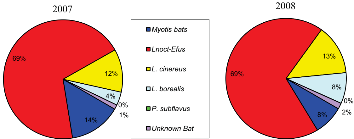
Figure 22. Distribution of Bat Activity by Species at the Cobb MID Microphone
