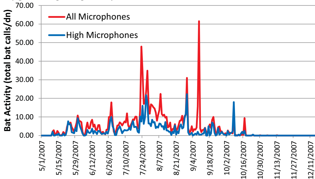
Figure 2. Seasonal Variation in Bat Activity Across the MRWP Site, 2007
