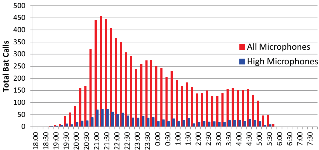
Figure 5. Temporal Variation in Bat Activity Across the MRWP Site, 2008
