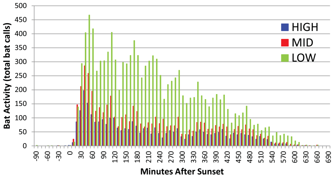
Figure 6. Temporal Variation in Bat Activity Relative to Sunset (both years combined)
