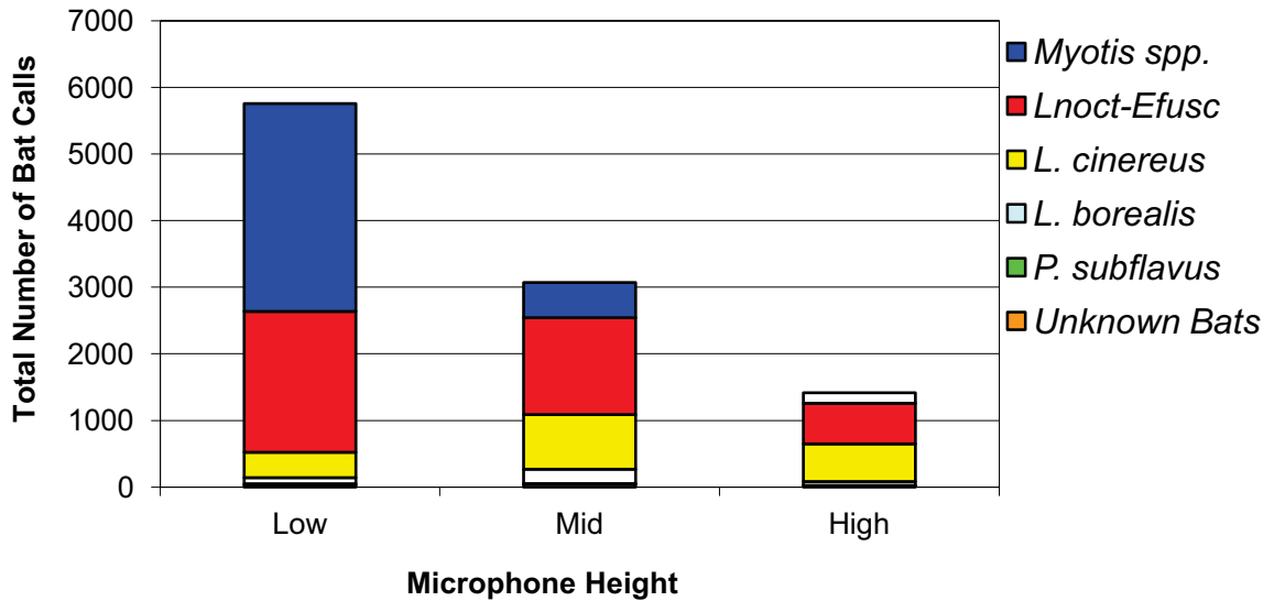
Figure 11. Distribution of Bat Activity At Flat Rock Site (2007 and 2008 combined)
