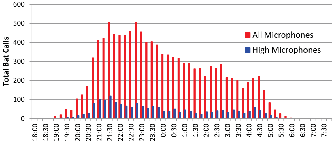
Figure 4. Temporal Variation in Bat Activity Across the MRWP Site, 2007
