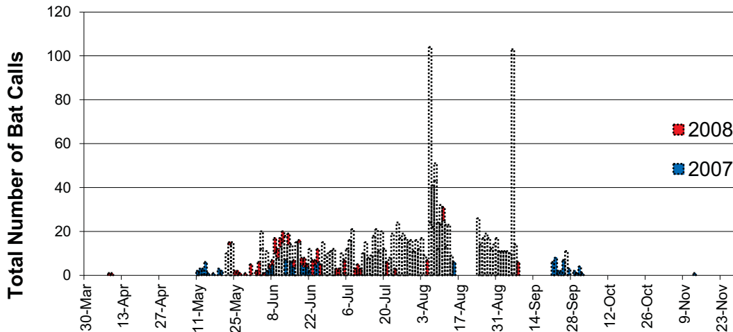
Figure 28. Temporal Distribution in Bat Activity at the Gardner LOW Microphone
