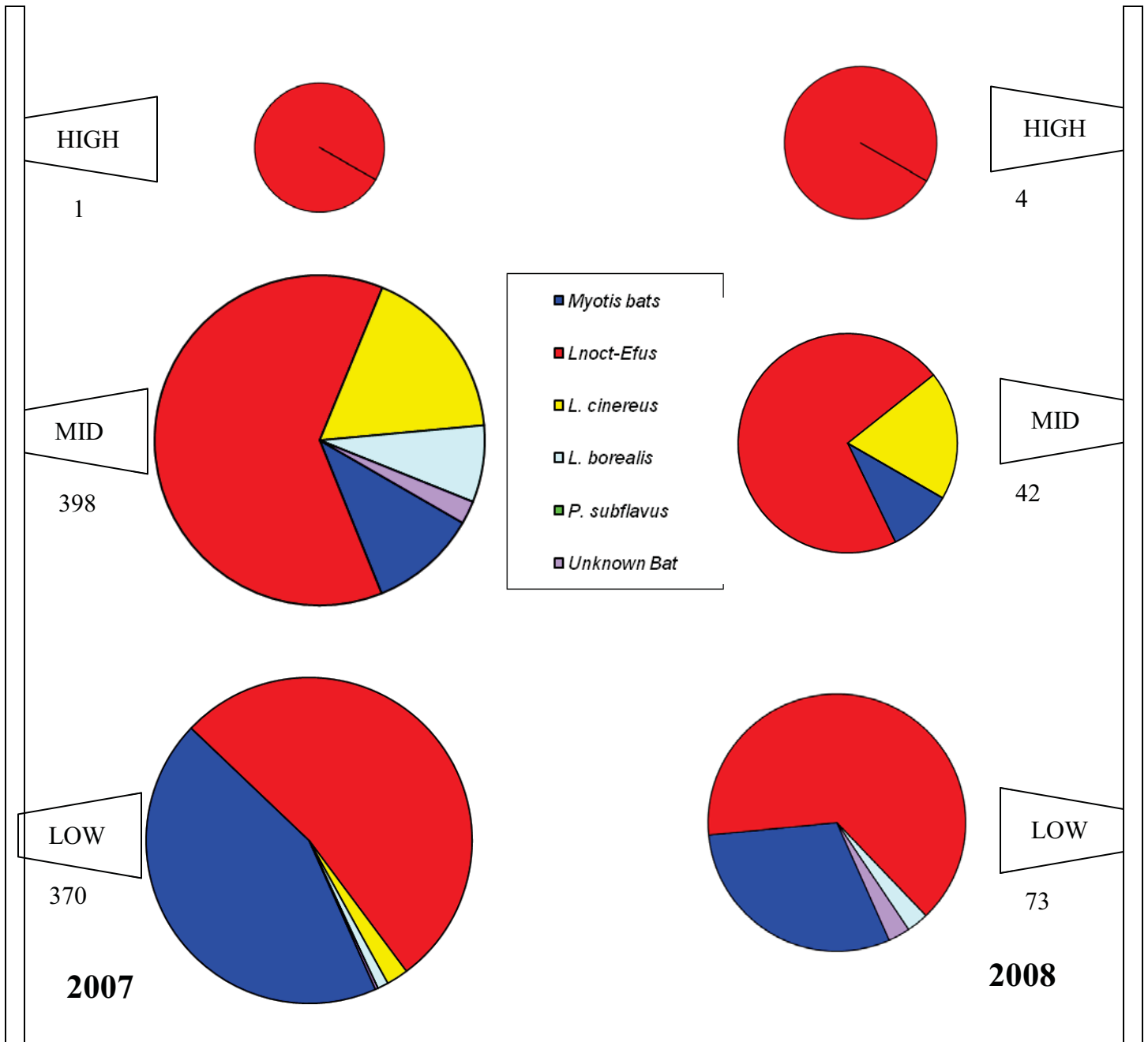
Figure 33. Distribution of Bat Activity across Microphone Heights at Porter Site
