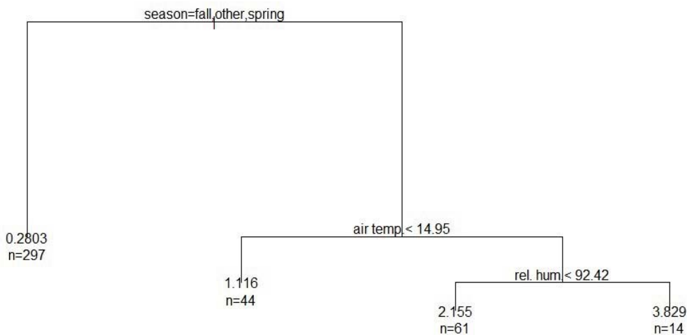
Figure 43. Regression tree for total nightly bat activity in the hoary bat ( L. cinereus ). The numbers at the terminal nodes represent mean nightly bat activity (n=number of nights).
