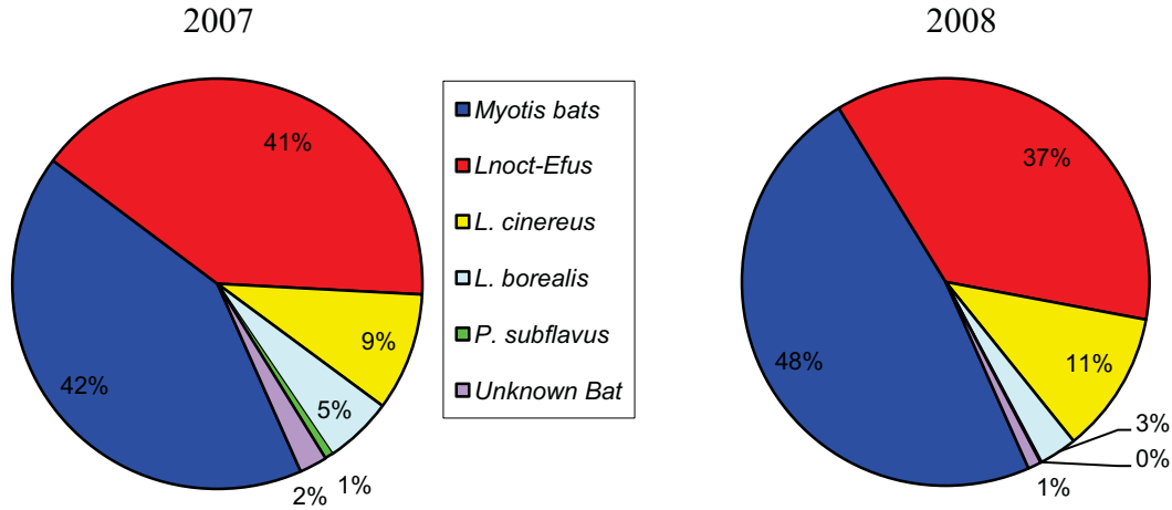
Figure 27. Distribution of Bat Activity by Species at the Gardner LOW Microphone
