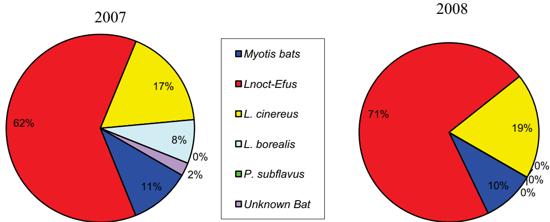
Figure 36. Distribution of Bat Activity by Species at the Porter MID Microphone
