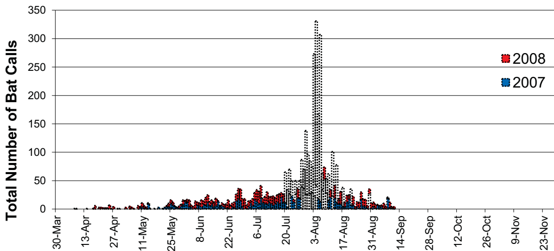
Figure 21. Temporal Distribution in Bat Activity at the Cobb LOW Microphone
