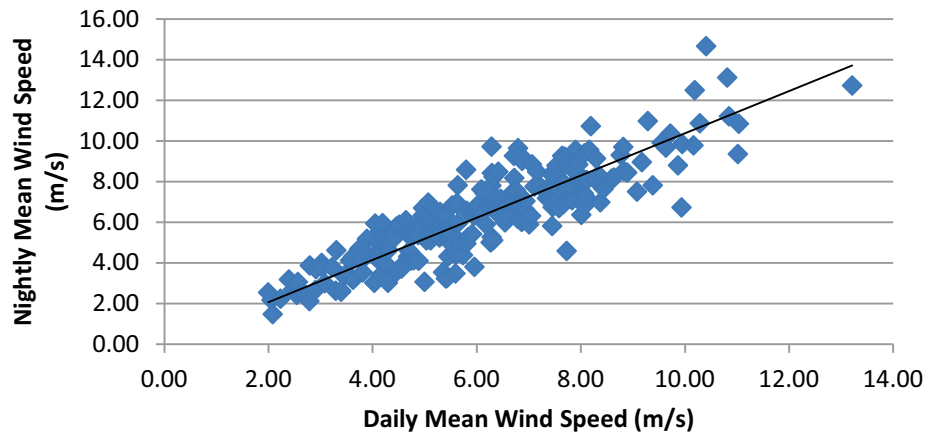
Figure 39. Correlation between Daily Wind Speed and Nightly Wind Speed
