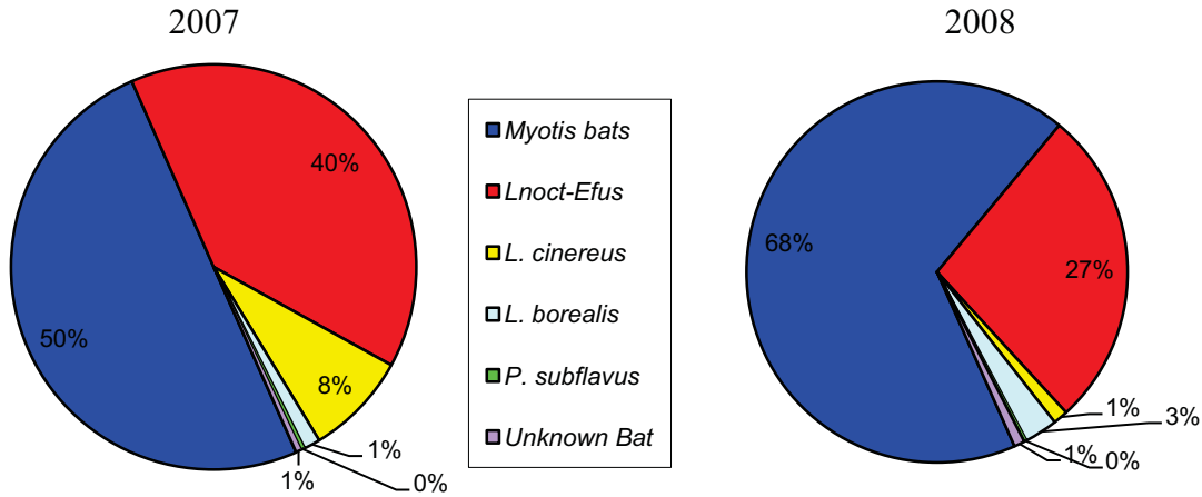
Figure 13. Distribution of Bat Activity by Species at the Flat Rock LOW Microphone
