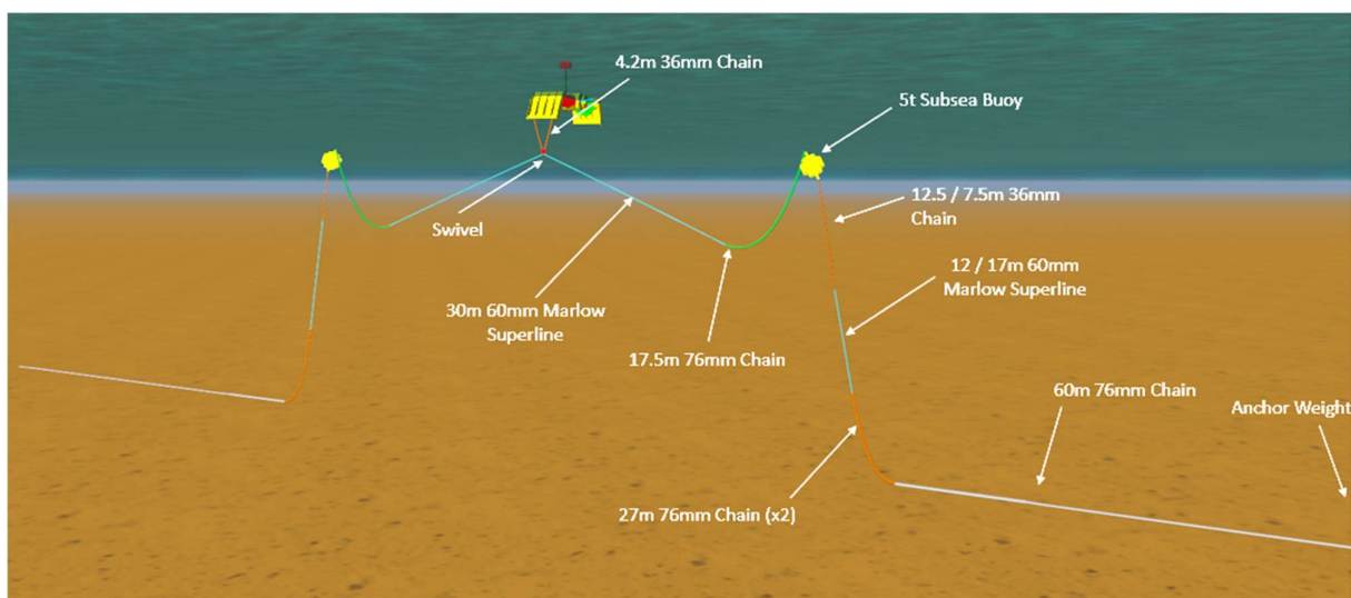
Figure 2-5 Mooring leg structure
