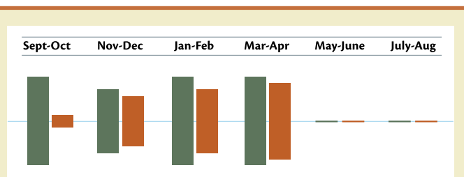
Figure 10: Temporal changes in relative abundance for Surf Scoters. This chart shows the year-round relative abundance of Surf Scoters observed by boat (■) and video aerial surveys (■) in two-month periods. Surf Scoters were most commonly observed in winter and none were observed in May-August.
