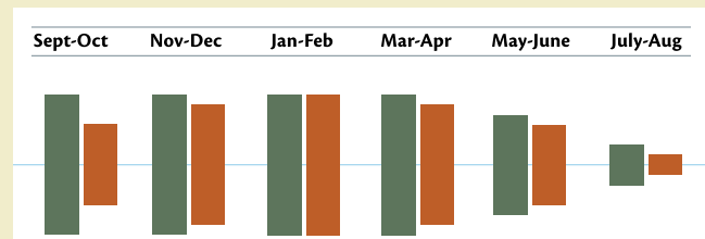
Figure 17: Temporal changes in relative abundance for Northern Gannets. This chart shows the year-round relative abundance of Northern Gannets observed by boat (■) and video aerial surveys (■) in two-month periods. Gannets were observed year-round, but were present in greatest numbers during winter.
