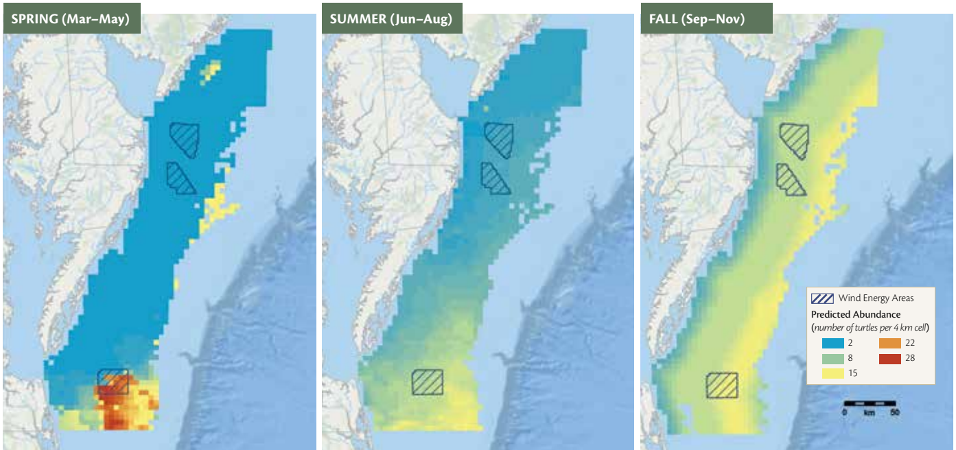
Figure 22: Predicted relative abundance of sea turtles by season, based on two years of digital video aerial survey data (2012–2014). Models used observation data from aerial surveys and remotely sensed environmental covariate data to predict abundance across the study area. Turtles had a dense southerly distribution in the spring, and were dispersed more broadly in the summer. By the fall, they were distributed fairly evenly across the mid-Atlantic in offshore areas.
