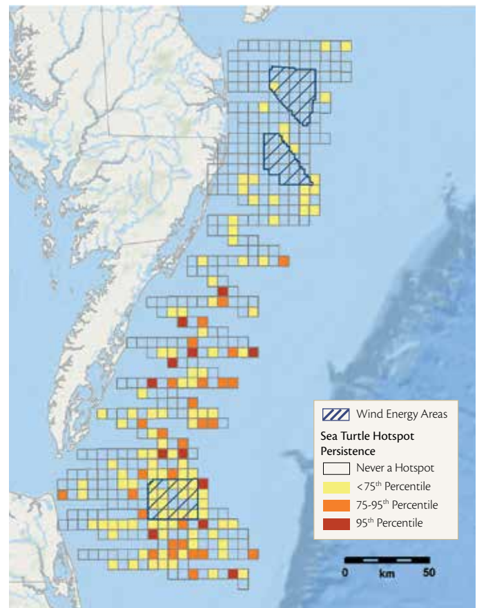
Figure 21: Persistent abundance hotspots for turtles ( Testudines spp.) observed in video aerial surveys, March 2012–May 2014. Data are split into only three persistence classes as the 75th and 85th percentile of persistence fell at the same value.
