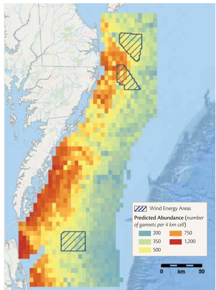
Figure 15: Predicted abundance of Northern Gannets for a given day in winter of 2013-14. This model used observation data from boat-based surveys and remotely sensed environmental covariate data to predict abundance across the study area. The highest abundance of Northern Gannets was predicted to occur closer to shore in regions with high primary productivity.
