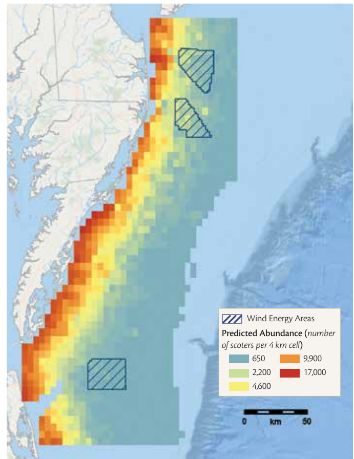
Figure 9: Predicted abundance of scoters (including White-winged Scoter, Black Scoter, and Surf Scoter) for a given day during winter of 2012-13. Model outputs combine observation data from boat-based surveys with environmental covariate data to predict scoter abundance across the study area. The highest abundance of scoters was predicted to occur close to shore and in regions with high primary productivity.
