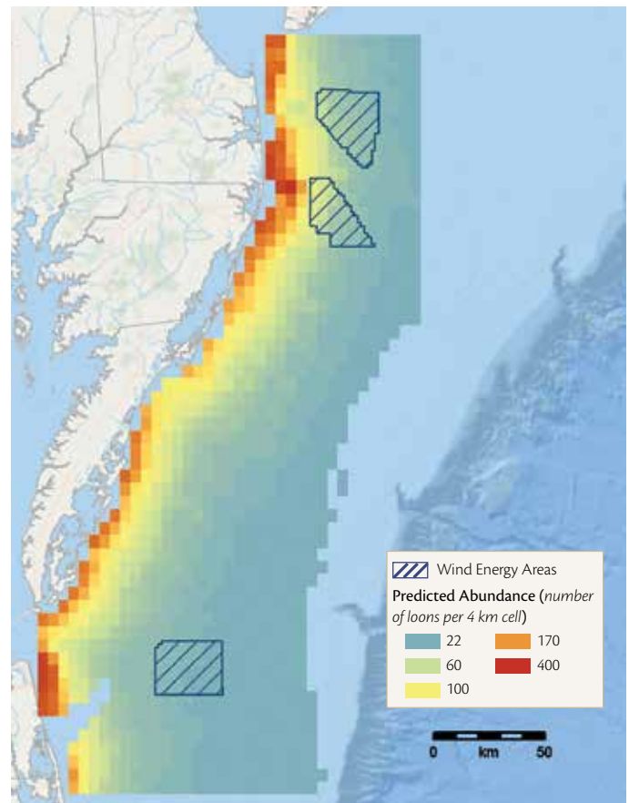
Figure 12: Predicted abundance of Red-throated Loons for a given day in winter of 2013-14 (Nov.-Jan.). Model outputs combine observation data from boat-based surveys with environmental covariate data to predict Red-throated Loon abundance across the study area. The highest abundance of Red-throated Loons was predicted to occur close to shore, and in regions with cooler water and high primary productivity.
