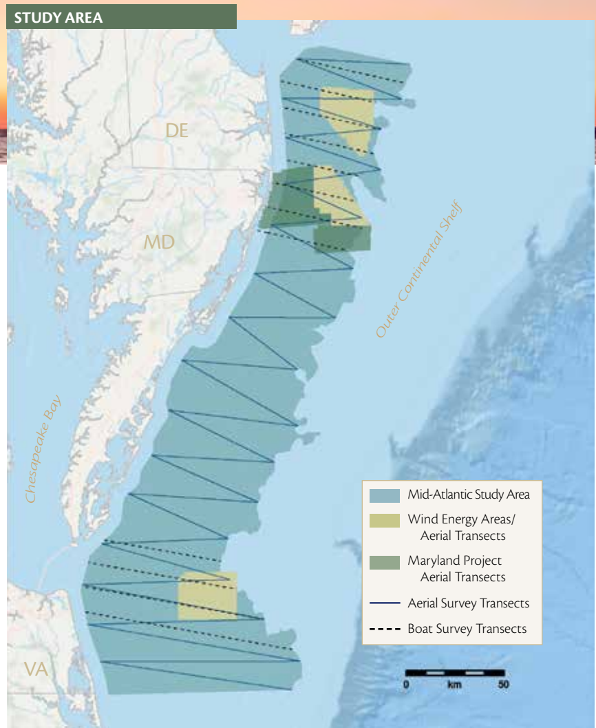
Figure 1: The study areas for the Mid-Atlantic Baseline Studies and Maryland projects, with WEAs and boat and aerial survey transects. Fine scale aerial transects (20% coverage) were carried out within the WEAs and the Maryland project area.
