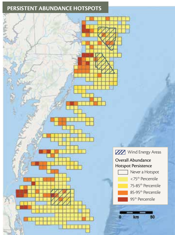
Figure 8: Persistent abundance hotspots—areas with consistently greater numbers of individuals across all taxa and surveys.
