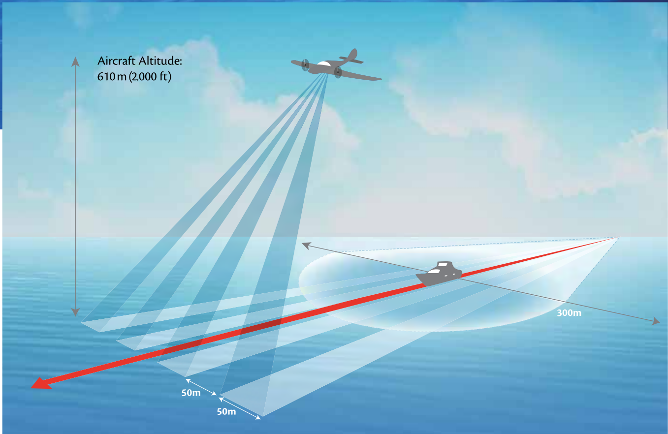
Figure 5: Boat–aerial survey comparison. The diagram shows the fields of view available during boat surveys and digital video aerial surveys. The combined strip width for all four video cameras was 200 m; the boat transect had an intended minimum strip width of 300 m, although observations of animals were made up to 1,000 m from the vessel. Apart from the experimental comparison (see below), boat and plane followed different transect lines (Figure 1).
