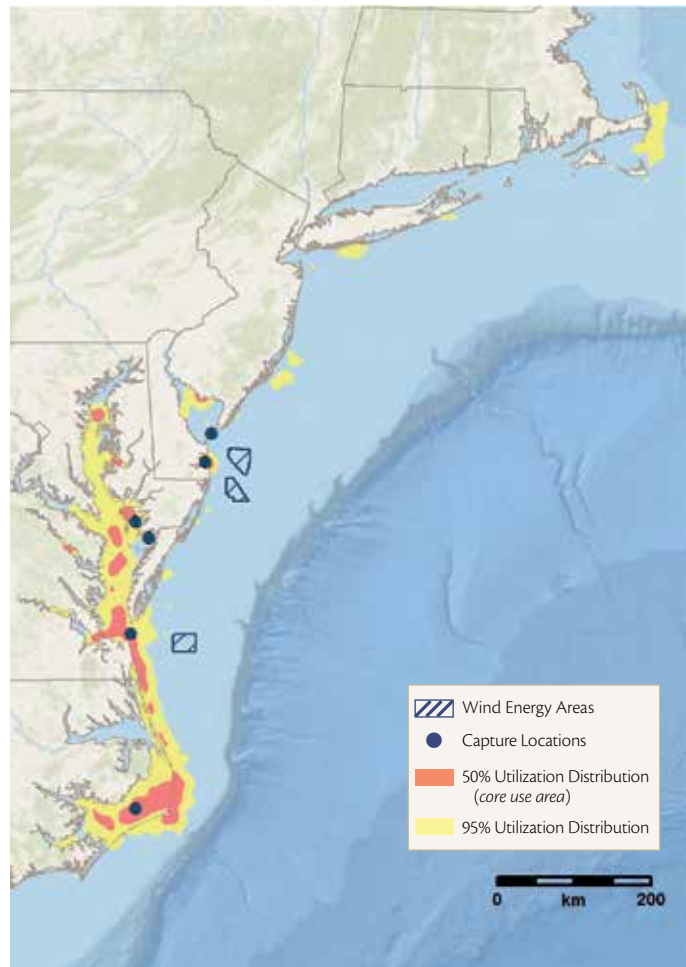
Figure 14: Winter utilization distribution for satellite-tagged Red-throated Loons (n=23; data are preliminary).
