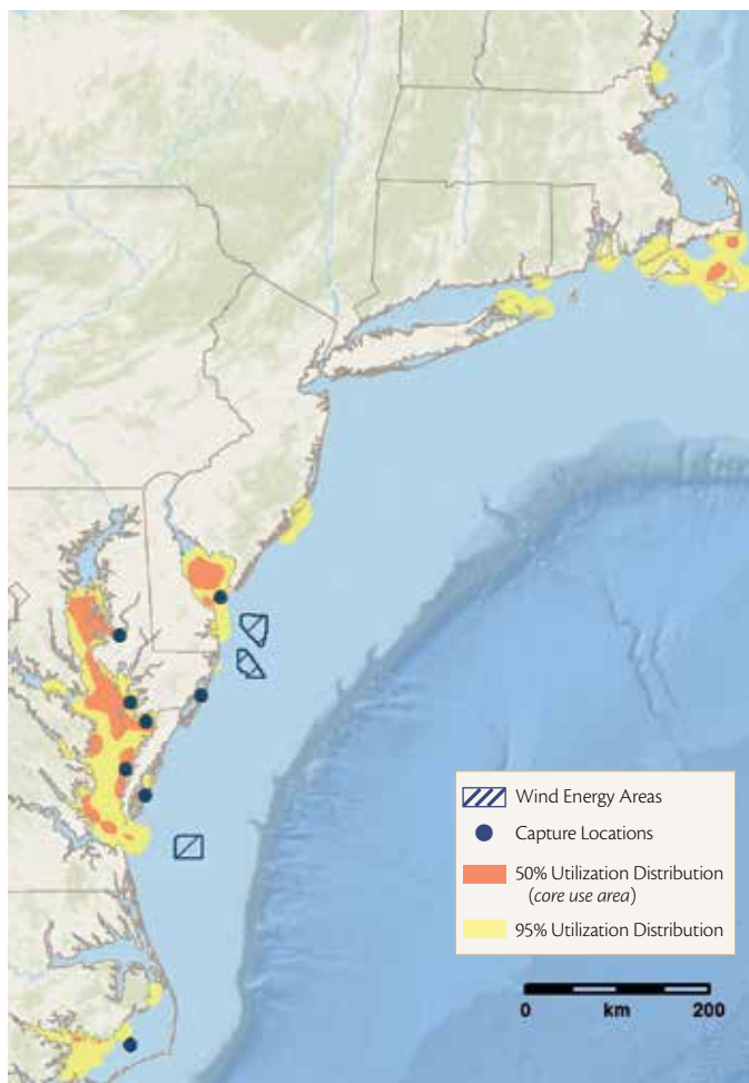
Figure 11: Winter utilization distribution for satellite-tagged Surf Scoters (n=101; data are preliminary). Additional capture locations in Labrador, Québec, and New Brunswick are not shown on this map.
