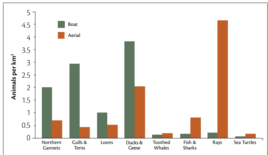
Figure 4: Comparison of total effort-corrected boat and aerial survey counts across all surveys for selected taxa. Aerial densities were calculated using actual transect strip widths, and boat densities were calculated using estimated strip widths for each taxon. Effective boat transect strip widths were calculated for avian taxa based on their effective half strip widths, and for aquatic taxa based on their median distance of observations from the boat. Observations of groups that were not individually counted or identified (e.g., some fish and ray schools) are excluded from this figure.
