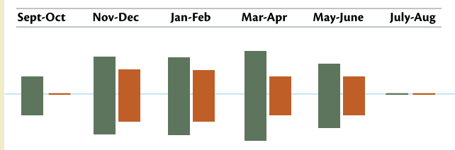
Figure 13: Temporal changes in relative abundance for Red-throated Loons. This chart shows the year-round relative abundance of Red-throated Loons observed by boat (■) and video aerial surveys (■) in two-month periods. Red-throated Loons were most commonly observed in winter. No individuals were observed in July-August by either survey method.
