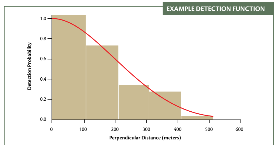
Figure 3: Detection function for Bottlenose Dolphins from boat surveys (in summer). A detection probability of 1.0 (y-axis) indicates the 100% probability of an observer spotting an animal that is present in the transect strip. The probability of detection decreases with distance of the animal from the observer (x-axis), with <10% probability of spotting a dolphin at 500 m. Actual survey data are summarized by tan bars; the distance curve, fitted to these data, indicates the estimated detection probability for an animal at a specified strip width.
