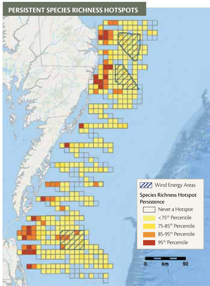
Figure 7: Persistent species richness hotspots—areas with consistently greater numbers of species across all surveys.
