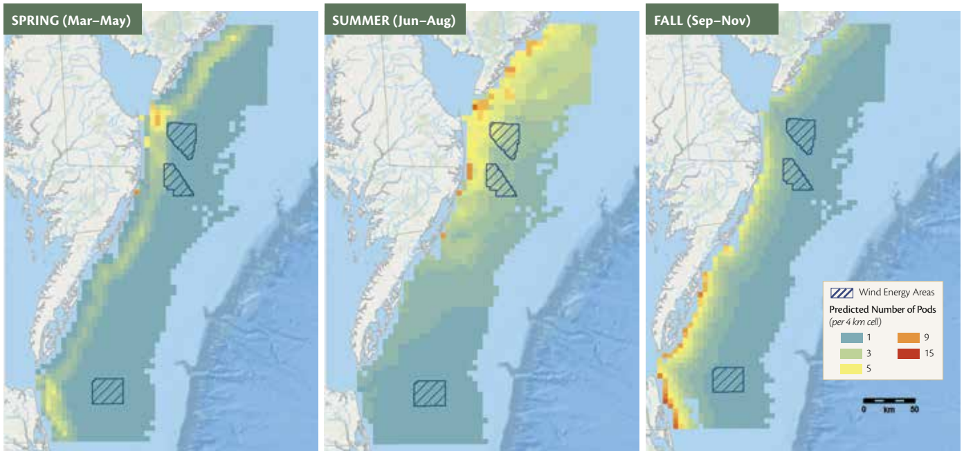
Figure 19: Predicted numbers of Bottlenose Dolphin pods by season, based on two years of boat survey data (2012-2014). Models used observation data from boat-based surveys and remotely sensed environmental covariate data to predict numbers of pods across the study area. Strong nearshore distributions were predicted in spring and fall, likely driven by the species' resident coastal ecotype. Dolphins were predicted to be more evenly distributed longitudinally in summer.
