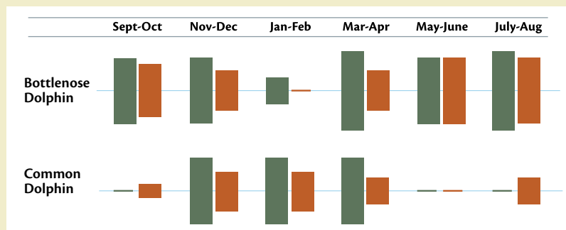
Figure 19: Predicted numbers of Bottlenose Dolphin pods by season, based on two years of boat survey data (2012-2014). Models used observation data from boat-based surveys and remotely sensed environmental covariate data to predict numbers of pods across the study area. Strong nearshore distributions were predicted in spring and fall, likely driven by the species' resident coastal ecotype. Dolphins were predicted to be more evenly distributed longitudinally in summer.
