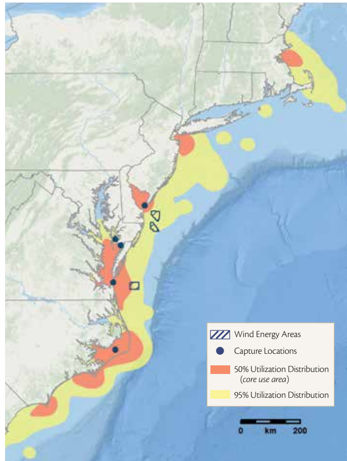
Figure 16: Winter utilization distribution of Northern Gannets tracked via satellite telemetry (n=17; data are preliminary).
