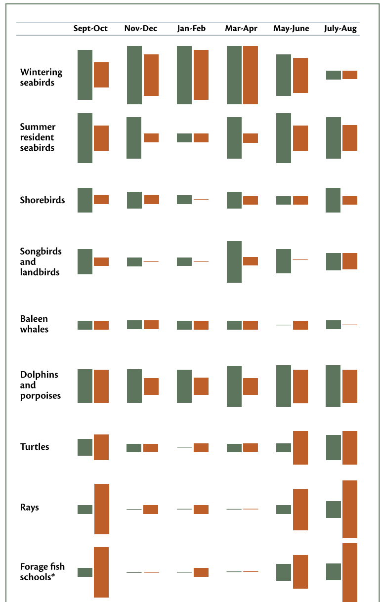
Figure 6: Temporal changes in relative abundance for major taxonomic groups. Data are from the boat-based surveys (■, left) and high resolution digital video aerial surveys (■, right) conducted in 2012-2014. Species included in each category are listed in Williams et al. (2015). Labels refer to seasons in the Northern Hemisphere.
