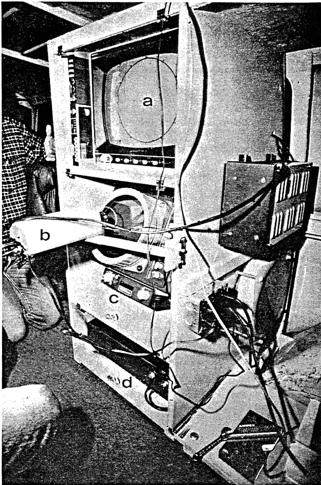
Figure 6. Interior of utility van showing monitoring equipment: a) video monitor, b) TV camera, c) radar (PPI) screen, d) video recorder.
