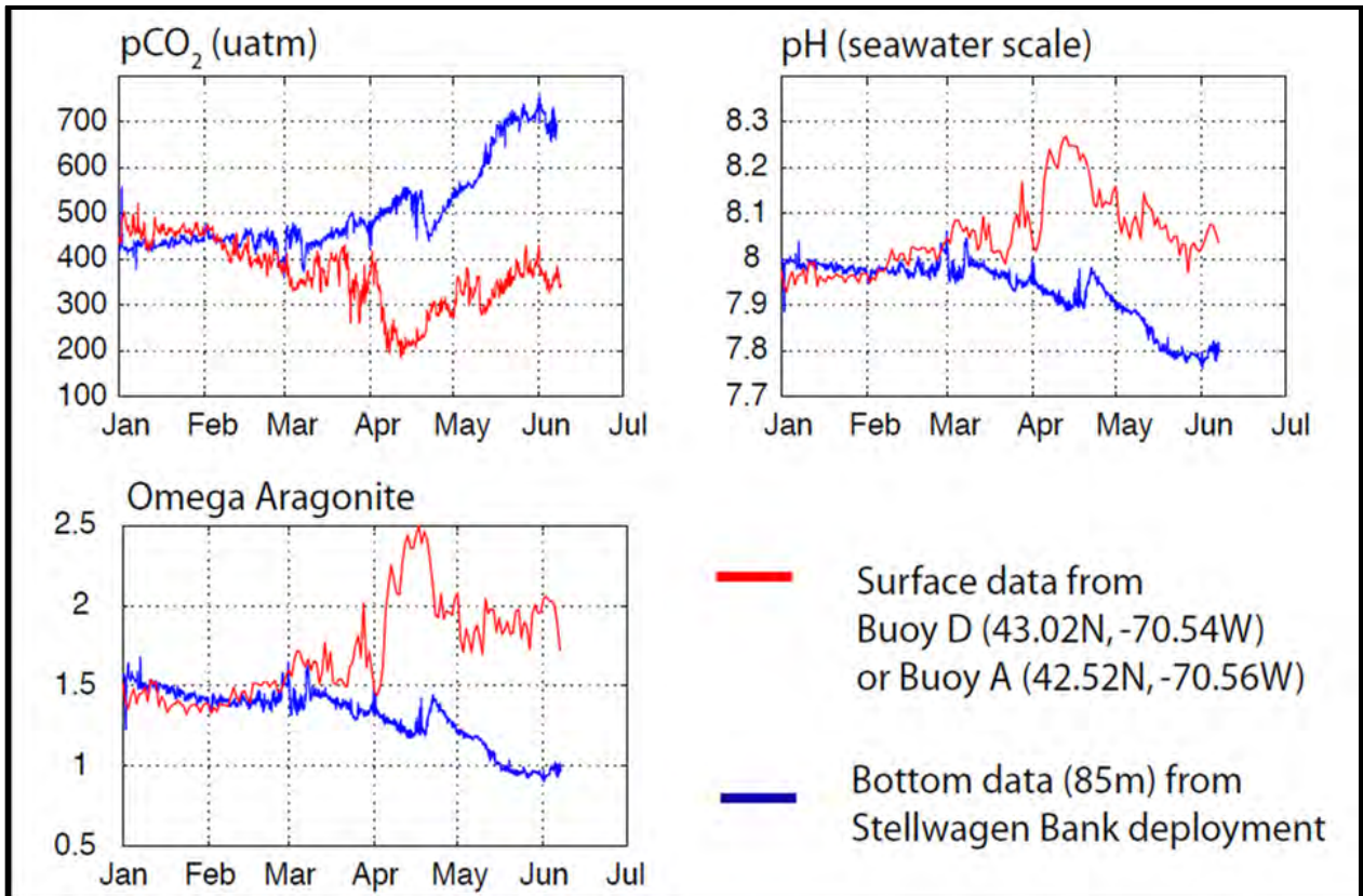
Figure 3. The partial pressure of CO 2 (microatmospheres), pH, and derived aragonite saturation (omega) at the surface (-2 m, red) and bottom (-85 m, blue) of the western Atlantic ocean. The surface measurements were recorded at the University of New Hampshire (UNH) buoy near Appledore Island. 71 The bottom measurements were recorded by Stellwagen Bank National Marine Sanctuary on a buoy in Massachusetts Bay. Figure courtesy of Joe Salisbury, University of New Hampshire.
