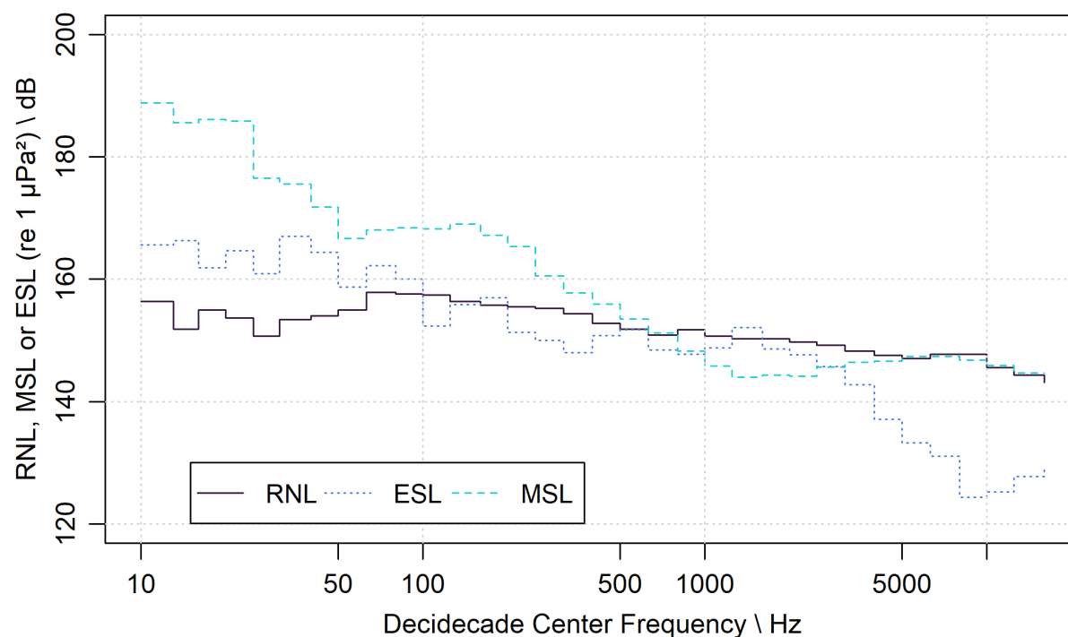
Figure D-11. Comparison of the three methods used to compute the sound levels emitted by the ferry Margaret's Justice .
