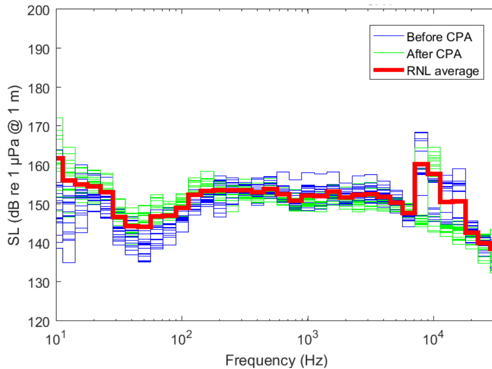
Figure D-15. Decade radiated noise level calculated for the pass of the ferry Margaret's Justice that was recorded on 16 Oct 2018 at 14:30. The broadband radiated noise level (RNL) for this measurement is 167.5 dB re 1 \mu Pa m (1 Hz to 32 kHz); the calculation (average RNL, red solid line) is influenced by the energy introduced by the projector sound emissions, as visible from the peaks that are present around 10 kHz. Furthermore, the low end of the spectrum below 300 Hz is elevated by the ambient noise.
