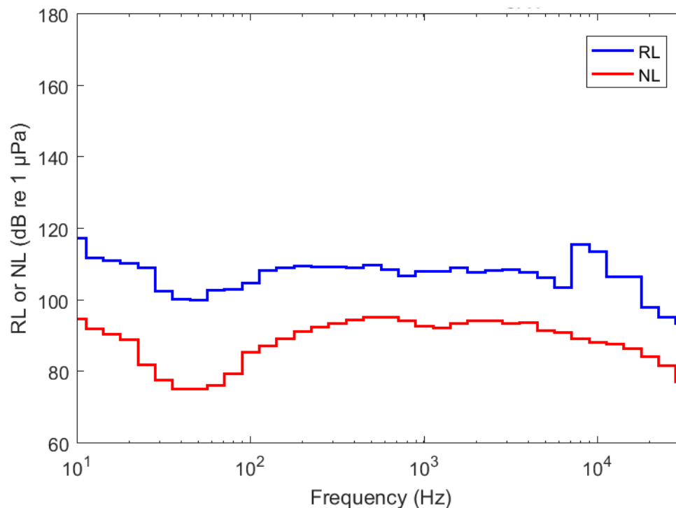
Figure D-16. Decade received level calculated for the pass of the ferry Margaret's Justice that was recorded on 16 Oct 2018 at 14:30 and ambient noise level average.
