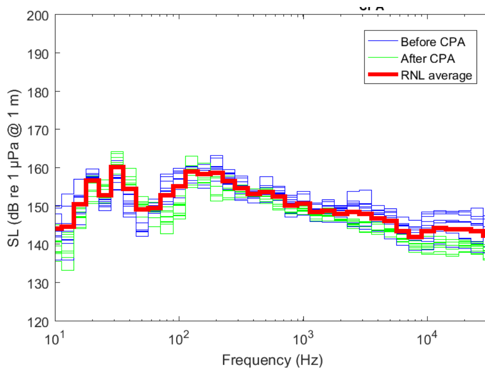
Figure D-3. Decade radiated source level calculated for the pass of the ferry Margaret's Justice that was recorded on 4 Oct 2018 at 01:05 am. The broadband Radiated noise level (RNL) for this measurement is 168.5 dB re 1 \mu Pa m (1 Hz to 32 kHz).
