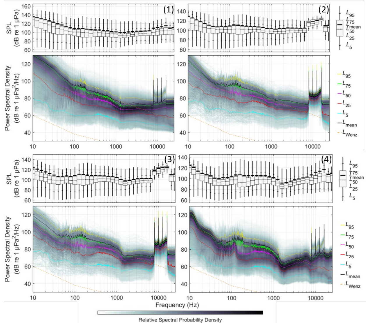
Figure B-16. AMAR A, channel 1 (top left), channel 2 (top right), channel 3 (bottom left) and channel 4 (bottom right): Exceedance percentiles and mean of 1/3-octave-band SPL and exceedance percentiles and probability density (grayscale) of 1-min power spectral density levels compared to the limits of prevailing noise (Wenz 1962).
