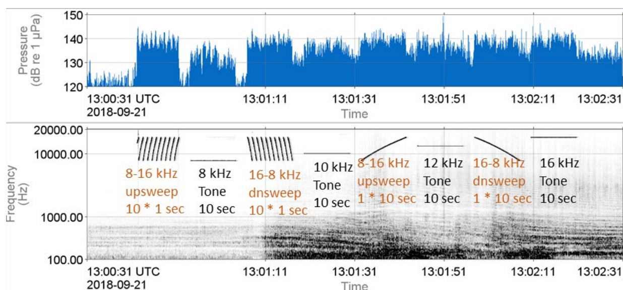
Figure A-5. Two-minute (top) time series and (bottom) spectrogram showing the sounds emitted by the experimental source in Grand Passage on 21 Sep 2018. The types of signals are described in Table A-4.
