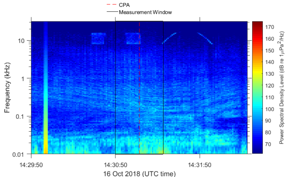
Figure D-14. Spectrogram of the measurement for one of the rejected ferry passes. The measurement window and closest point of approach (CPA) are highlighted in the spectrogram. The sounds emitted by the projector are visible between 10–20 kHz, as well as low frequency noise below 30 Hz.
