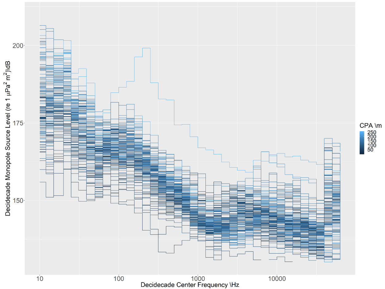
Figure D-7. Monopole Source Level for the ferry Margaret's Justice computed using the propagation loss shown in Figure D-1. The colour of each line indicates the distance to the closest point of approach distance.
