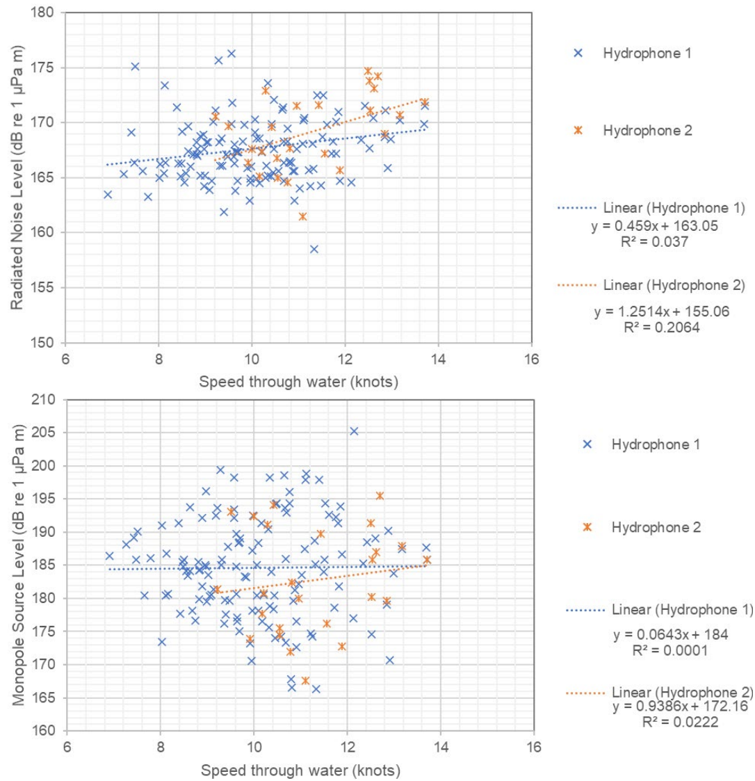
Figure D-9. Scatter plots of Radiated Noise Level (RNL, top) and Monopole source level (MSL, bottom) versus speed through water for the ferry Margaret's Justice Ferry calculated from measurements at hydrophone 1 (blue) and hydrophone 2 (orange) of AMAR B. The dotted lines represent the linear fit trends for each data set. Linear regression lines and r-squared values are also displayed for each data series.
