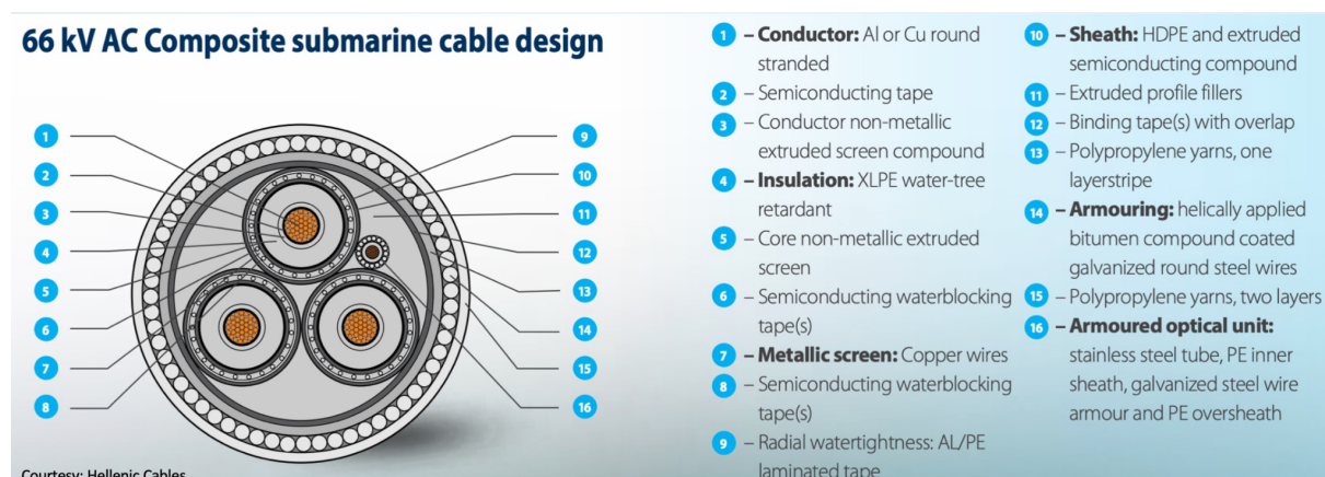
Figure 9. Composite subsea cable design. Dynamic inter-array cables require two layers of armoring for additional fatigue resistance (instead of a single layer for static cables). Source: Hellenic Cables.
