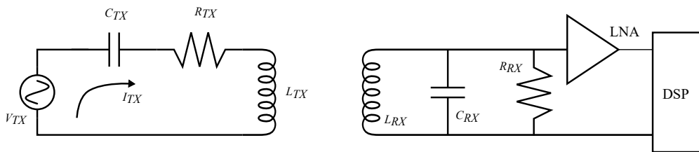
Fig. 3.7: Model of the system front-end
