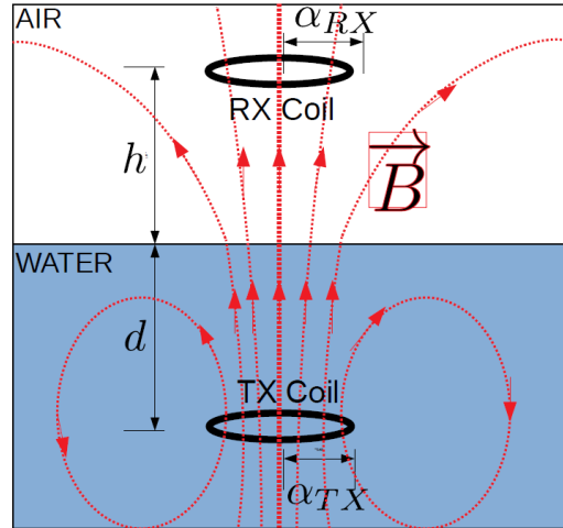
Fig. 3.3: Representation of the Magnetic Fields
