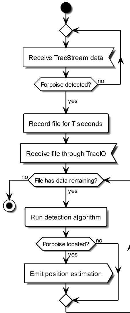
Fig. 2.7.3: Activity diagram on the Zybo board
