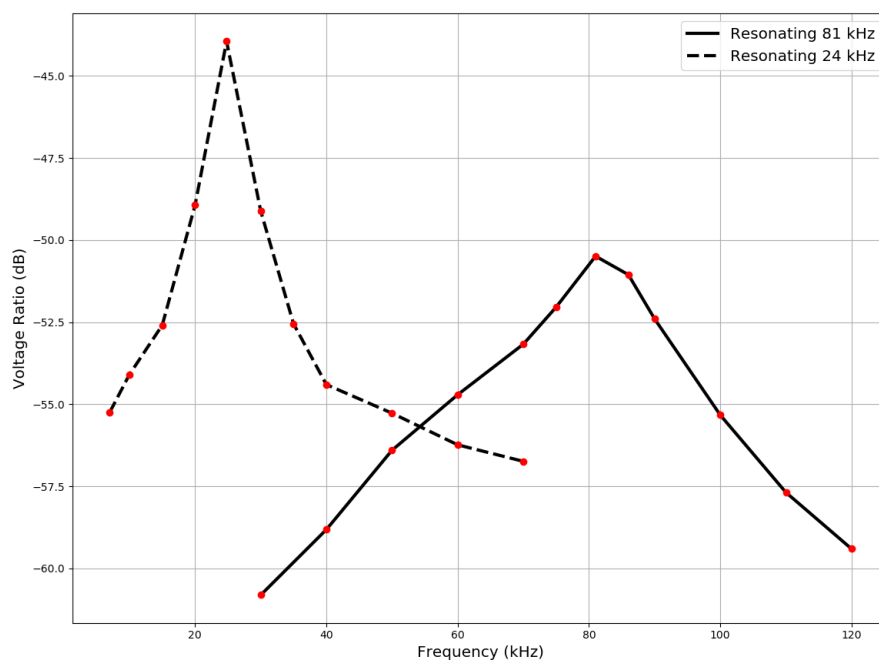
Fig. 3.17: Measured voltage ratio for a TX depth of 2 ft and at two resonating frequencies: At 24 kHz and at 81 kHz.
