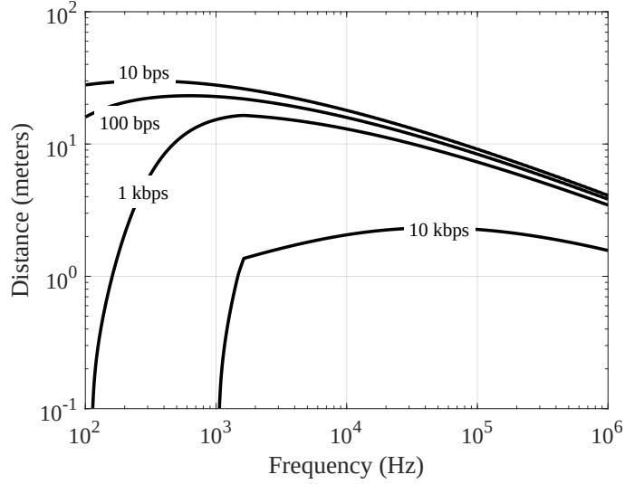
Fig. 3.5: Capacity of the magneto-inductive link
