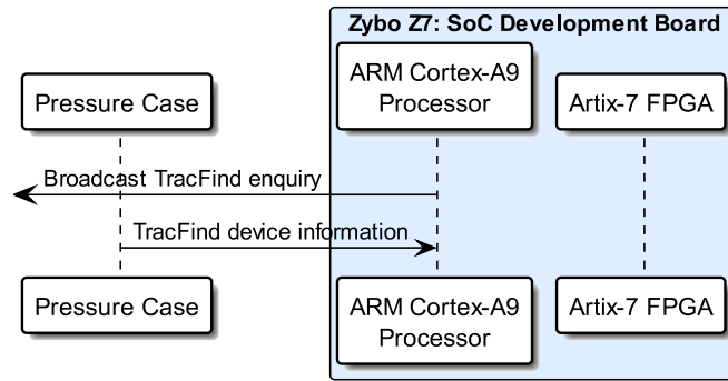
Fig. 2.7.4: TracFind program sequence diagram
