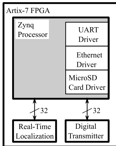
Fig. 2.7.1: Firmware architecture for the real-time remote sensor
