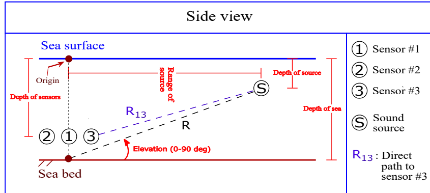
Fig. 2.2.2: Side view of a planar hydrophone array that is mounted horizontally.
