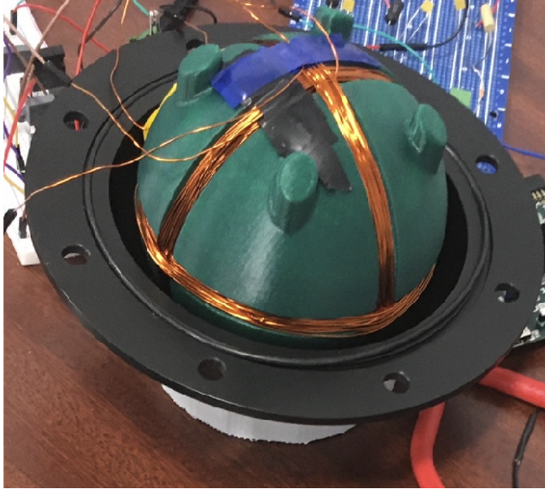
Fig. 3.8: Image of the interior of the transmitter
