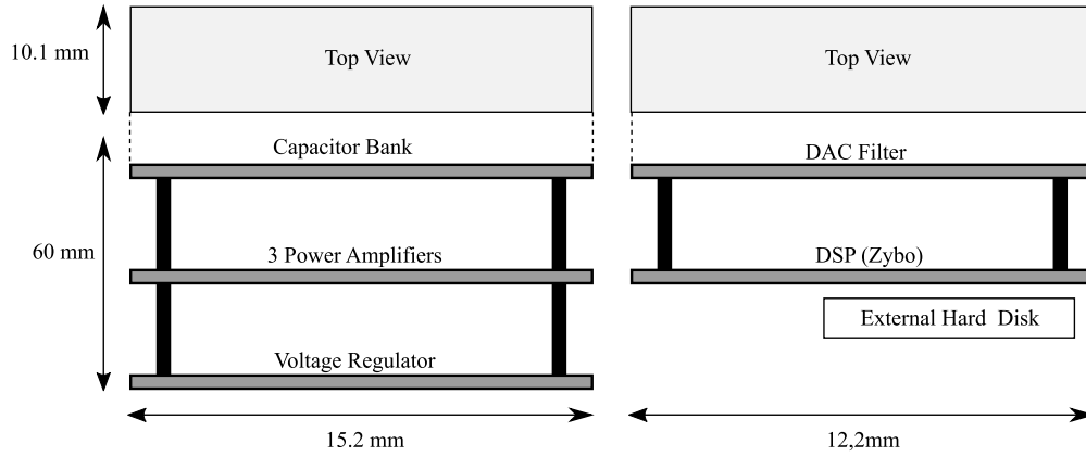
Fig. 3.9: Transmitter Electronic Board Design
