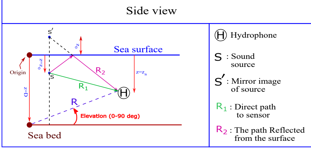
Fig. 2.2.4: Representation of the Lloyd-mirror model.
