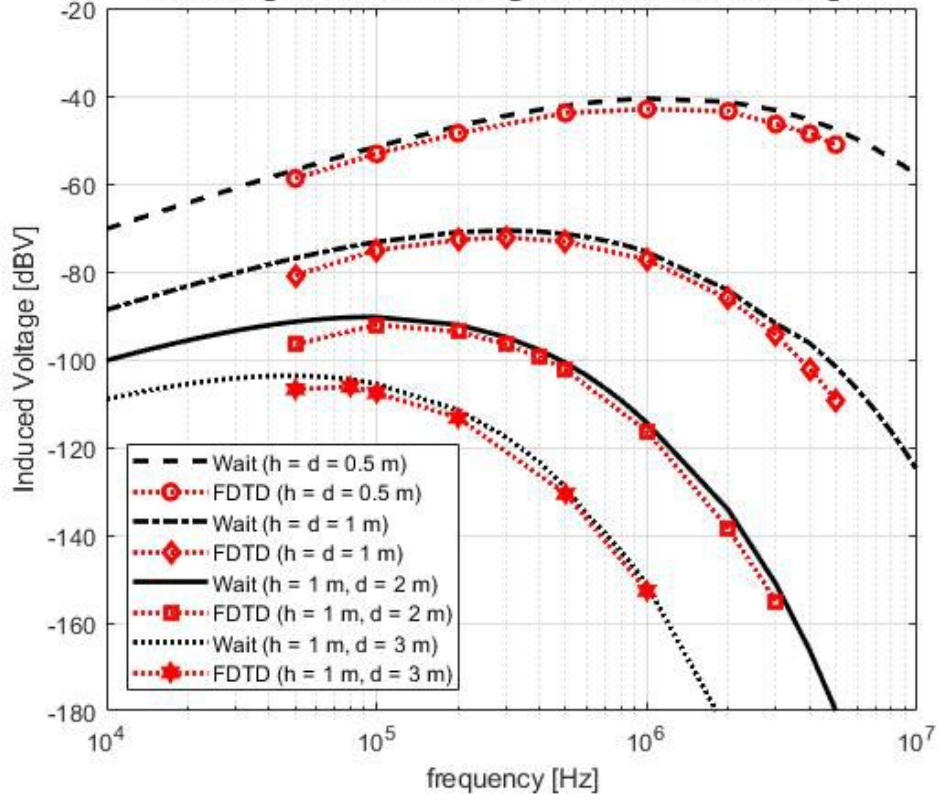
Fig. 3.4: Comparing the Predictions of the Induced Voltage in Receiver Coil Using Wait's Analytical Model and the FDTD Simulations as a Function of Frequency, Transmitter Depths ( d ), and Receiver Heights ( h ).
