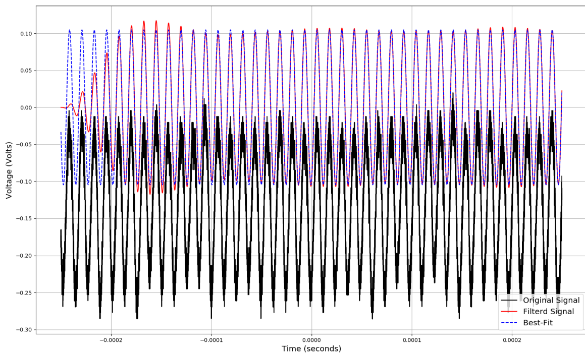
Fig. 3.16: Sample illustration of how the signal is passed through a bandpass filter and then a least-squares fit is applied.
