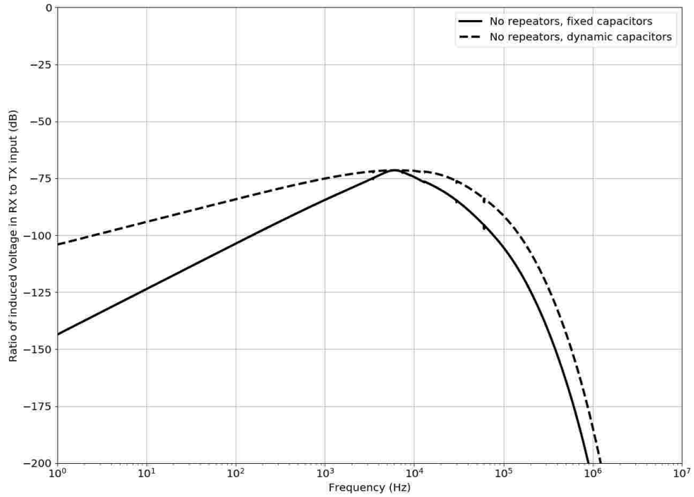
Fig. 3.6: Sample frequency response plot for a node 10 meters below the sea surface
