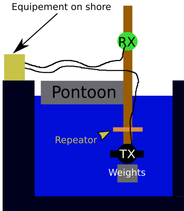
Fig. 3.12: Schematic of the Coils Setup in the Aquatron.
