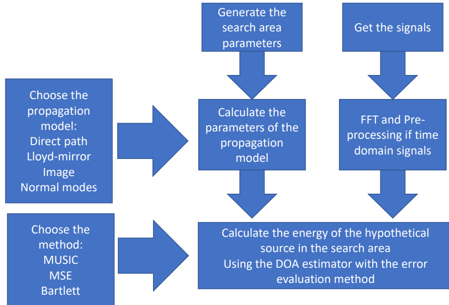
Fig. 1.1: General Structure for the Localization Algorithm.
