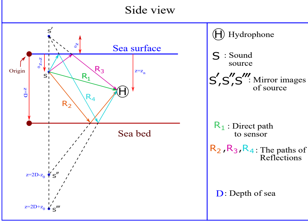
Fig. 2.2.5: Schematic of the Image model.
