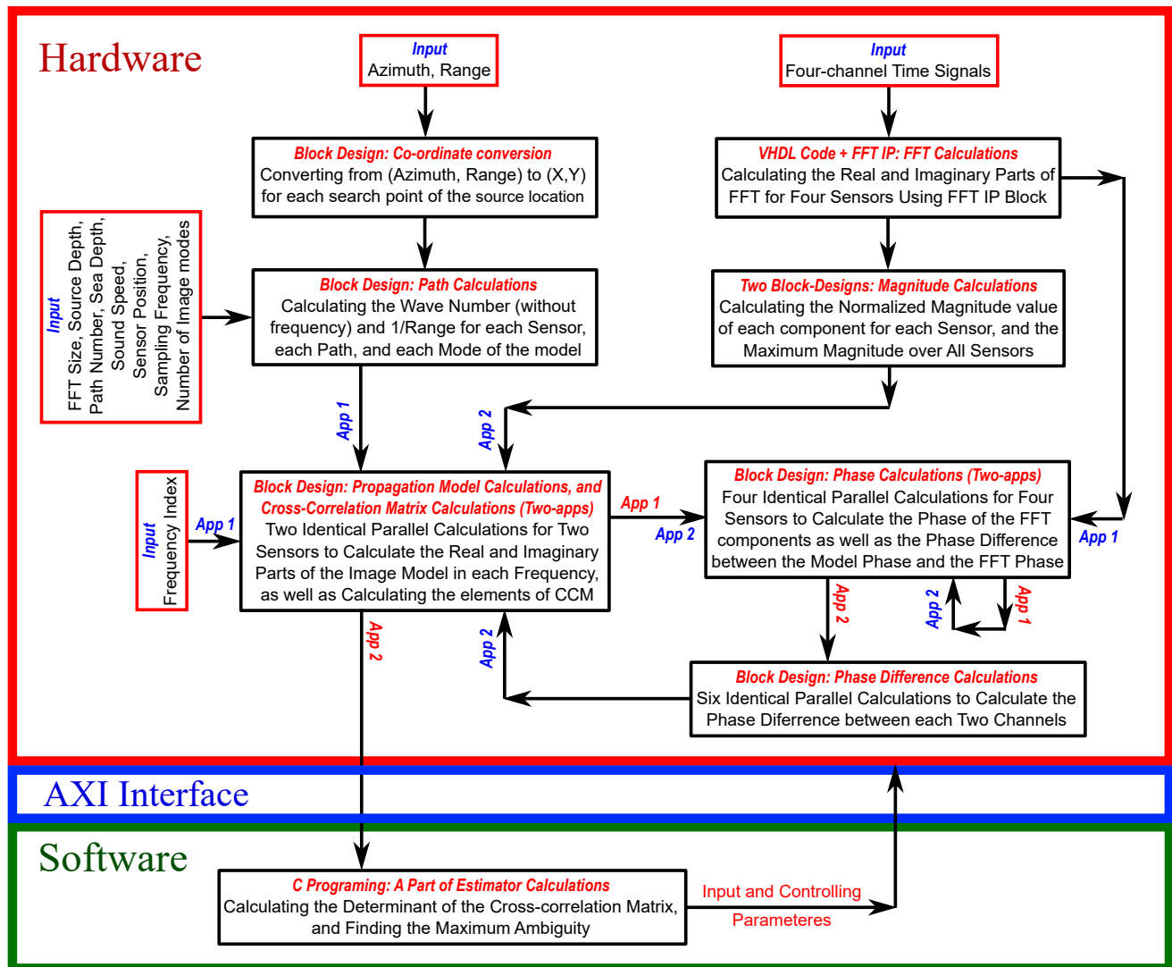
Fig. 2.7.7: An overview of the block separation
