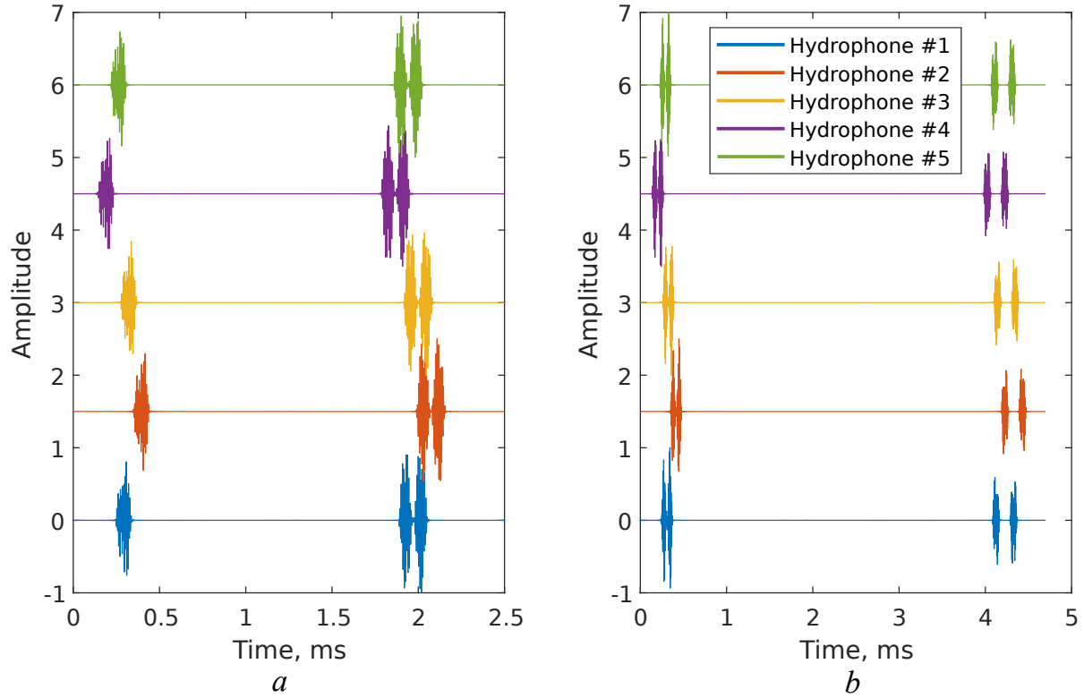
Fig. 2.6.14: Synthetic signals of the hydrophones in the time-domain.
