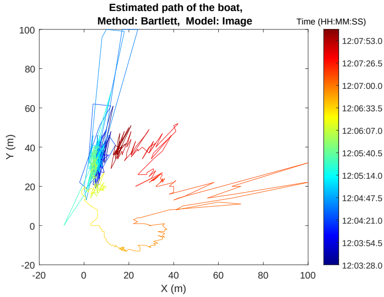
Fig. 2.6.9: The complete path of the maximum energy for the propeller noise of the boat.
