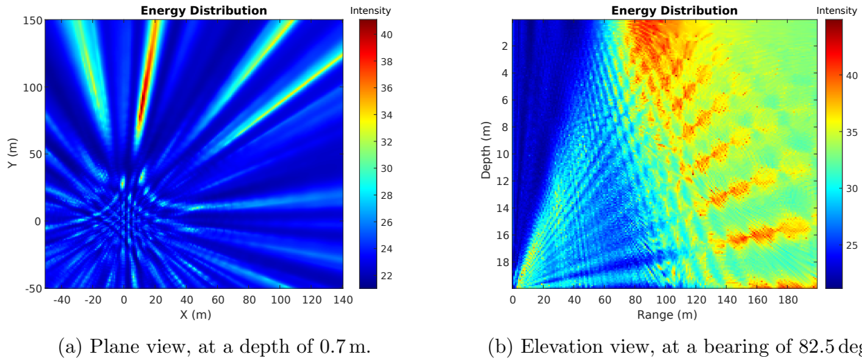
Fig. 2.6.8: 3D Localization of the sonar pulse using ambiguity function. Regions of high intensity represent potential location of the target.
