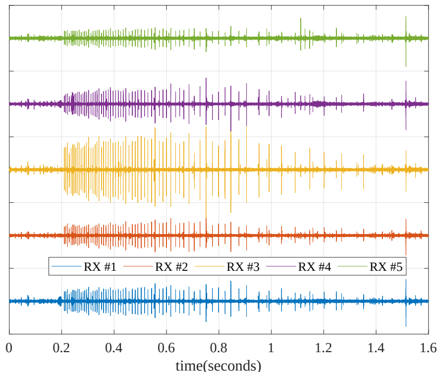
Fig. 2.6.5: In the window between 0.2 and 0.8 seconds, 53 clicks are emitted, with an average click interval of 11 msecs. Clicks last on the order of 0.1 msecs.
