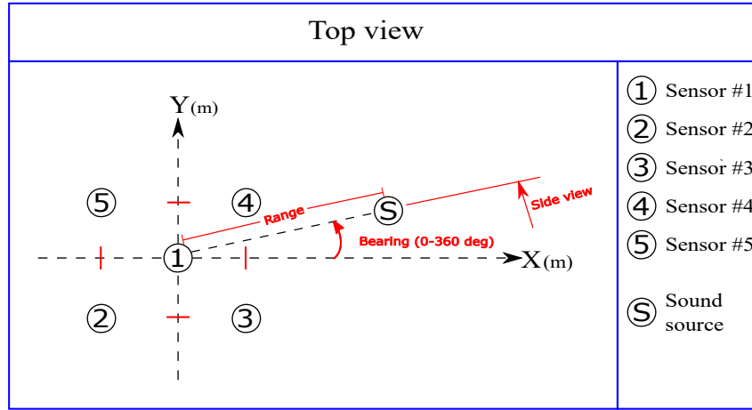
Fig. 2.2.1: Top view of a planar hydrophone array that is mounted horizontally.
