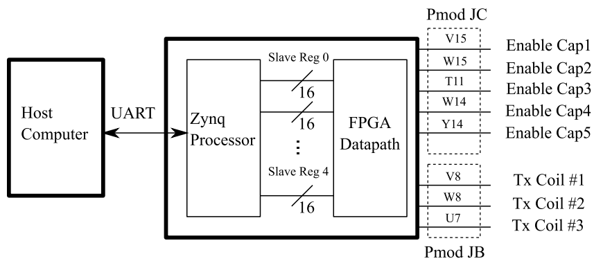
Fig. 3.10: Transmitter Firmware Interface to Generate Transmit Signals
