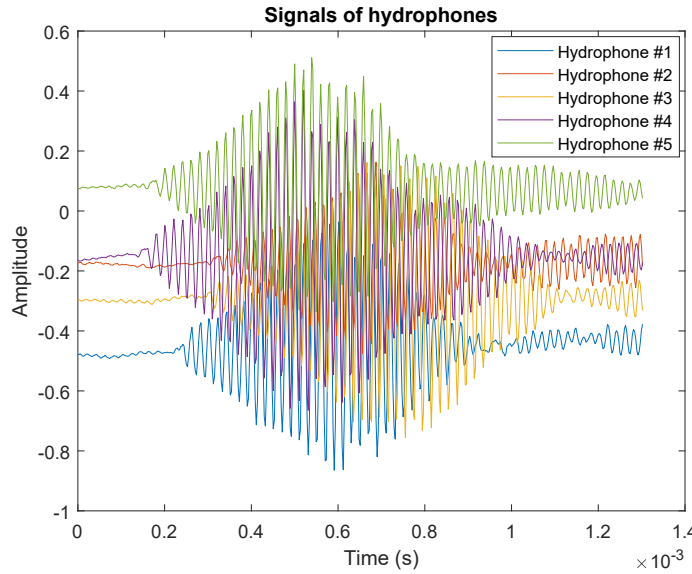
Fig. 2.6.7: Received signals of a sonar at the five hydrophones.
