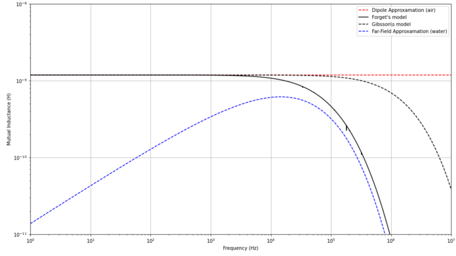
Fig. 3.2: Plots comparing Forget's model (64) to Gibson's (65) with h = 1 m, d = 19 m.
