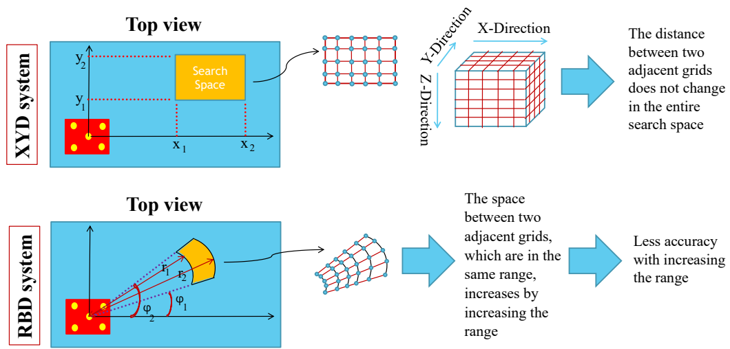
Fig. 2.2.3: The Search Space in the XYD and RBD Coordinate Systems.
