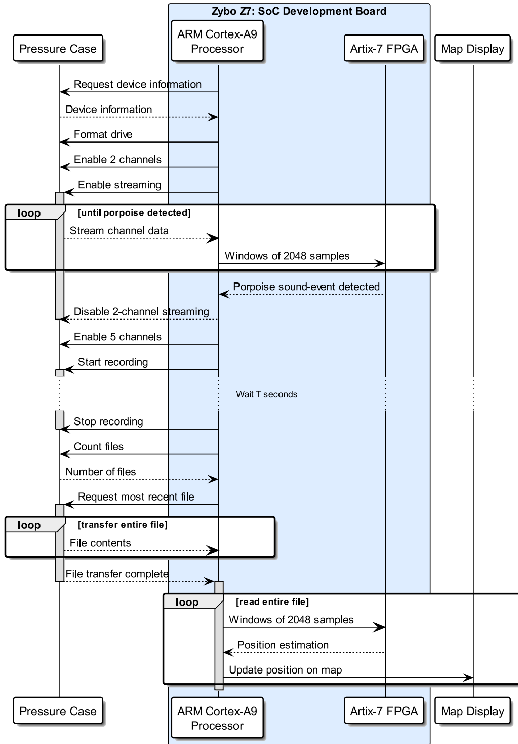
Fig. 2.7.5: Trac program sequence diagram
