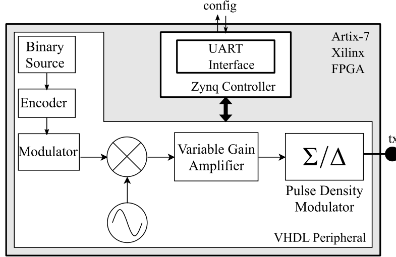
Fig. 2.7.6: Transmitter system architecture
