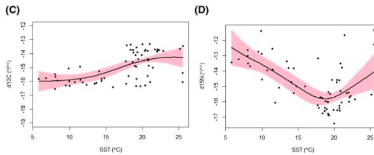
Figure 3.12 Generalised additive model (GAM) results showing significant non-linear relationships between (C), \delta^{13}\text{C} and sea surface temperature (SST) °C; (D), \delta^{15}\text{N} and SST. The solid line is the model estimated mean, and the pink polygon represents the model standard error (Atkins et al. 2023).
