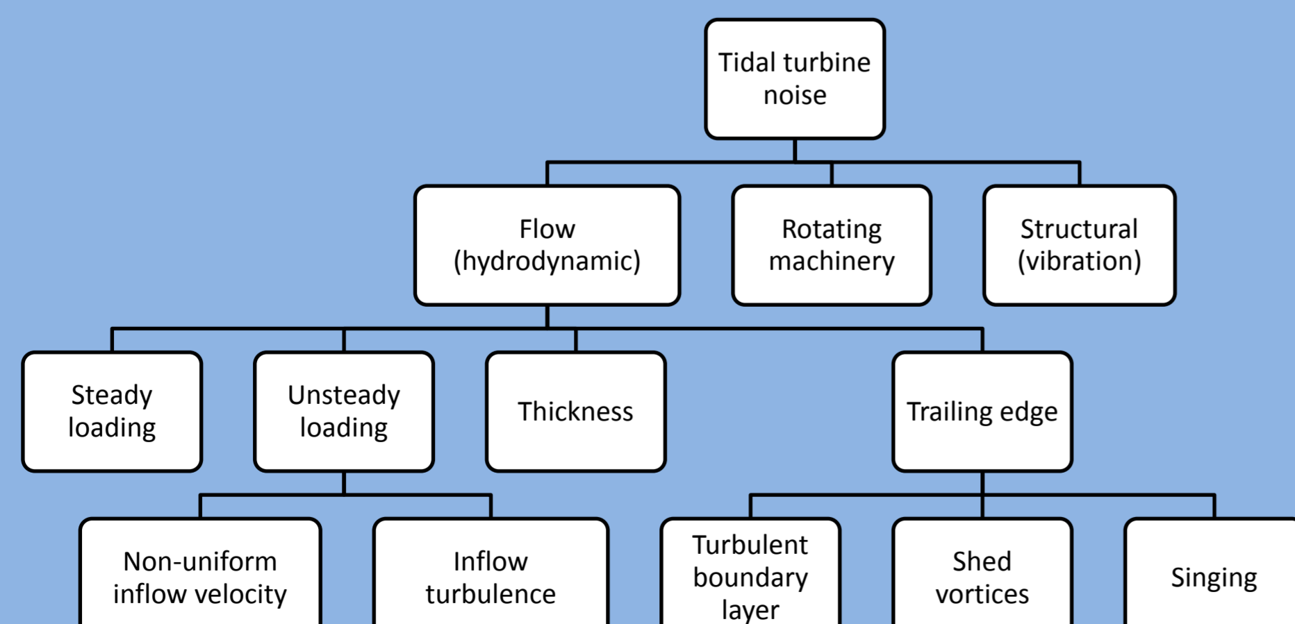
Figure 3: Classification of noise sources associated with tidal turbine
