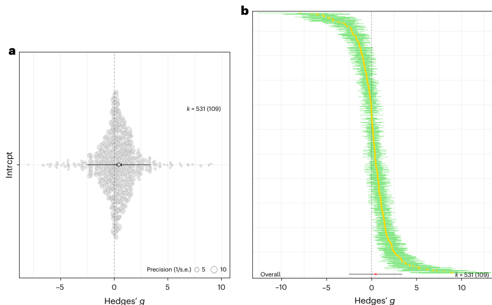
Fig. 2 | Overall ecological effect of MAS. The overall meta-analytic model shows significant moderate positive effects of MAS on marine ecosystems compared with sites without structures present ( t_{108} = 3.7249 , P = 0.0003 ). a , Visualized using an orchard plot. Individual effect sizes from studies are represented as grey bubbles. The dot represents the estimated mean Hedges' g value 0.47. The bold error bars represent the 95% confidence interval (95% CI 0.22, 0.73). The thin
