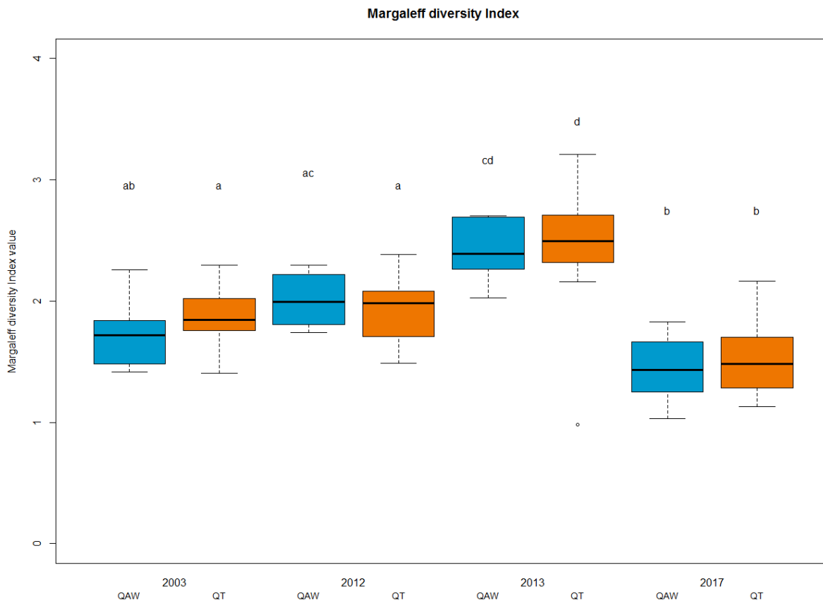
Figure 5-8: Margalef diversity calculated from the species data in the wind park (QT, orange) and adjacent waters (QAW, blue) over the four years. Similar letters above the individual boxes indicate no significant difference between the different levels of the year-park combinations (QT and QAW), based on Tukey's HSD post-hoc multiple comparisons ( p > 0.05 ).
