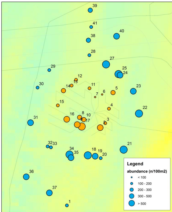
Figure 5-20: Benthic fauna abundance (n/100 m 2 ) found in the wind park (yellow) and outside the wind park (blue) (from: Leewis & Klink, 2017).
