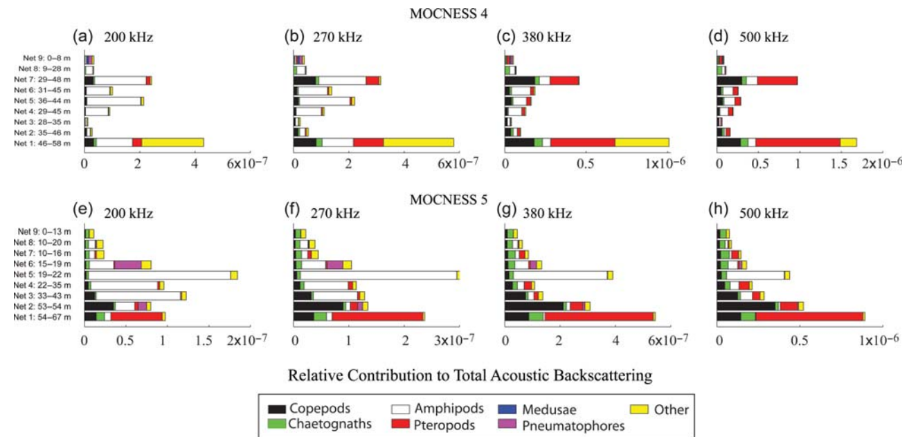
Figure 6. Relative predicted contribution to total scattering from different zooplankton collected in (a–d) the MOCNESS 4 (24 August 2006), and (e–h) the MOCNESS 5 (26 August 2006) at the centre frequencies of the four channels.
