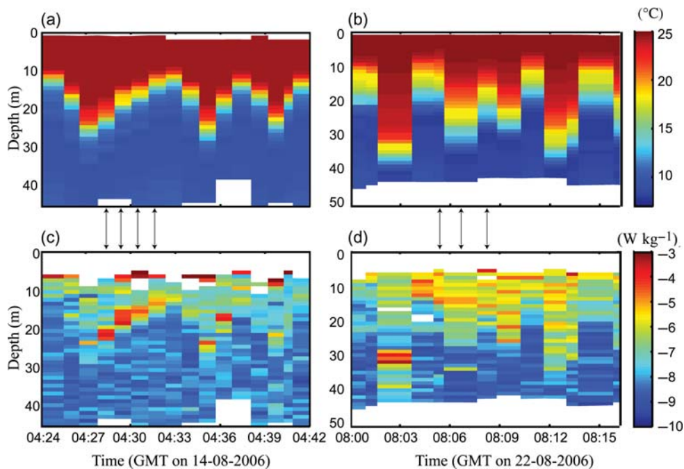
Figure 8. (a and b) Temperature ( ^{\circ}\text{C} ) and (c and d) dissipation rate of turbulent kinetic energy, \varepsilon ( \text{W kg}^{-1} ), on a log scale, as measured by the direct microstructure profiler on 14 and 22 August 2006. The measurements were collected at the same time as the broadband acoustic data illustrated in Figure 7. The arrows indicate the profiles plotted in Figure 11 for comparison with the acoustic inferences of \varepsilon .
