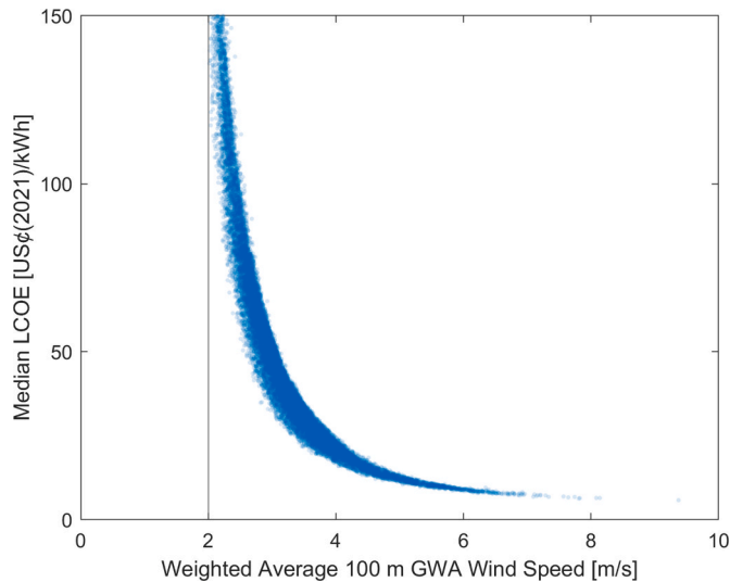
Fig. 6. Median leveled cost of electricity vs. weighted average 100 m GWA wind speed per meshed polygon. For clarity, the graph is limited to wind speeds \geq 2 m/s and \text{LCOE} \leq 150 US¢(2021)/kWh as the LCOE move towards infinity at smaller wind speeds.
