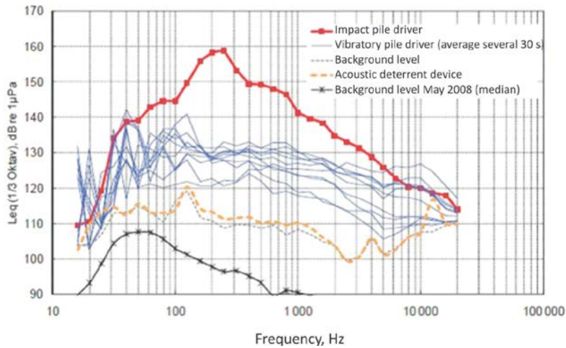
Figure 41: Sound level during the application of a vibratory pile driver in the OWF alpha ventus at the converter platform AVO (BETKE & MATUSCHEK 2009), compared to the impact pile driver and the background noise, measured at 1.2 km distance (source: BETKE & MATUSCHEK 2010, modified)
