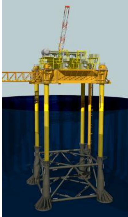
Figure 68: Platform founded on buckets for water depths of 50 m and deeper (source: Overdick GmbH & Co. KG, Hamburg )
