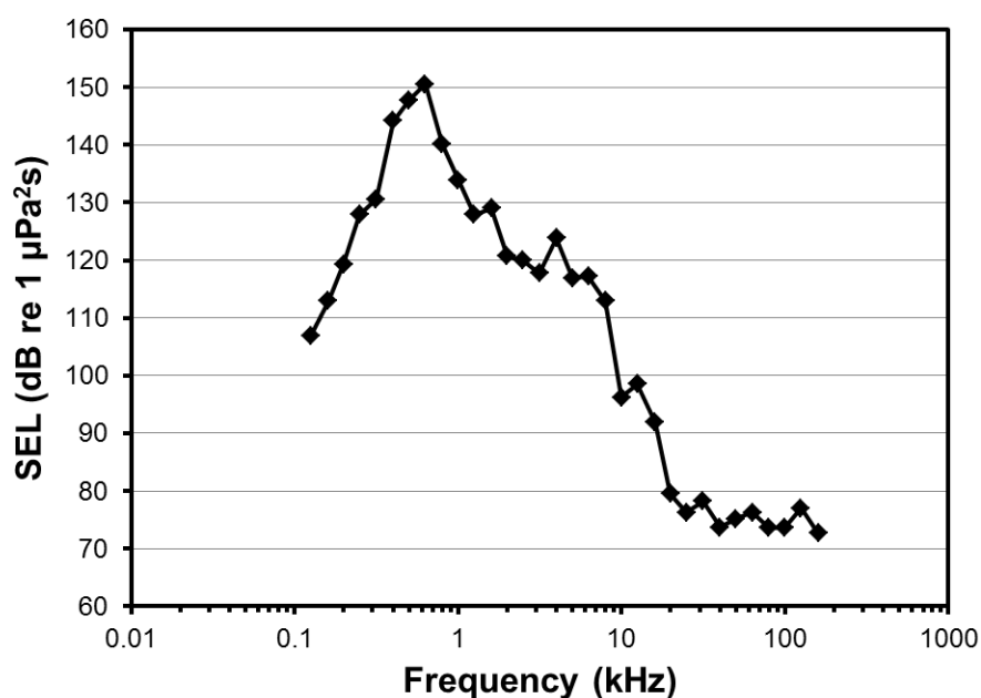
FIG. 1. The 1/3-octave band spectra of the SEL of a single played back pile driving sound in the pool. Measurements were conducted at 1 m depth, 2 m from the source. At the measurement location, the signal had a SEL of 155 dB re 1 \mu\text{Pa}^2\text{s} , and an L_{z-p} of 179 dB re 1 \mu\text{Pa} . The average received sound exposure level was 146 dB re 1 \mu\text{Pa}^2\text{s} , and the 1/3-octave band centered at 630 Hz contained the most energy.
