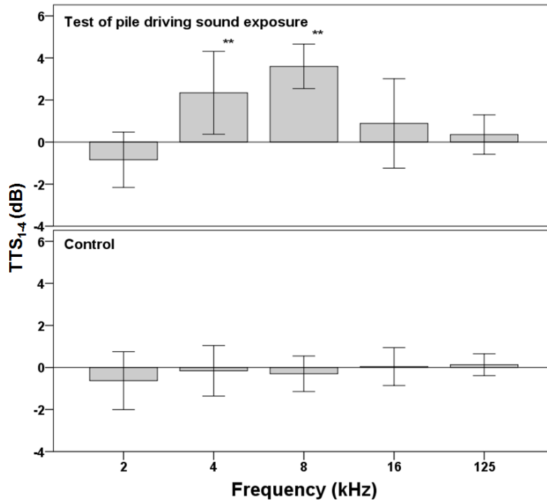
FIG. 3. Mean TTS_{1-4} in the harbor porpoise, (a) 1-4 min after exposure to playback of a series of pile driving sounds for 60 min at a mean received SEL of 146 dB re 1 \mu Pa^2 s ( SEL_{cum} : 180 dB re 1 \mu Pa^2 s ) (exposure condition), and (b) after exposure to the low ambient noise for 60 min (control condition). n = 7 for each frequency tested per condition. ** indicates a significant difference between the exposure condition and the control condition (one-tailed t -test; P < 0.01 ).
