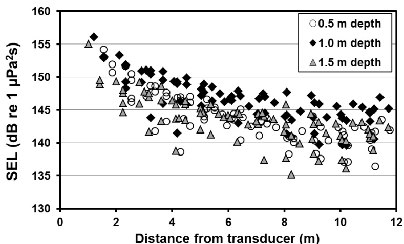
FIG. 2. The SEL distribution in the outdoor pool when the pile driving sound, as fatiguing noise, was being played back (231 measurement locations; 77 per depth). Per location, the SEL did not vary much per depth, and only a very small SEL gradient occurred in relation to the distance to the transducer. These data were used to calculate the level of the average received sound exposure (dB re 1 \mu\text{Pa}^2\text{s} ) that the harbor porpoise experienced during a single noise exposure: 146 \pm 4 dB re 1 \mu\text{Pa}^2\text{s} (mean \pm SD; n = 231 ).
