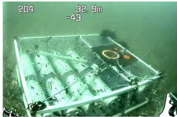
Figure 3 - FLOWBEC platform during deployment at EMEC from Williamson et al. 2017.
