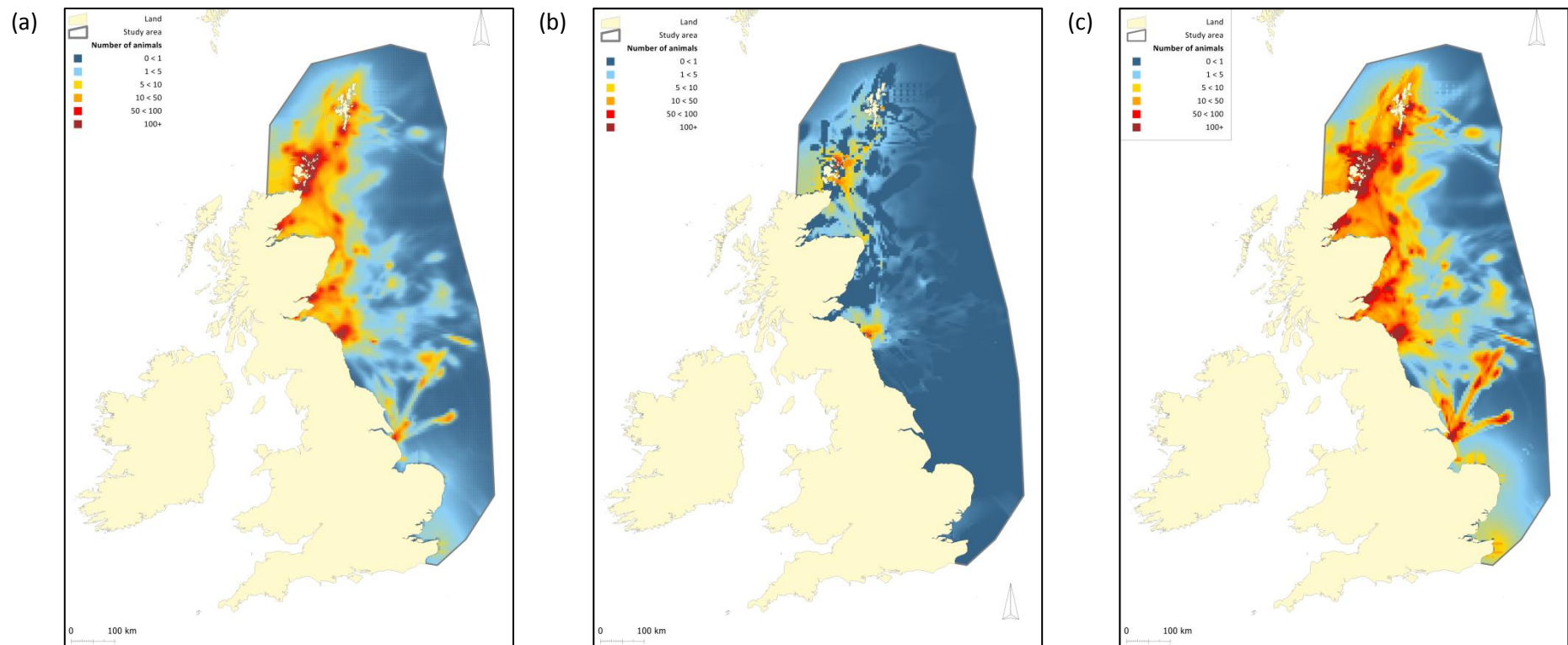
Figure 5. 5 km x 5 km usage maps produced for the Scottish Government in 2013. Adapted from Jones et al. (2013). Grey seal at-sea North Sea usage map showing number of animals in each 5 km x 5 km grid cell within the study area (a), as well as the lower (b) and upper (c) 95% confidence intervals.
