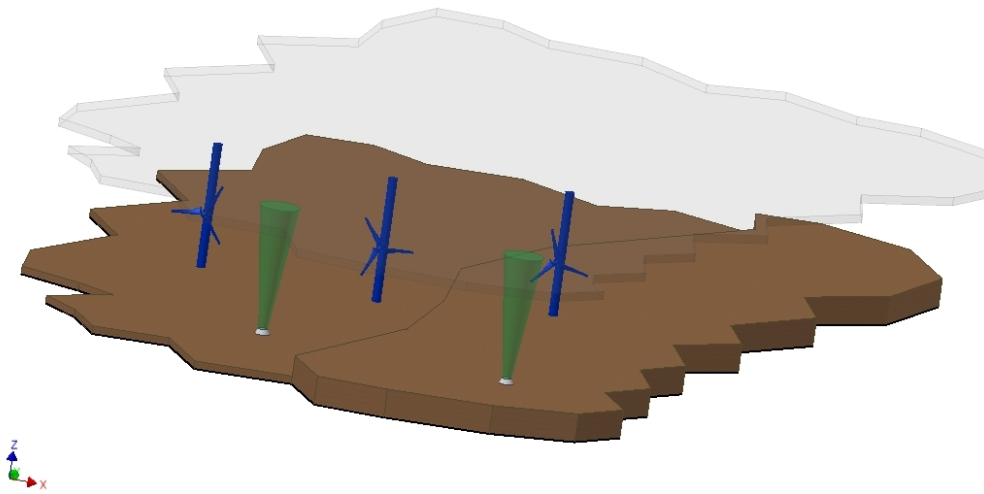
Figure II.C.12: Tidal Array installation over varying depth will require increased measurement to accurately define inflow conditions.
