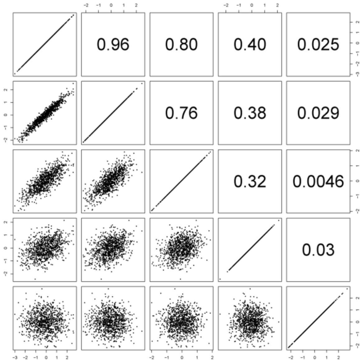
Figure II.A.8: Linear Correlation Example. Taken from Wikimedia.
