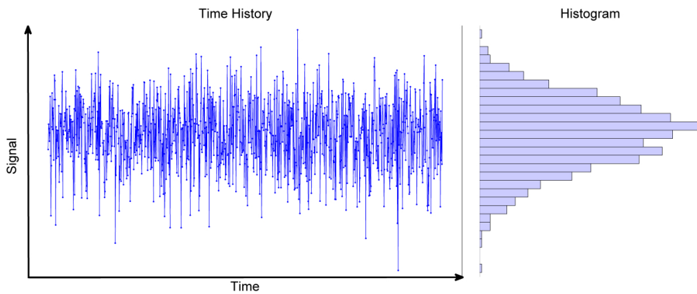
Figure II.A.4: Illustration of a noisy time series of data, and the associated histogram of values.
