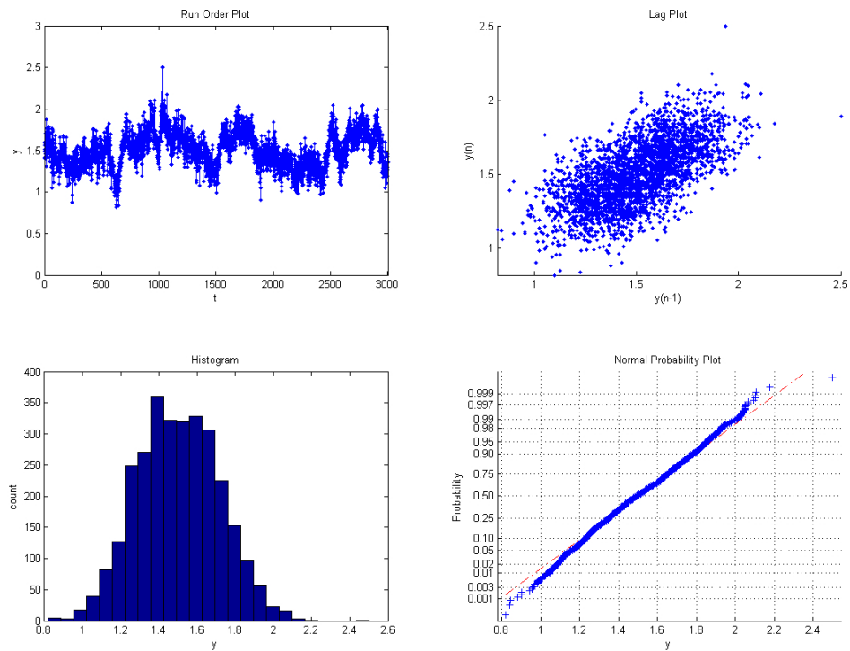
Figure II.A.7: The 4-Plot for a data series.
