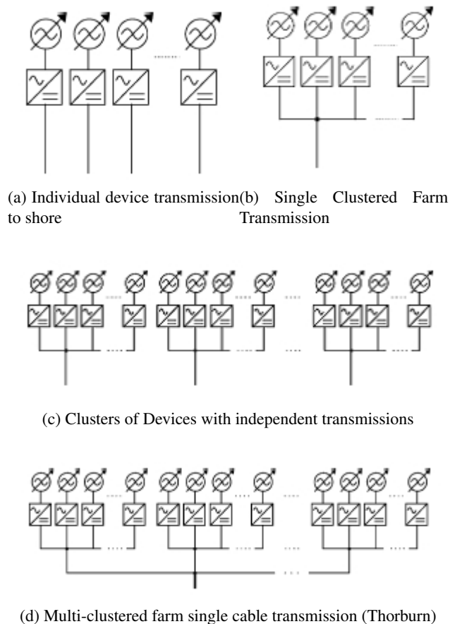
Figure II.C.5: Electrical integration configurations
