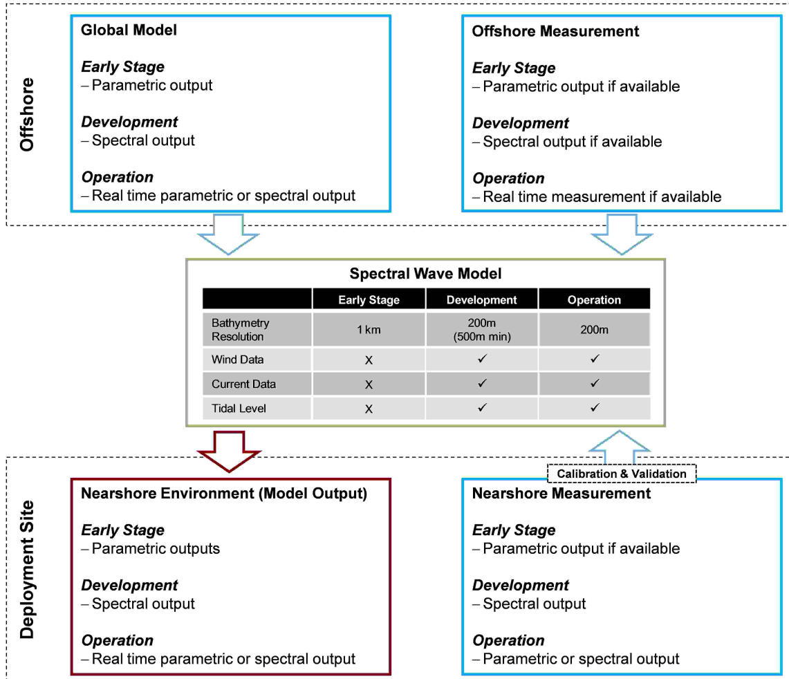
Figure I.A.8: Summary of the required inputs and expected outputs for numerical modelling for wave energy resource assessment.
