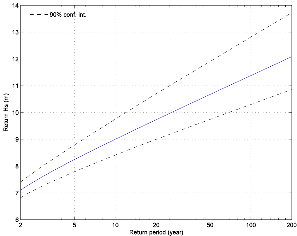
Figure I.A.14: Typical representation of return values.
