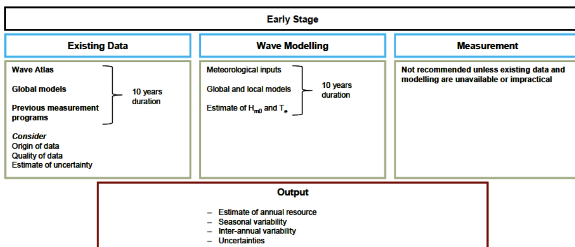
Figure I.A.2: Resource assessment for the early stage aspect of a wave energy development.
