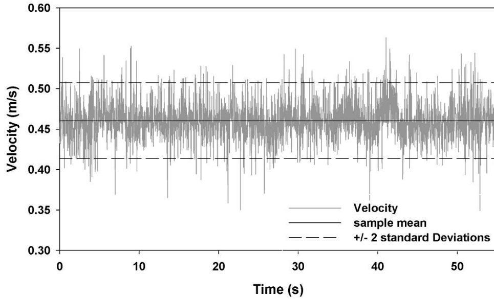
Figure II.A.6: Velocity measurement in a towing tank facility
