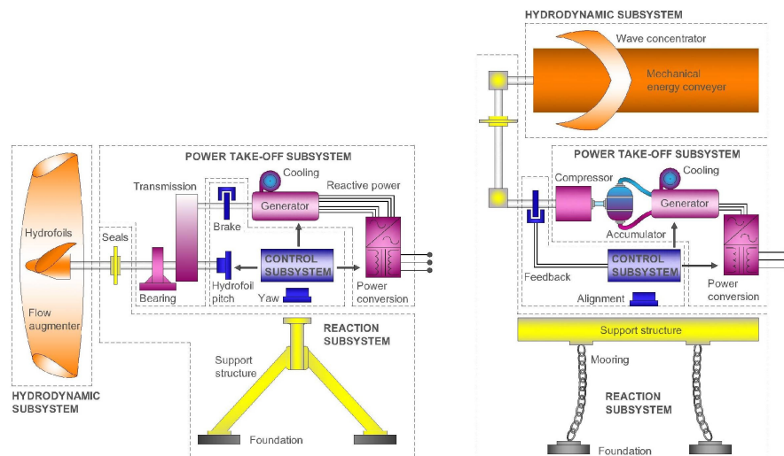
Figure II.C.1: Schematic subsystem diagram of tidal (left) and wave (right) energy devices
