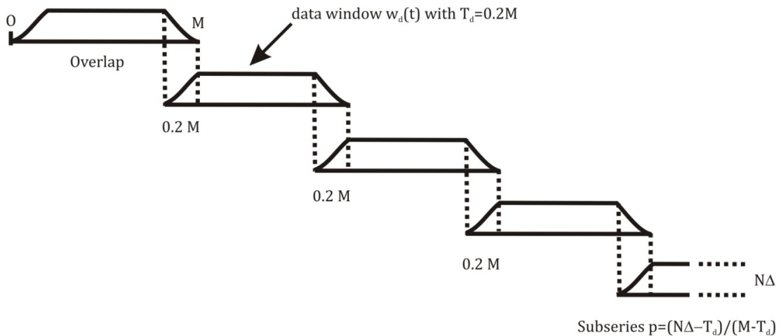
Figure II.A.5: Illustration of windowing, tapering and overlapping.
