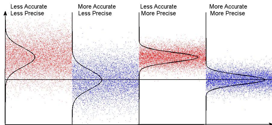
Figure II.A.2: Illustration of Precision and Accuracy components of experimental uncertainty, and also the notion of a probability density function.
