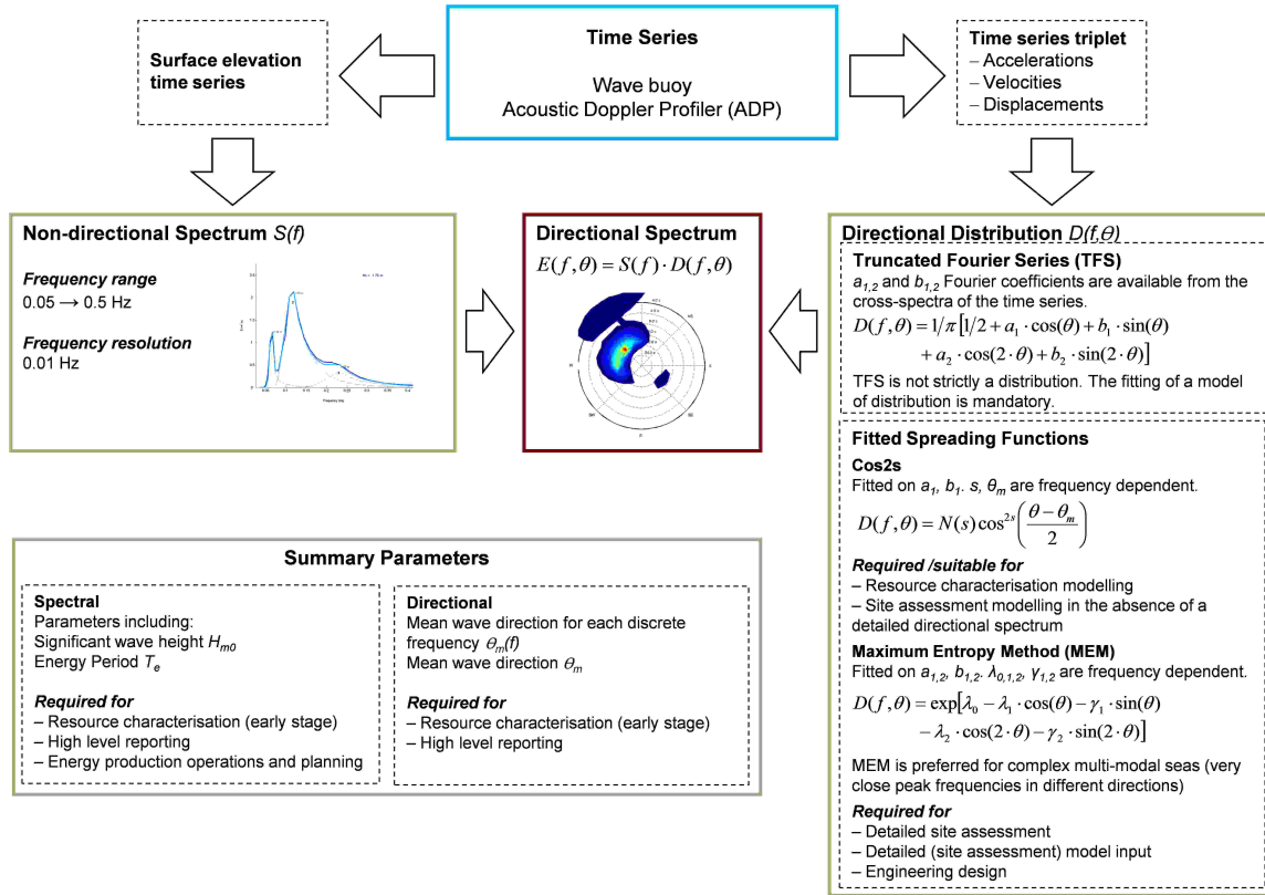
Figure I.A.7: Calculation of the directional spectrum from raw time series data.
