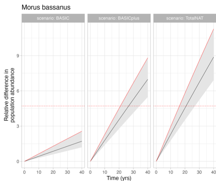
Figure 5.1 Main output of the population model, calculated as the relative difference in final population size between the unimpacted and the impacted scenario, for each of the scenarios (panels). Solid black line represents the median outcome, red solid line the 95 th percentile, and the red dashed line indicates the threshold.
