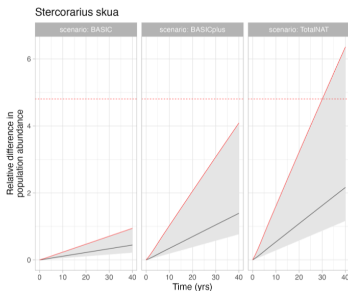
Figure 5.3 Main output of the population model, calculated as the relative difference in final population size between the unimpacted and the impacted scenario, for each of the scenarios (panels). Solid black line represents the median outcome, red solid line the 95 th percentile, and the red dashed line indicates the threshold.
