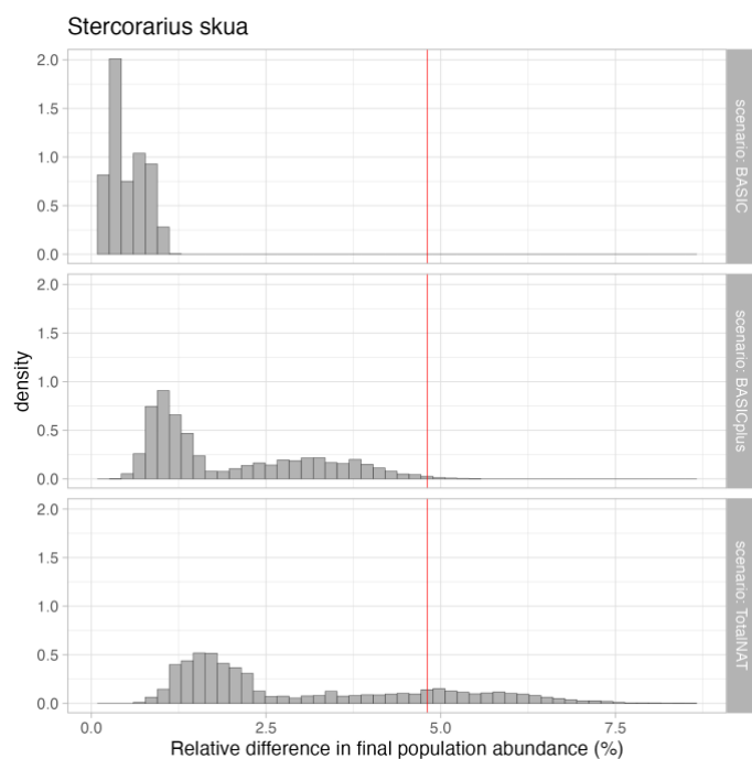
Figure 5.4 Density distribution of relative differences in final population abundance (grey bars). Red line indicates the threshold for an unacceptable decline. The ALI is violated when more than 5% of the simulations have an unacceptable decline (above the red line), which is the case for the TotalNAT scenario.
