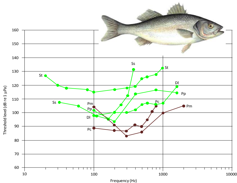
Figure 3: Hearing curves for European seabass and other benthopelagic fish species: Dl = Dicentrarchus labrax (seabass, Fam. Moronidae). Seabass are most sensitive in the range of 100-400 Hz and also hear up to 1000 Hz, but become rapidly insensitive to sound at higher frequencies. Ss= Salmo salar (salmon, Fam. Salmonidae); St= Salmo trutta (sea trout, Fam. Salmonidae); Pp= Pungitius pungitius (nine-spined stickleback, Fam. Gasterosteidae); Pm= Pagrus major (red seabream, Fam. Sparidae); Pc= Pogonias chromis (black drum, Fam. Sciaenidae). Green = species of the North Sea. Brown = species of the same family as a species of the North Sea area (from Bouton et al. SONIC-report 2015).
