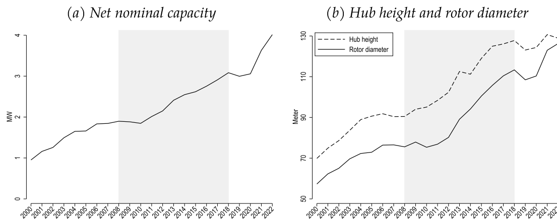
Fig. 7. Development of wind turbine characteristics over time. Notes: The shaded area indicates the sample period of the econometric analysis.
