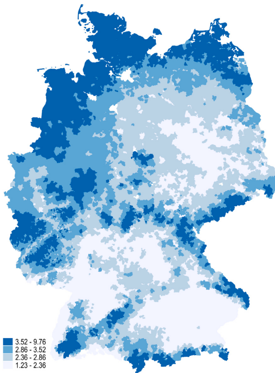
Fig. 5. Wind potential in Germany.
