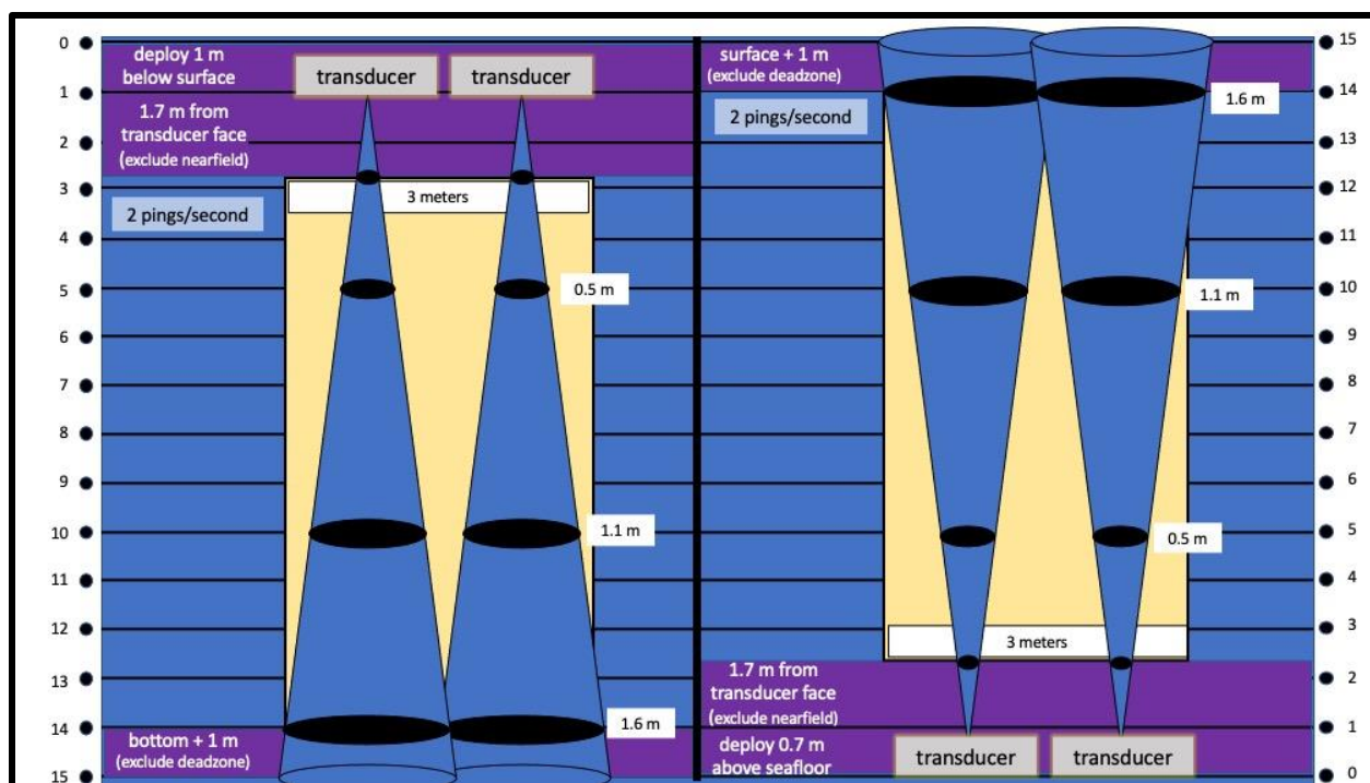
Figure 4.3.6: Echosounder Beam Diameter and Proportion of Water Ensonified at 2 Hz. This graphic illustrates the ensonifying cones ( blue cone ) of an echosounder acoustic beam for a downward-facing transducer deployed at the surface ( left ) and an upward-facing transducer deployed at the sea floor ( right ). Ping rate is 2 Hz. All other assumptions are as specified in Figure 4.3.5.
