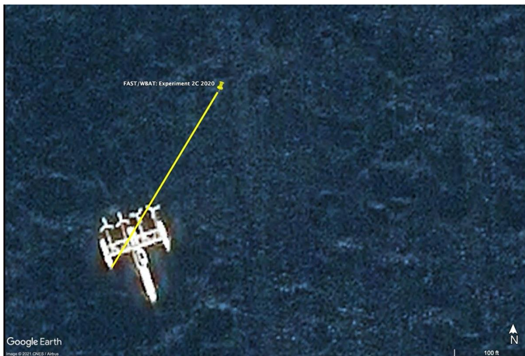
Figure 3.4.2: Deployment location of the WBAT echosounder mounted on the FAST platform, shown for Study 2C relative to the PLAT-I on a flooding tide. Length of yellow line represents the horizontal length from the EK80 echosounder deployed at the leading edge of the starboard pontoon to the position of the FAST platform: ~85 m.
