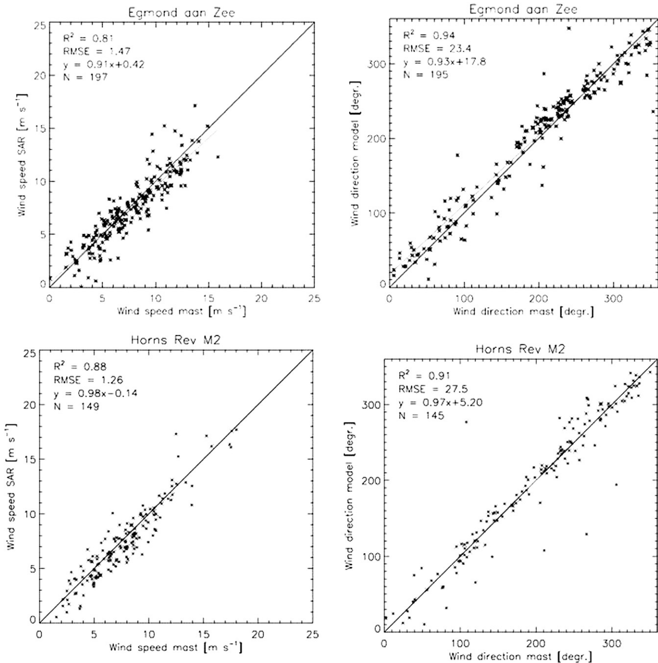
Fig. 6. Comparison of wind speed (left) and wind direction (right) of observations at the meteorological mast and SAR-based wind maps using CMOD-IFR2 for winds in the range 0–25 m s^{-1} for Egmond aan Zee (above) and Horns Rev M2 (below) for equivalent neutral winds at 10 m. The correlation coefficient squared ( R^2 ), root mean square difference (RMSE), linear regression slope and intercept, and the number of samples ( N ) are included. Few samples of wind direction are omitted near 0^\circ/360^\circ .
