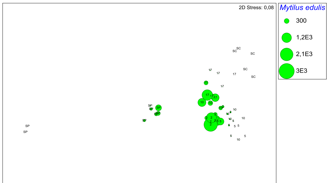
Figure 14: MDS of biomass of Mytilus edulis ; samples are indicated with the depth value
