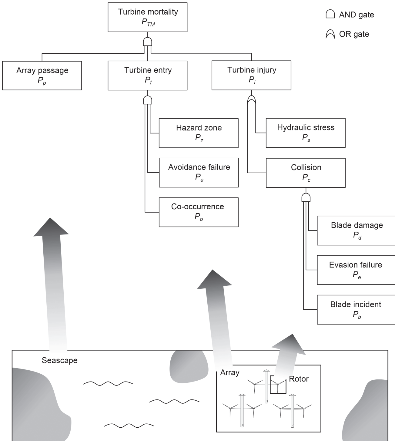
Fig 1. The generic collision risk model described as a fault tree diagram. Turbine mortality is the top event. Intermediate events are connected to basic events through AND gates and OR gates. The probability of each basic event is case-specific and should be assigned using applied equations or estimates. If detailed data on fish movements within the array are available P_o will be accurate and P_p can be removed (see section on P_o ). The lower panel indicates how the P_p , P_t and P_i deals with events at the scale of population range, at the scale of the array and turbines and at the scale of the rotor blades, respectively. Each basic event, referred to as model components, is examined in the main text and an example of model implementation is provided.
