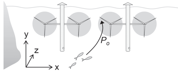
Fig 3. Conceptual representation of the probability of co-occurrence ( P_o ) for fish passing through a turbine array. P_o is the probability that a given specimen that passes through an area with tidal turbines, during times when rotors are rotating, will come across a rotor. P_o can be described as the combined probabilities of the fish moving along current ( z ) at the same depth ( y ) and horizontal position ( x ) as the rotors. These probabilities are influenced by the particular behavior of fish swimming in strong currents.
