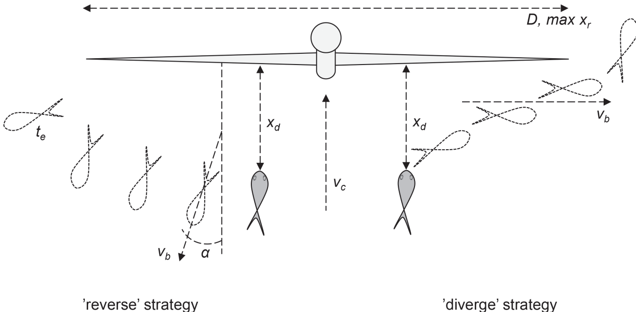
Fig 8. Representation of the two modeled avoidance strategies for a fish approaching a turbine. In these simplified models of fish avoidance D denotes the rotor diameter, defining the maximum swimming path of avoiding fish. x_r is the random position on the rotor disc where the fish appears when approaching the turbine and x_d is the distance at which the fish detects the turbine. x_r is the required swimming path, defining the distance that the fish has to swim to reach safety. v_b denotes the fish burst speed and \alpha is the angle that reversing fish take in order to keep the turbine in the rear view while swimming away. t_e is the time to exhaustion for reversing fish, which defines the time in which the fish has to cover the required swimming path to safety (outside the rotor swept disc).
