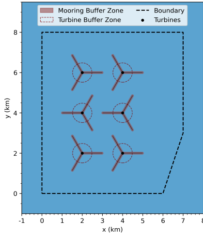
(a) Initial layout
