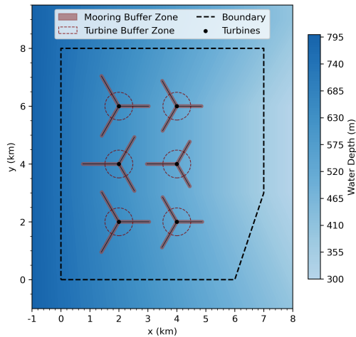
(a) Initial layout
