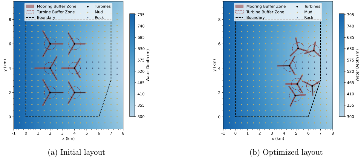
Figure 7: Minimizing CapEx on sloped seabed with varied soil (8.7% mooring cost reduction).
