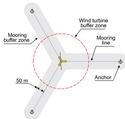
Figure 3: Spatial boundaries around a wind turbine
