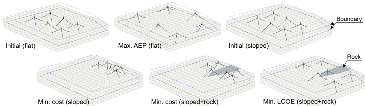
Figure 9: MoorPy three-dimensional model of the layouts in Table 2
