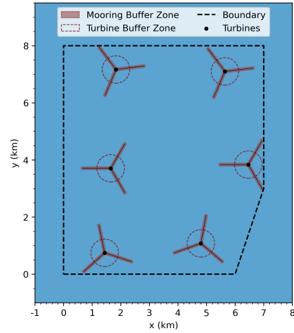
(b) Optimized layout
