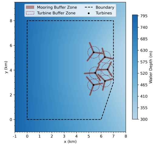
(b) Optimized layout
