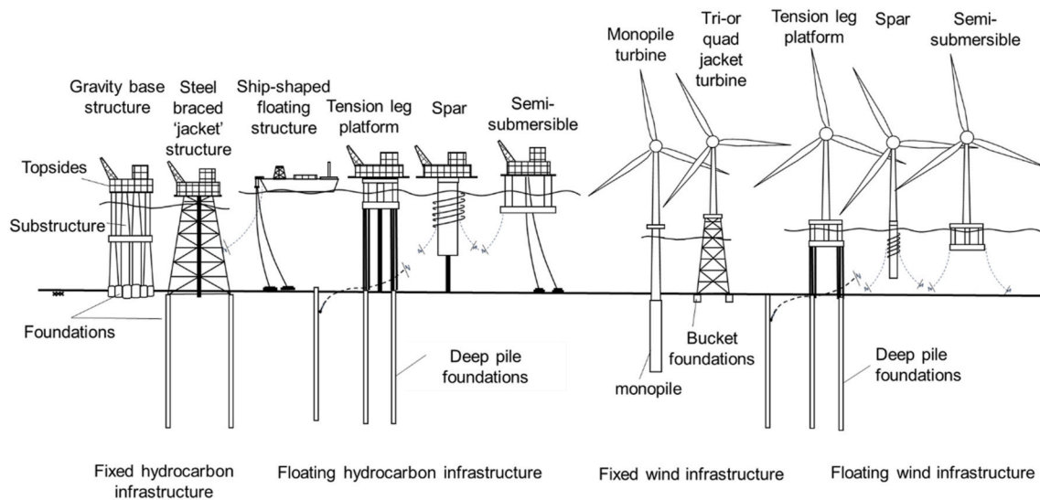
Fig. 4. Examples of offshore infrastructure for hydrocarbon and wind energy.
