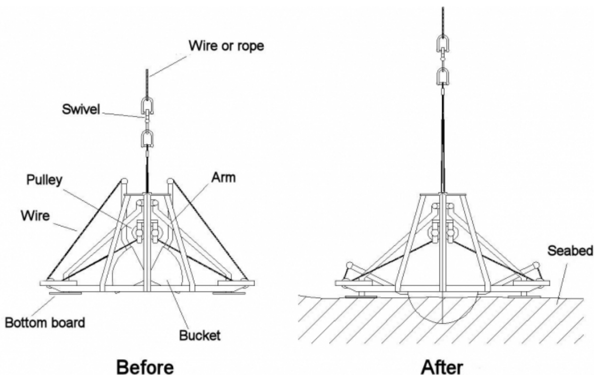
Figure 6.7. Schematic diagram of grab sampler before closing the bucket to capture the sample (left) and after grabbing the sample from seafloor (right)
