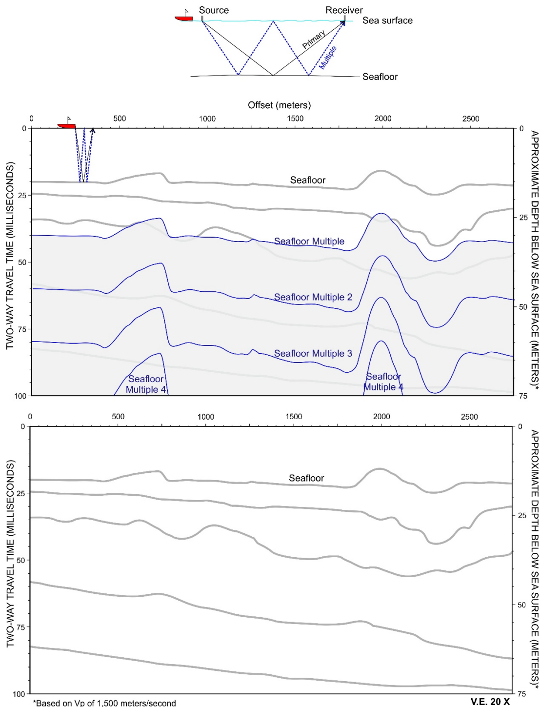
Figure 2.3. Schematic of water bottom multiples in seismic reflection data
