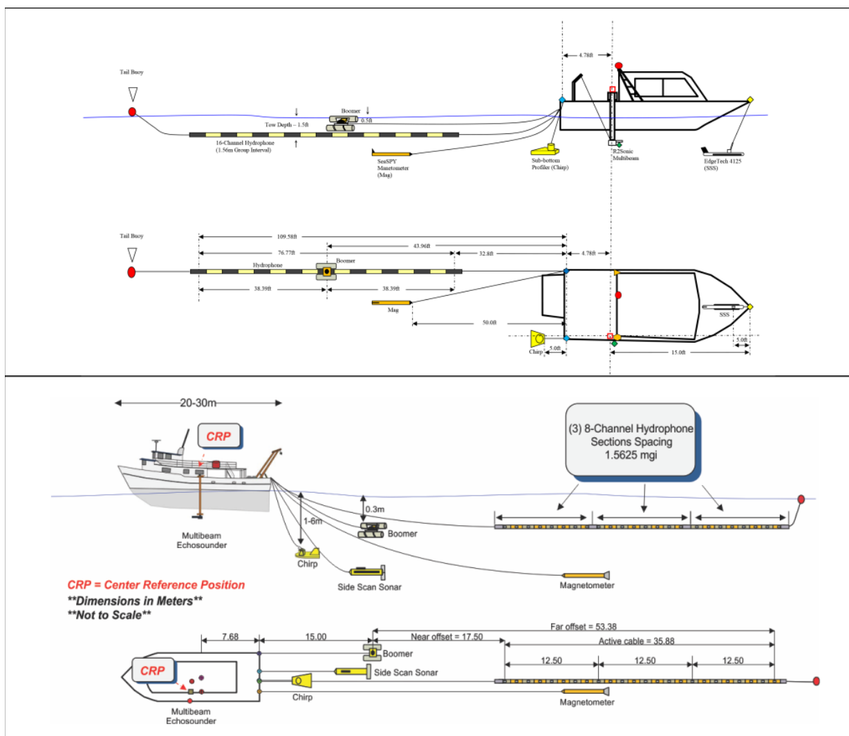
Figure 6.9. Example HRG survey configuration.
