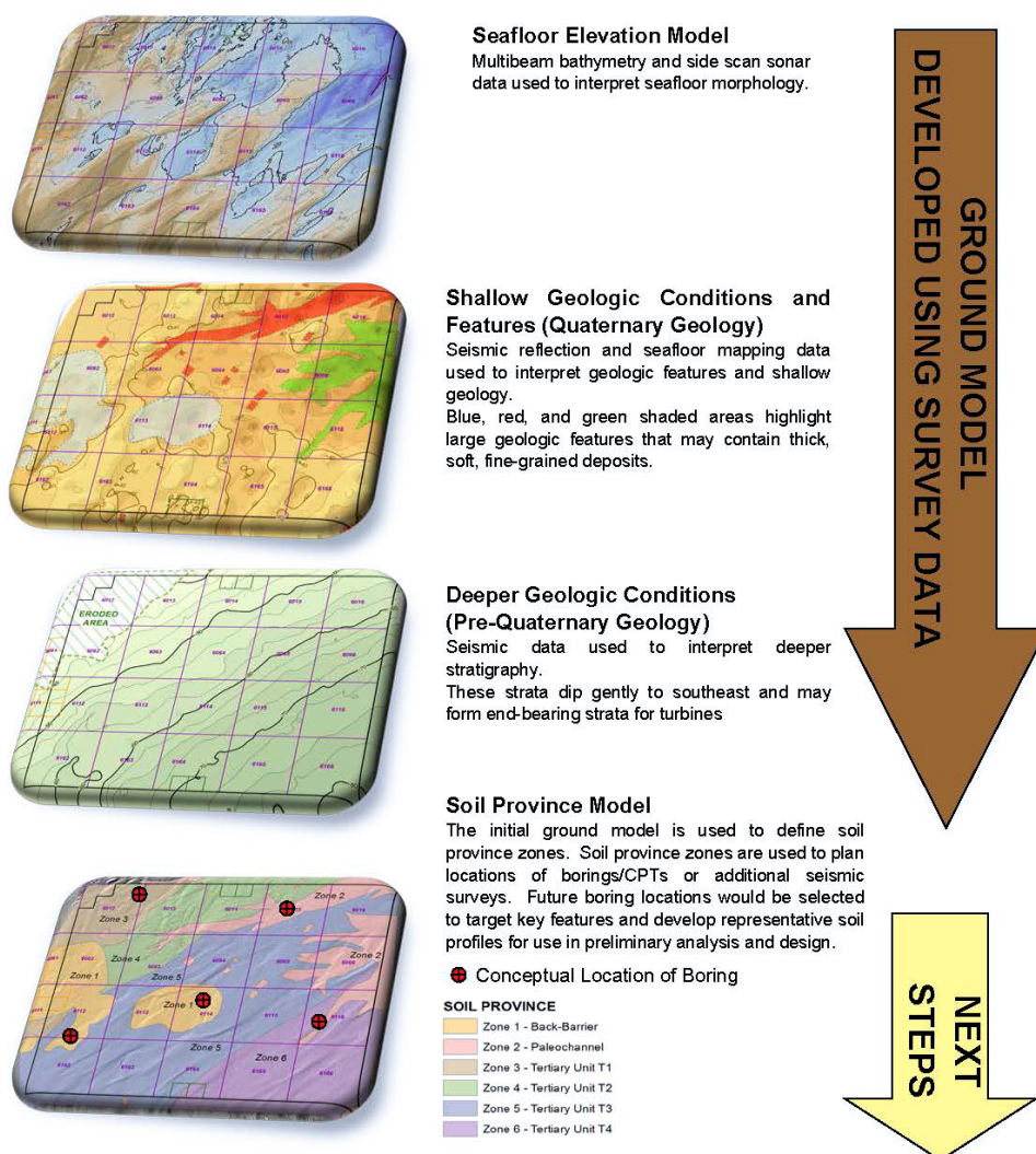
Figure 4.1. Using marine survey data to develop initial ground model Marine survey data are the first project-specific data used to define ground conditions
