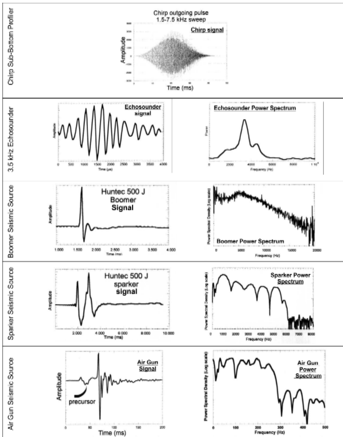
Figure 6.14. Example seismic source signatures
