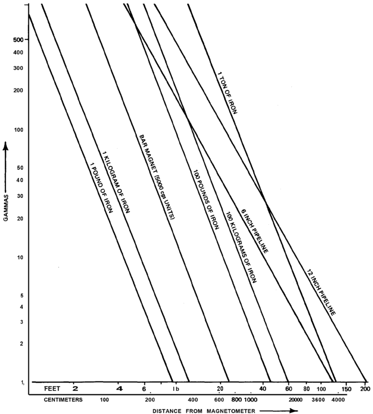
Figure 2.2. Nomogram for estimating anomalies from typical objects assuming dipole moment, M = 5 \times 10^5 cgs/tom, i.e., k = 8 cgs). Estimates valid only within an order of magnitude (Breiner, 1999)
