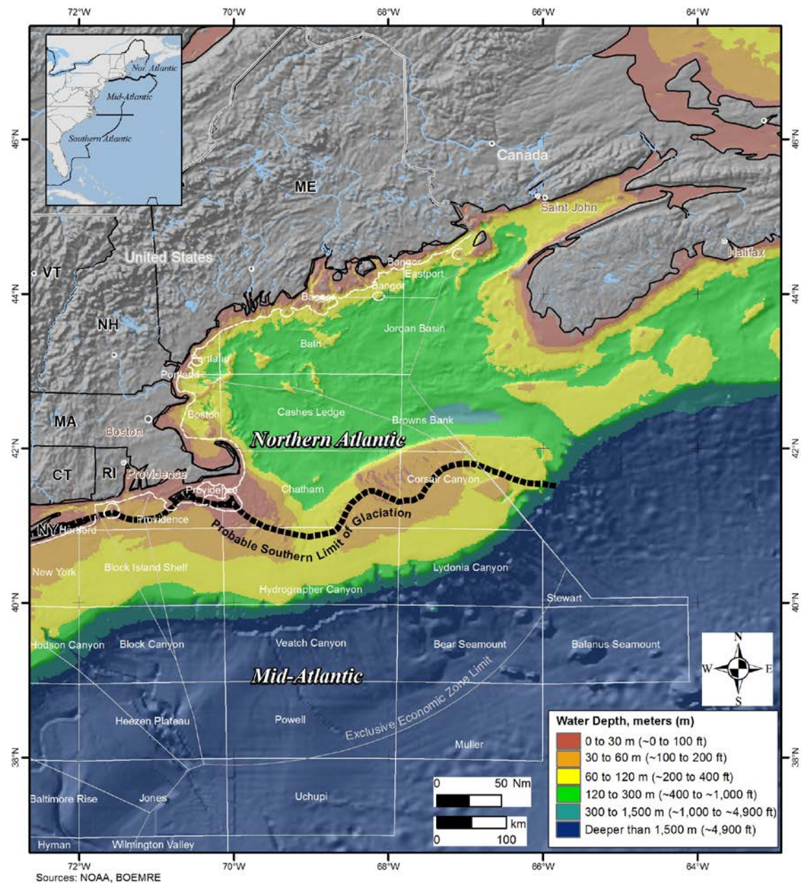
Figure 1.1. Water depths within the Northern Atlantic OCS
