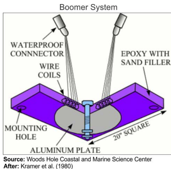
Figure 6.15. Boomer source schematic in cross section view
