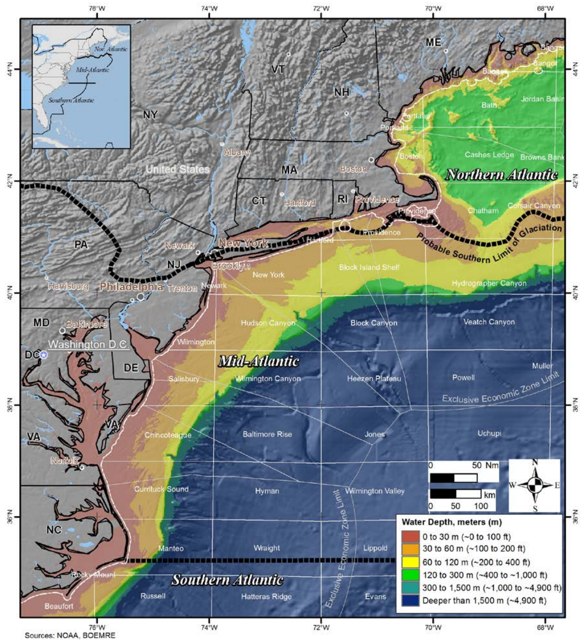
Figure 1.2. Water depths within the Mid-Atlantic OCS
