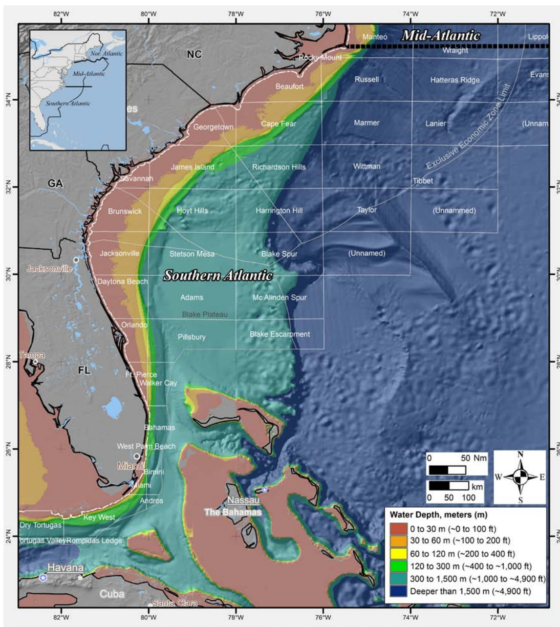
Figure 1.3. Water depths within the Southern Atlantic OCS
