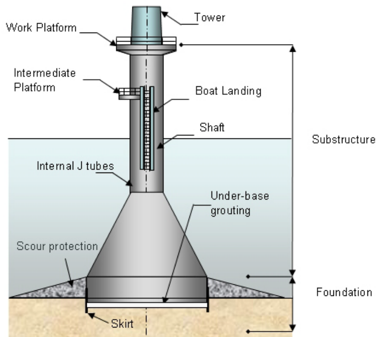
Figure 1.7. Schematic diagram of a gravity-based foundation system (Source: Mott MacDonald: “Offshore Wind – IEEE Boston PES”, 11/16/2010)
