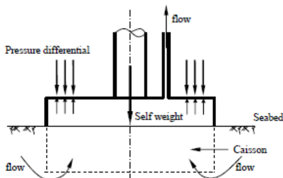
Figure 1.5. Installation schematic of suction caissons
