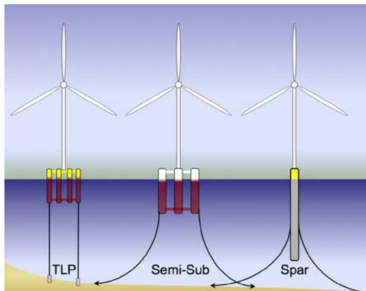
Figure 1.11. Schematic diagram of different floating wind turbines
