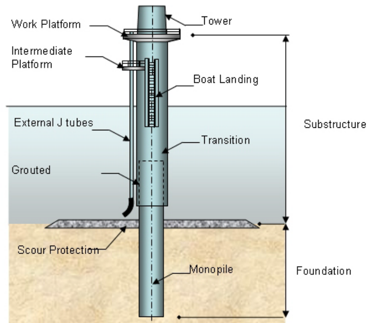
Figure 1.6. Schematic diagram of a monopile foundation system (Source: Mott MacDonald: “Offshore Wind – IEEE Boston PES”, 11/16/2010) – Pending approval from BOEM and Mott MacDonald
