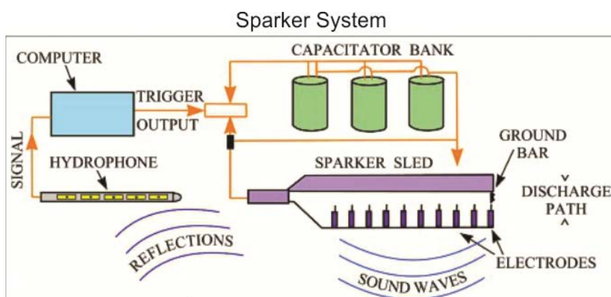
Figure 6.17. Sparker source schematic
