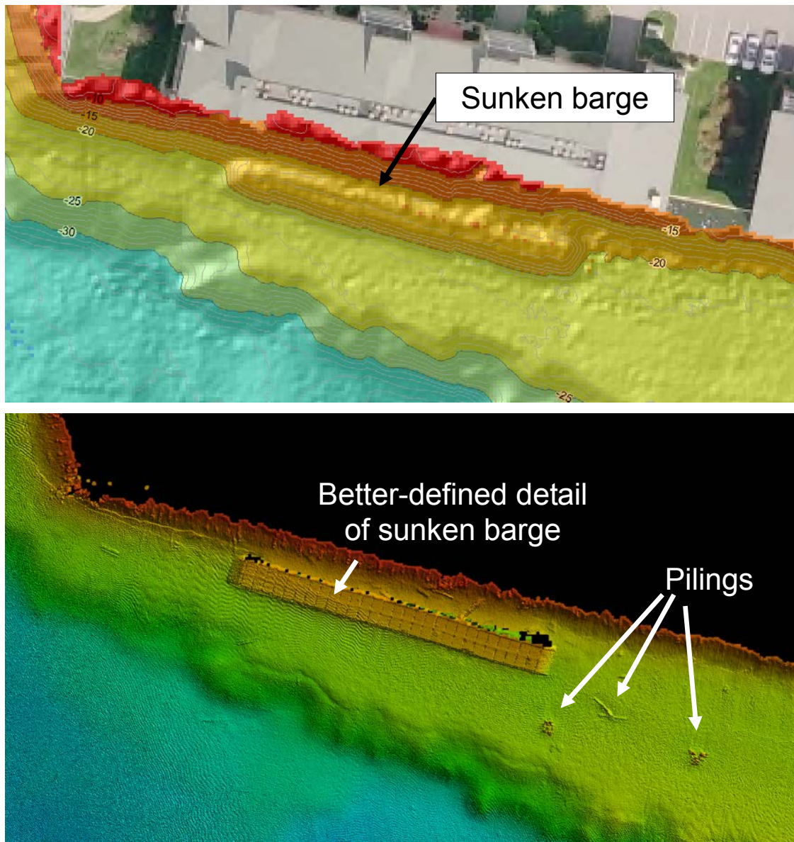
Figure 2.1. Comparison of bathymetric data density
