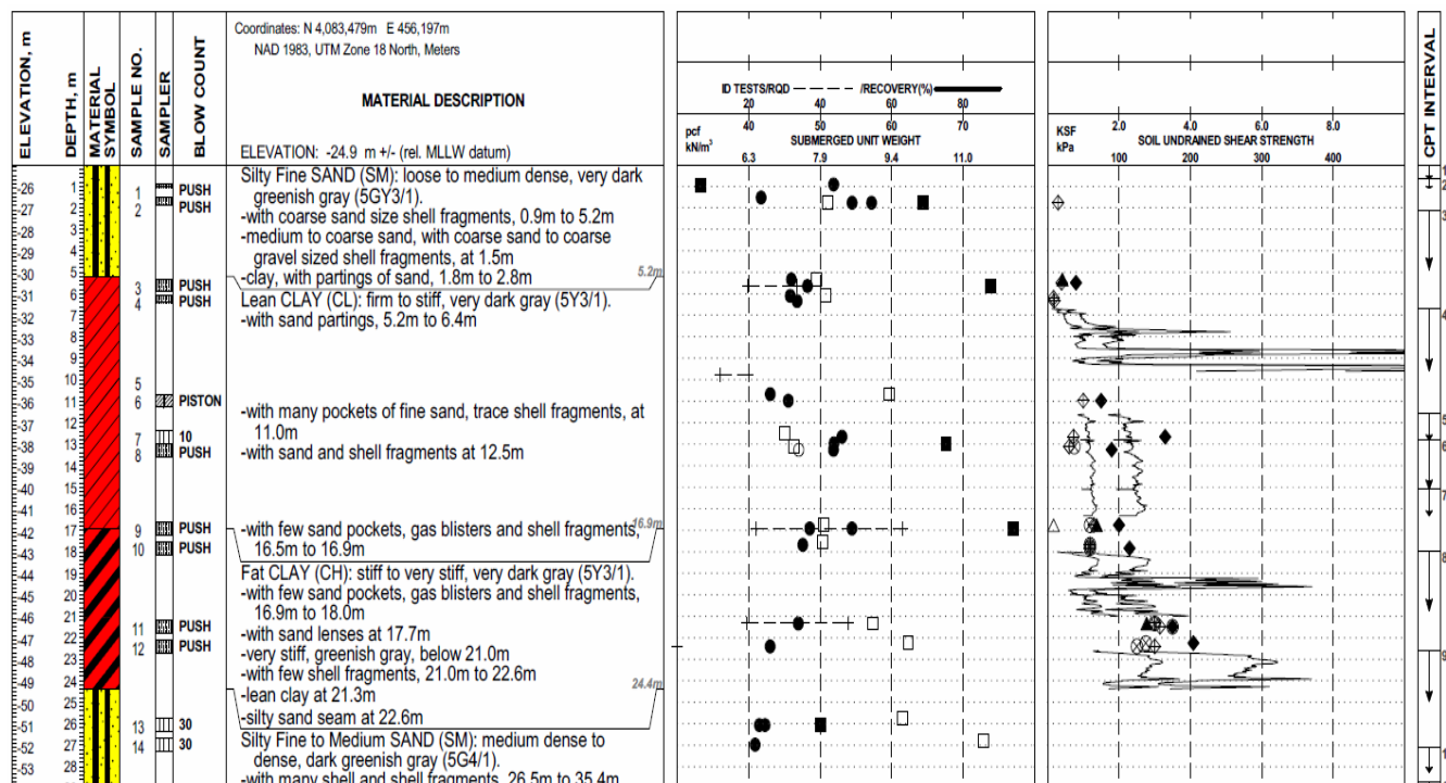
Figure 6.8. Example of a borehole log for offshore projects
