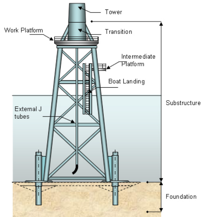
Figure 1.8. Schematic diagram of a jacket foundation system (Source: Mott MacDonald: "Offshore Wind – IEEE Boston PES", 11/16/2010)
