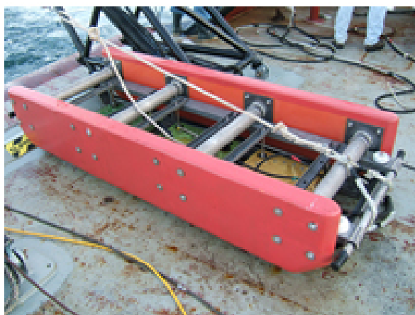
Figure 6.16. Triple-plate boomer source (Courtesy of Subsea Systems, Inc.)
