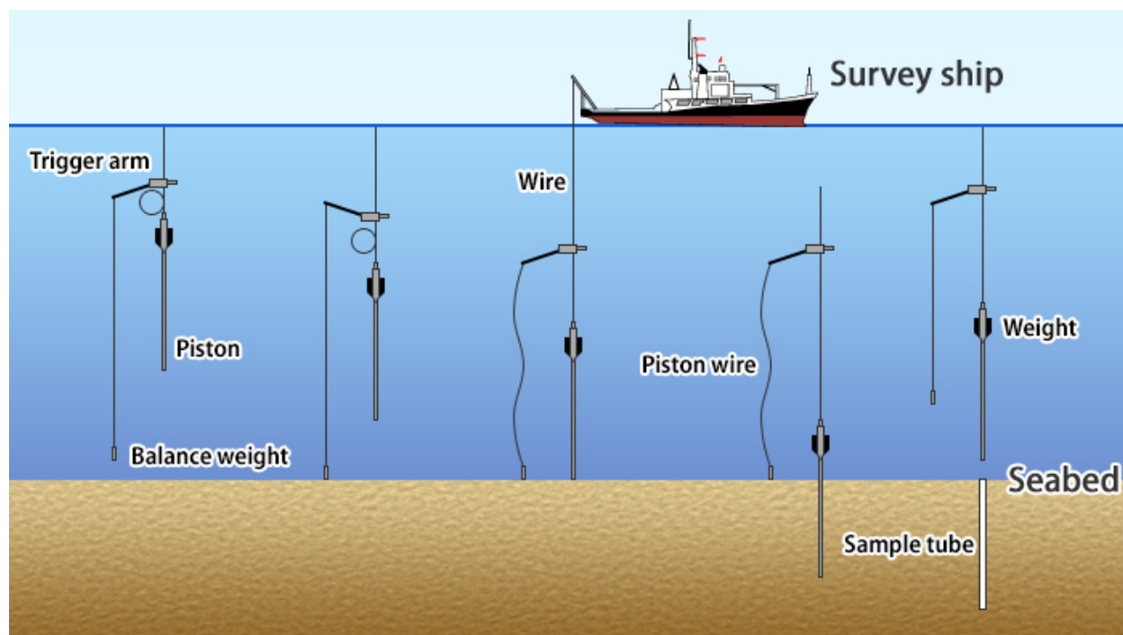
Figure 6.6. Schematic diagram of the deployment of piston sampler 2
