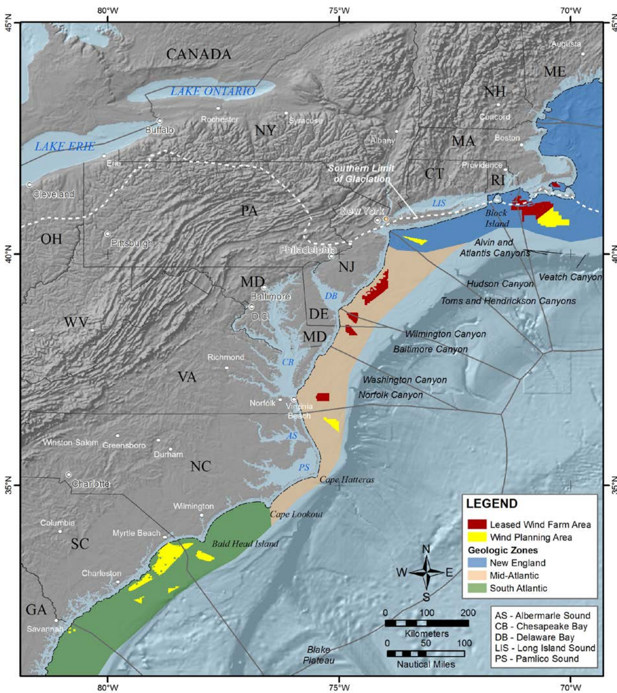
Figure 1.4. Regional geologic zonation
