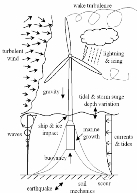
Figure 1.12. Sources of loading on offshore wind turbines (Source: Butterfield et al., 2005)
