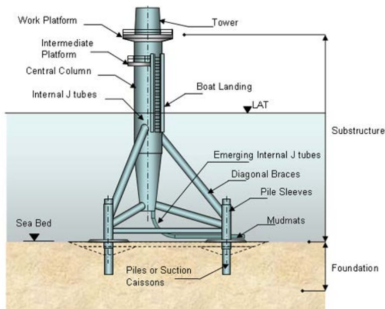
Figure 1.9. Schematic diagram of a tripod foundation system (Source: Mott MacDonald: "Offshore Wind – IEEE Boston PES", 11/16/2010)
