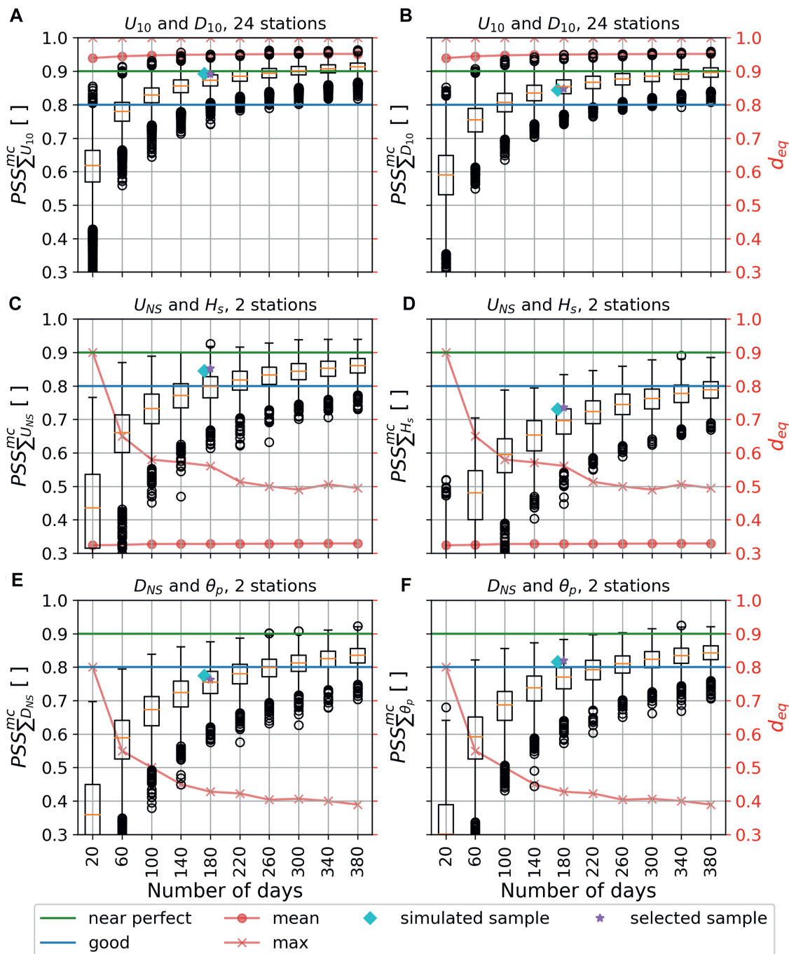
FIGURE 6 | Same as Figure 3 , but for (A,B) the projected two-dimensional distributions 10-m wind speed, U_{10} , and direction, D_{10} , (C,D) near-surface wind speed ( U_{NS} ) and significant wave height ( H_s ), and (E,F) near-surface wind direction ( D_{NS} ) and peak wave direction ( \theta_p ).
