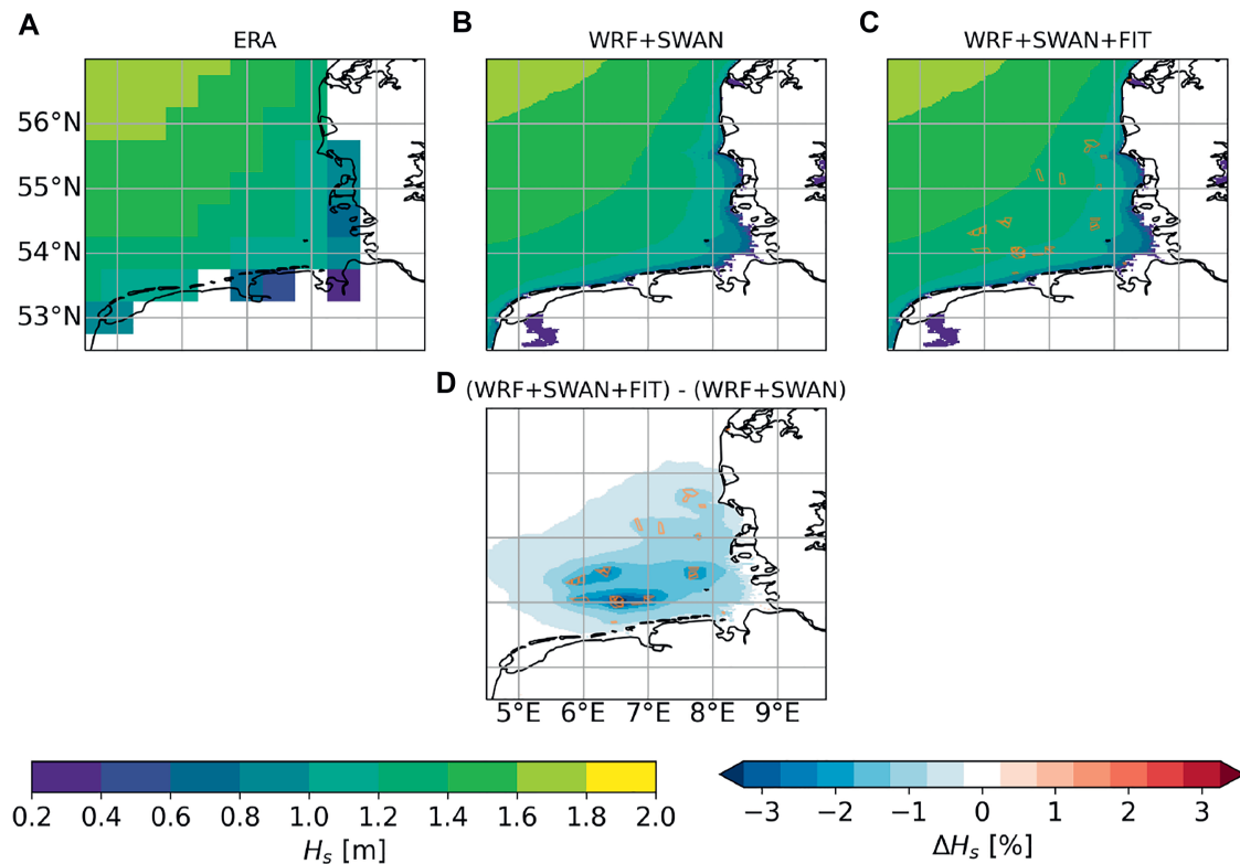
FIGURE 13 | (A) Long-term significant wave height ( H_s ) from ERA5 and simulated by (B) WRF + SWAN and (C) WRF + SWAN + FIT. (D) Relative reduction on significant wave height from (WRF + SWAN + FIT)-(WRF + SWAN) normalized by (WRF + SWAN).
