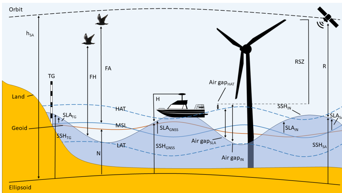
Figure 1.1. Schematic plot of the relationship between measures of sea surface height (instantaneous – SSHIN, satellite altimetry – SSHSA, tide gauge – SSHTG, GNSS – SSHGNSS), two commonly used reference altitudes (mean sea level – MSL, a modelled geoid) and a wind turbine. The instantaneous sea level anomaly (i.e. difference between measured and reference value) is shown for each method (instantaneous – SLAIN, satellite altimetry – SLASA, tide gauge – SLATG, GNSS – SLAGNSS). Measures of flight height (FH) refer to the distance between a flying bird and the instantaneous sea surface height while measures of flight altitude (FA) refer to the distance between a flying bird and a reference altitude. Turbine characteristics (e.g. RSZ, Air gap) are measured from the highest astronomical tide (HAT), the rotor swept zone (RSZ) refers to the area between the upper and lower limits of a turbines blades and the air gap refers to the distance between the RSZ and the HAT (Air gap HAT ). Both the instantaneous air gap (Air gap IN ) and the difference between this and the HAT value (Air gap SLA ) are also shown. Additional abbreviations include: hsa - ellipsoidal height, N – geoid undulation, R – distance between the satellite and the sea surface, H – GNSS antenna height from the sea surface. At the tide gauge, the geoid undulation (N) approximately coincides with the vertical datum zero N \approx \text{mean sea surface height above ellipsoid} .
