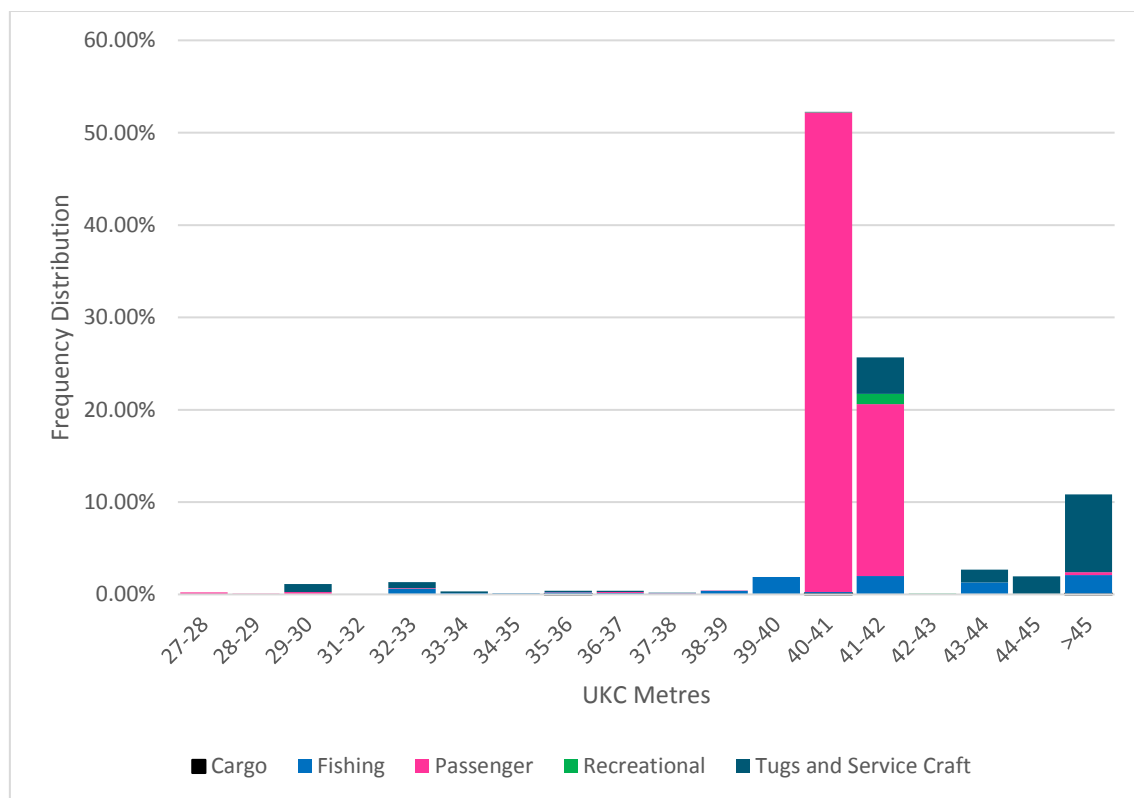
Figure 28: UKC for transits
