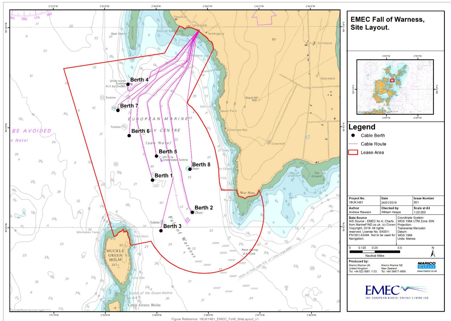
Figure 1: Test site layout at Fall of Warness.
