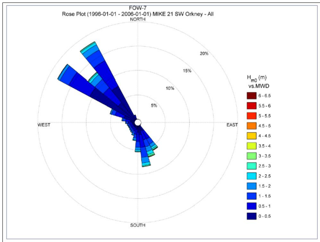
Figure 3: Wave rose plot for percentage occurrence with H_{m0} and direction (EMEC Fall of Warness – Berth 1: MecOcean & Physical Description 2015).
