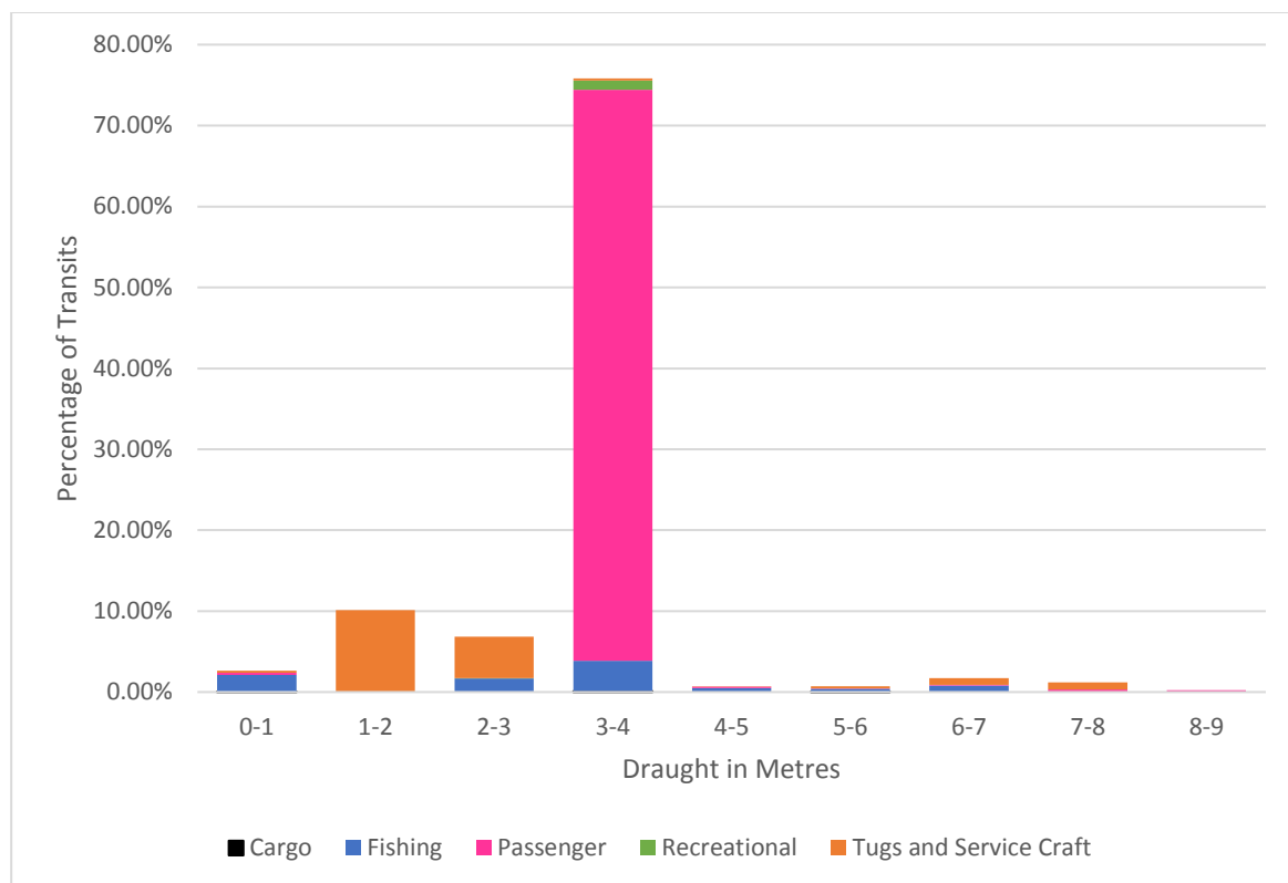
Figure 27: Vessel draught distribution within the site
