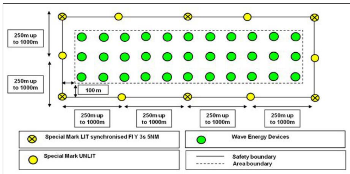
Figure 30: IALA recommendations on marking of wave and tidal devices.
