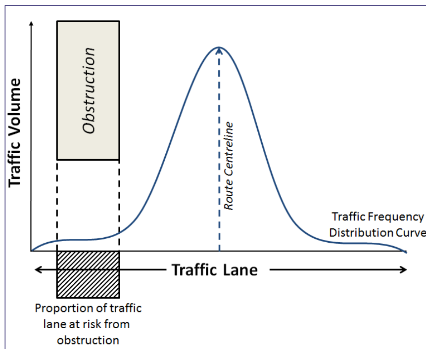
Figure 23: Risk Model.
