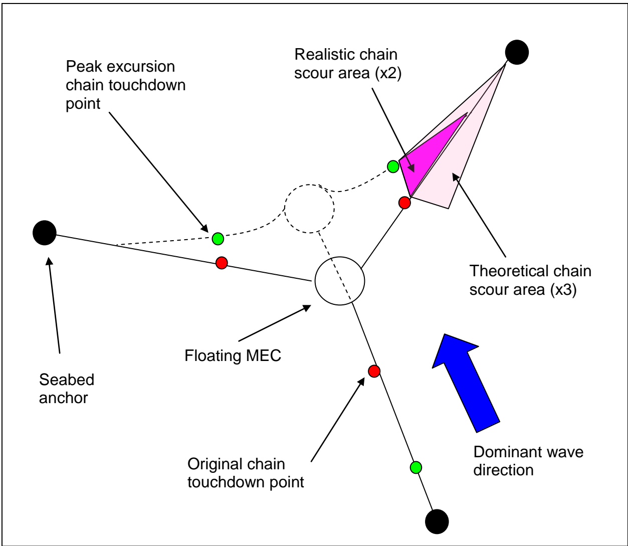
Figure 2: An illustration of realistic chain scour due to excursion
