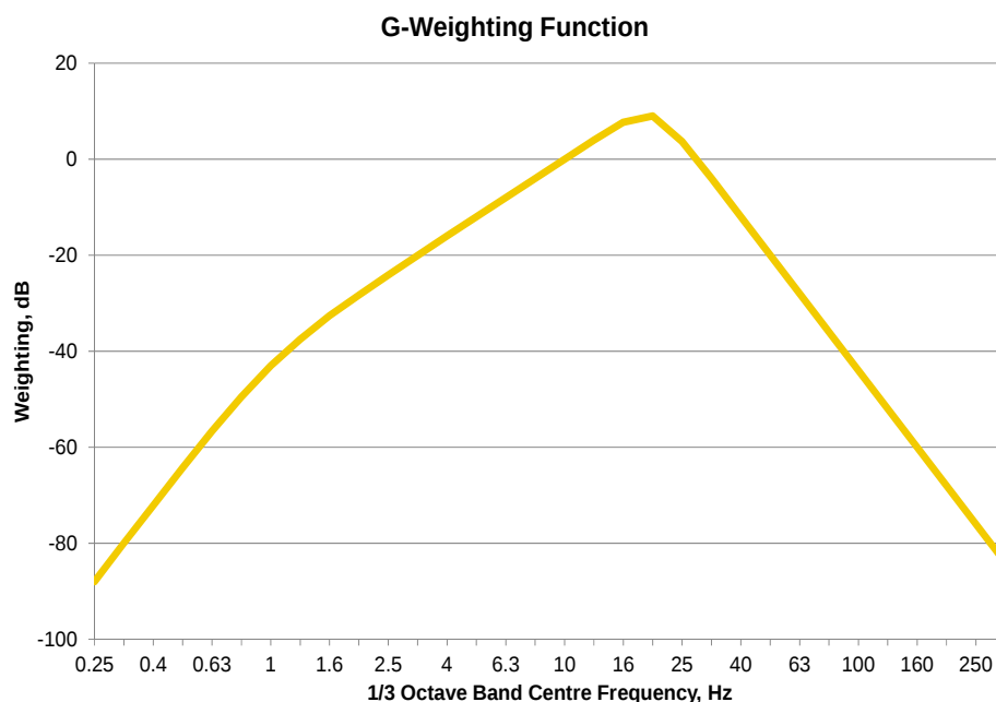
Figure 2 – G-weighting function
