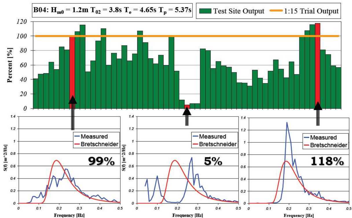
Figure 31 Example of different spectral shapes with the same summary seaway statistics[43]
