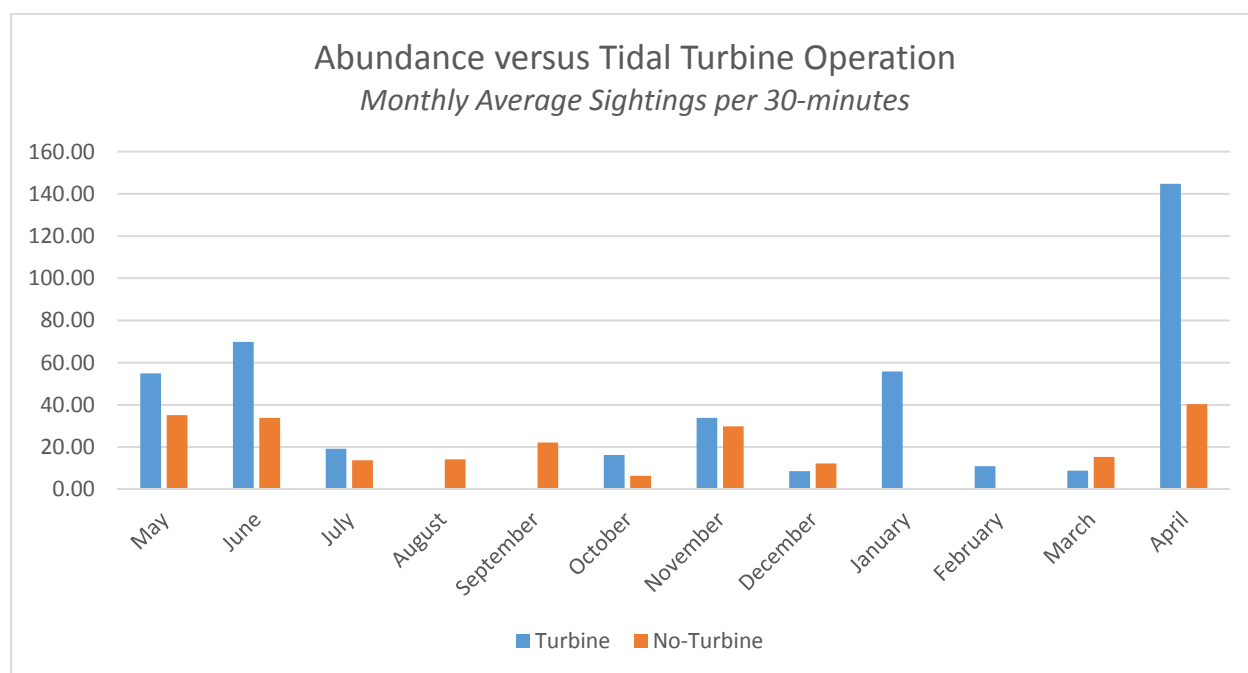
Figure 37. Abundance of seabirds and water-associated birds versus periods of turbine operation in shore-based surveys at the Fundy Ocean Research Center for Energy, Parrsboro, Nova Scotia.
