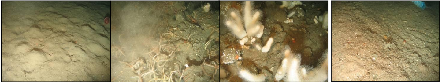
Plate 10: Typical seabed images showing the succession of different sediment types along transects across two selected boulder and cobble exposures within the proposed Neart na Gaoithe turbine array.
