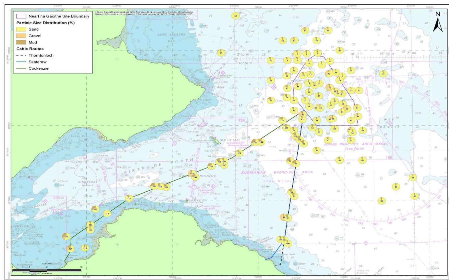
Figure 4.1: Distribution of principal sediment components (%gravel, %sand and %silt) across the Neart na Gaoithe survey area.
