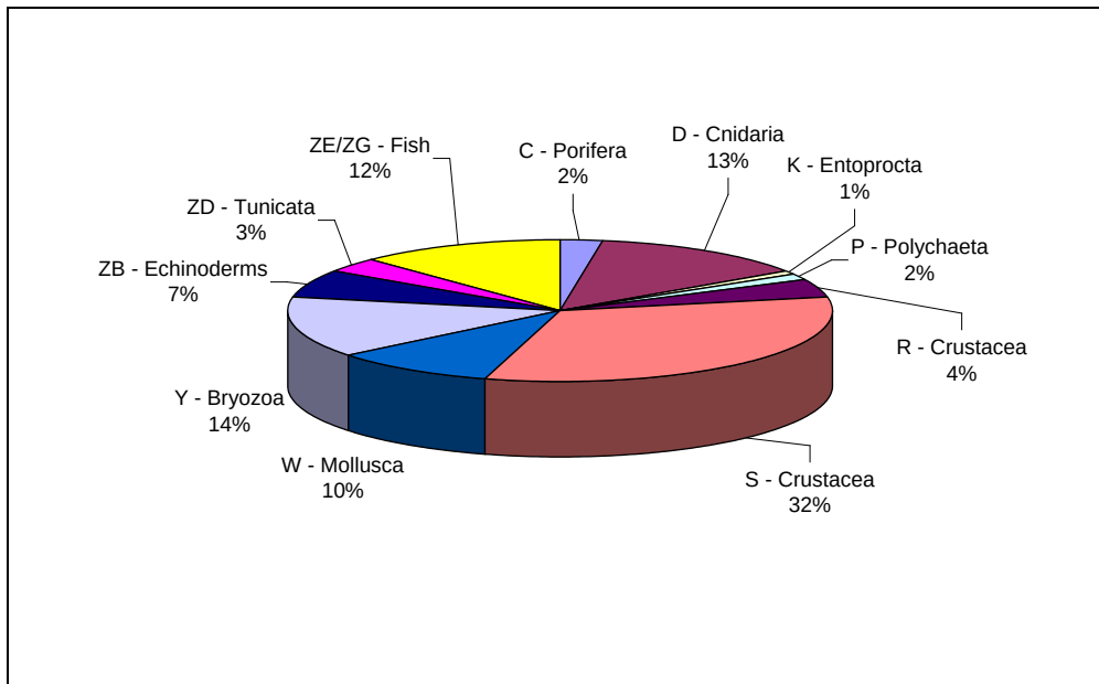
Figure 4.13: Percentage contributions of each major taxonomic group to the total species variety in 2 m beam trawl samples at Neart na Gaoithe.
