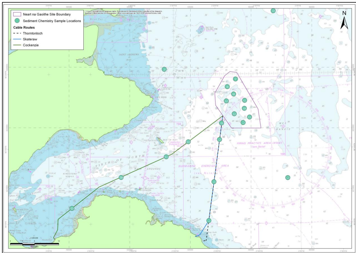
Figure 2.3: Location of sediment chemistry samples
