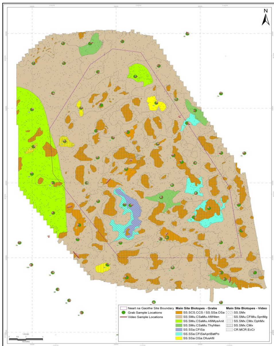
Figure 4.16: Biotope map of the proposed Near na Gaoithe turbine site.
