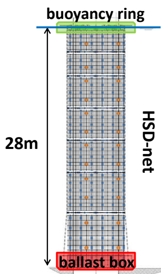
Figure 12. HSD-net, LA test,[5].
