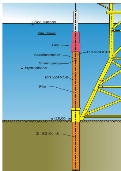
Figure 1. FINO1 foundation and impact energy., Elmer et. al. (2007)
