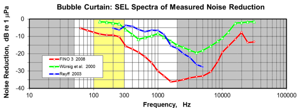
Figure 4: Noise reductions of bubble curtains, [2],Betke (2008).
