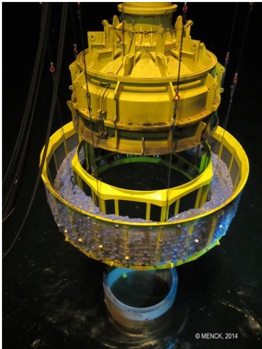
Figure 16. HSD-box hanging below the hammer
