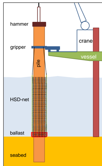
Figure 13. Net below the gripper,[5].
