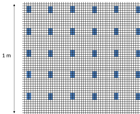
Figure 10. HSD net-layout at ESRA-test in the Baltic Sea in 2011, [5].
