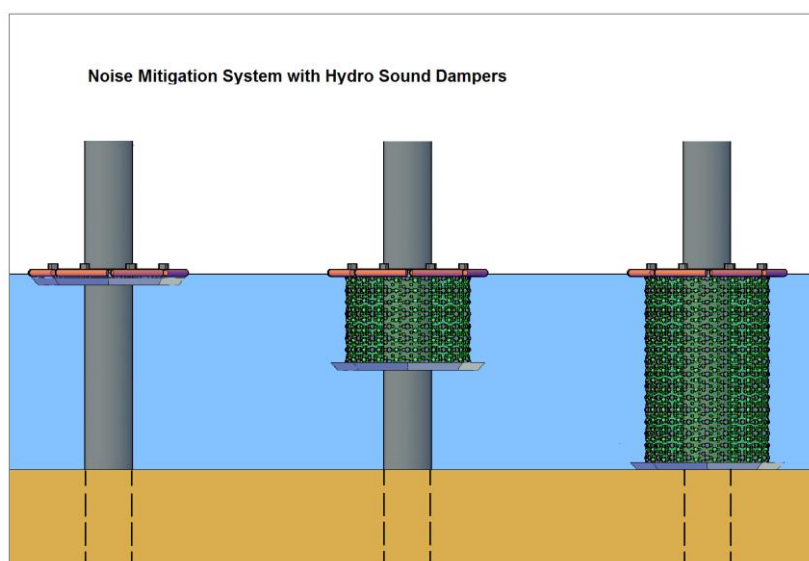
Figure 7. HSD-net enclosed in a donut-like container after Elmer et.al. (2011).
