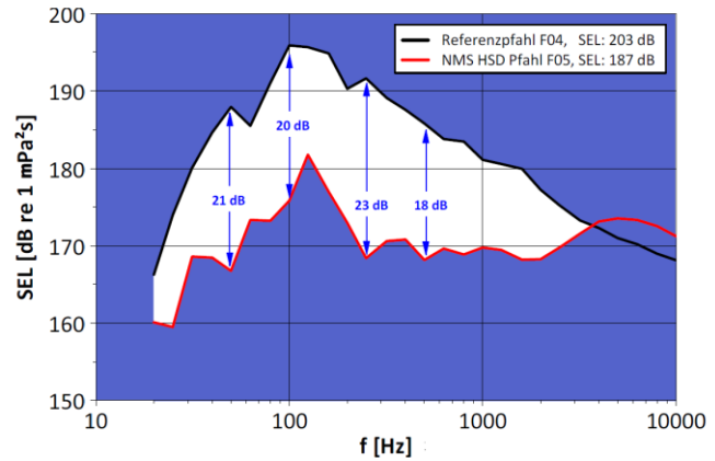
Figure 15. Third octave SEL spectra of underwater piling noise with and without HSD noise mitigation.
