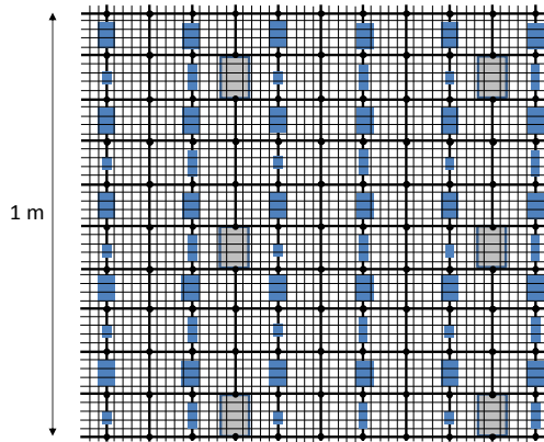
Figure 14. HSD net-layout at London Array test in the North Sea in 2012 after [5].
