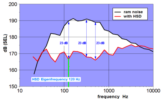
Figure 11. Third octave SEL spectra of underwater piling noise with and without HSD noise mitigation, [5].
