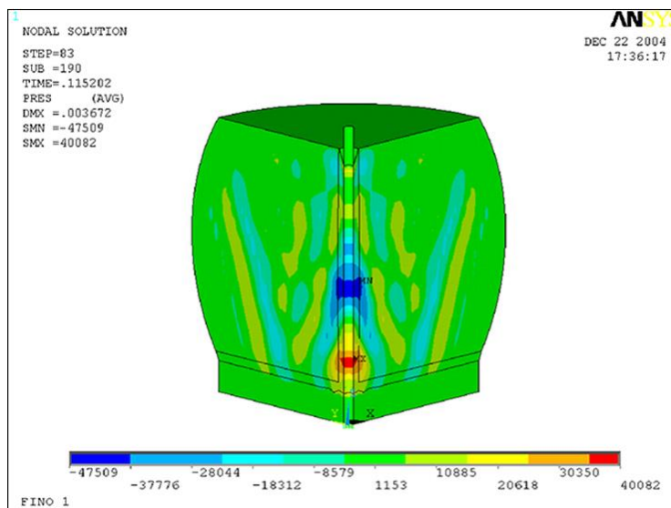
Figure 2. Travelling impact wave within the pile inducing uw-sound waves and reflections, Elmer et. al. (2007)
