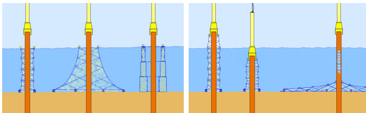
Figure 5: Staggered HSD-net, large fishing net and telescopic frames after [1], Elmer (2010).
