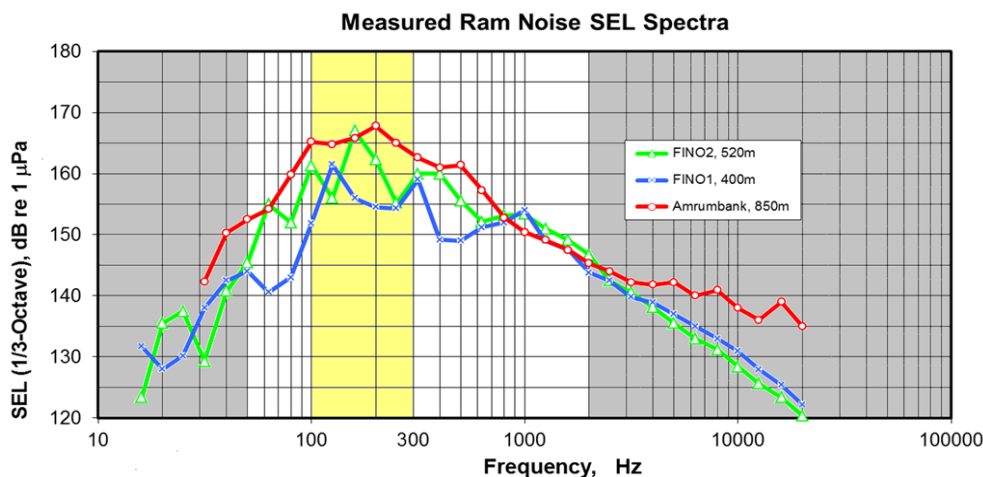
Figure 3: Third octave spectra of measured underwater noise of offshore projects, [2],Betke (2008)
