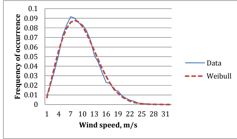
Figure AA.4: Typical frequency of occurrence of wind speeds, based on data and statistical model
