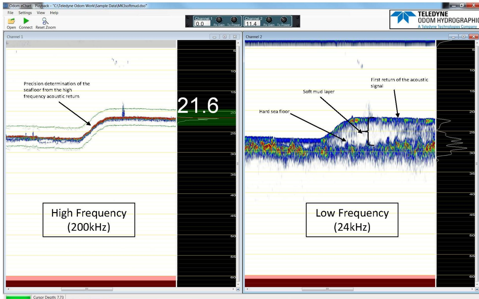
Example of a digital screenshot of dual frequency singlebeam echo sounder traces By Mredmayne (Own work) [CC BY-SA 3.0 ( http://creativecommons.org/licenses/by-sa/3.0/ )], via Wikimedia Commons
