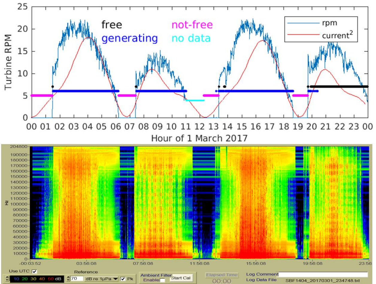
Figure 10. Top plot shows turbine operations on 1 March 2017. The turbine revolutions per minute (RPM) are also plotted along with the square of the modelled current speed. Bottom plot shows a Lucy spectrogram of hydrophone 1404 measurements over the same 24-hour period.
