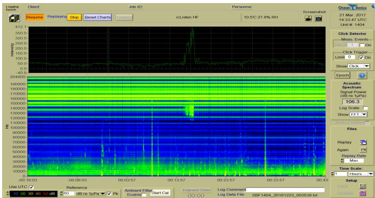
Figure 2. Screenshot from Lucy. Dec. 23, 2016. Reference 60 dB re 1µPa with a 10 dB step. Porpoise clicks are shown in the middle of the spectrogram with the detection intensity spiking in the upper graph. Horizontal banding from 120 to 204 kHz is found throughout the spectrogram, the sound was created by the sonar impulse signals. This shows the Lucy Click Detection software can identify porpoise clicks while there are sonar signals present.
