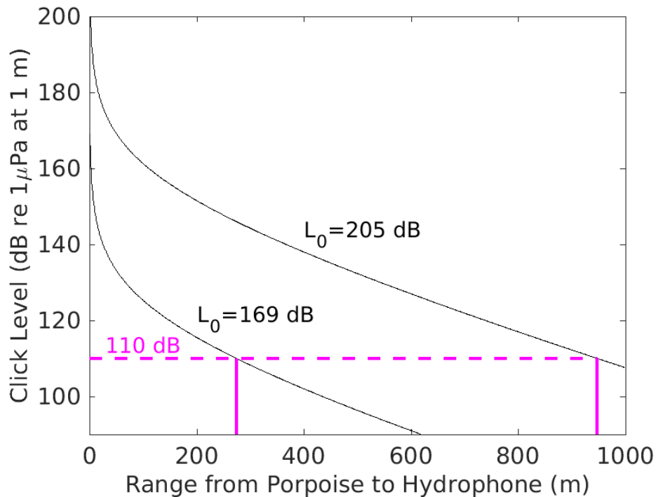
Figure 11. Sound level of porpoise clicks with source levels 205 and 169 dB re 1\mu\text{Pa} at a reference range of 1 m. Sound level falls with range due to radial spreading and attenuation of 37.5 dB/km. Ranges are shown corresponding to a 110 dB lower limit for click detection.
