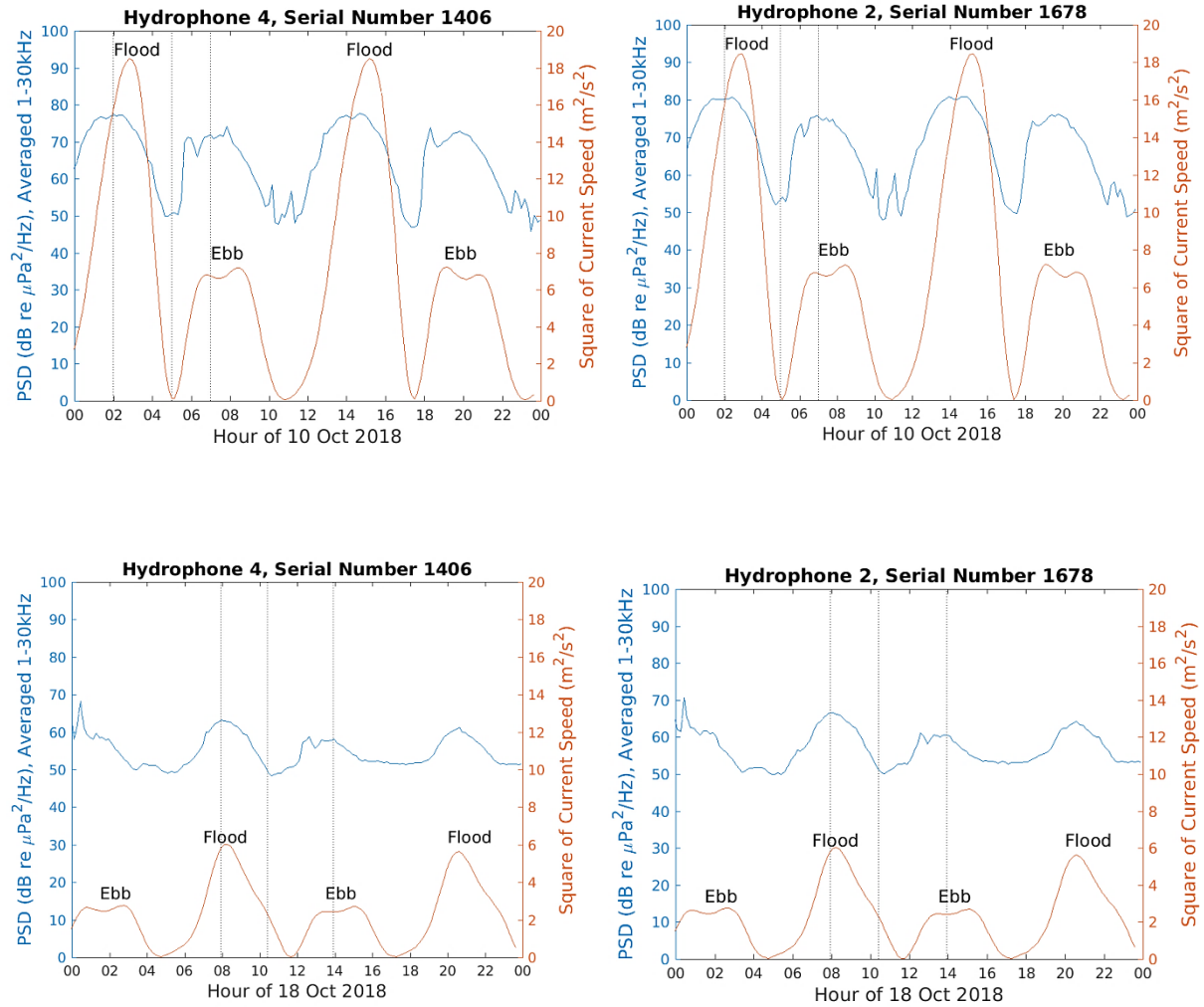
Figure 5. TOP: Sound and squared current speed on 10 October 2018 during a spring tide. BOTTOM: Sounds and squared current speed on 18 October 2018 during a neap tide. Sound is the power spectral density (PSD) averaged over the frequency range 1-30 kHz.
