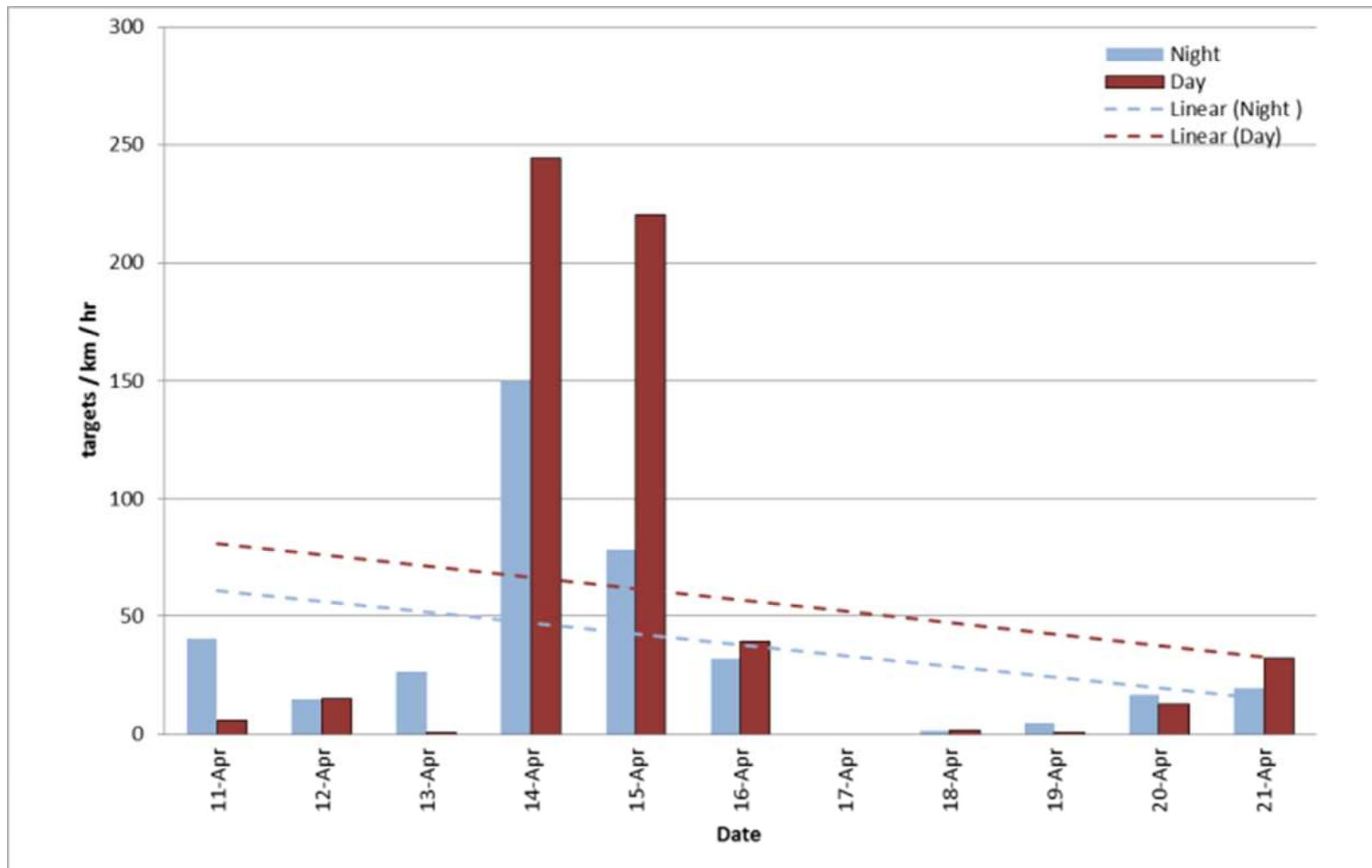
Figure 2.6 Onshore TPRs during the spring 2010 sampling period
