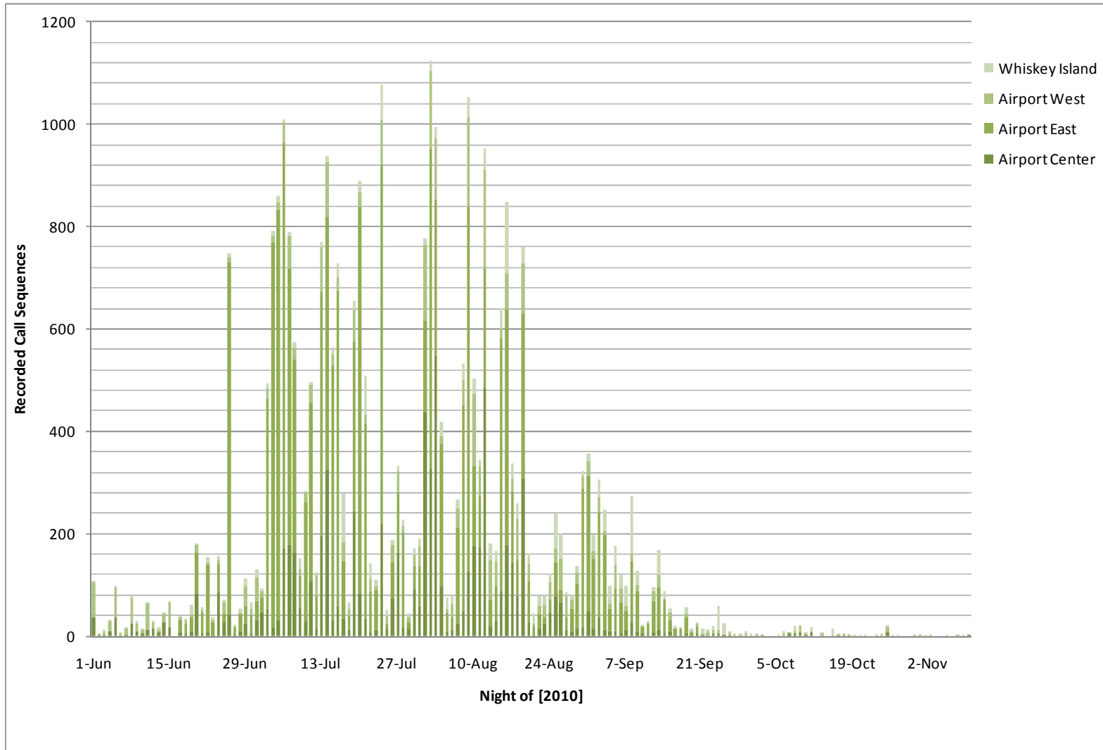
Figure D.12 Total number of bat call sequences recorded per night by the onshore detectors, fall 2010
