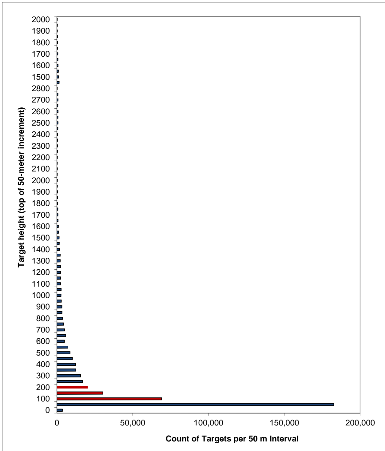
Figure 2.12 Number of offshore targets, spring and fall 2010
