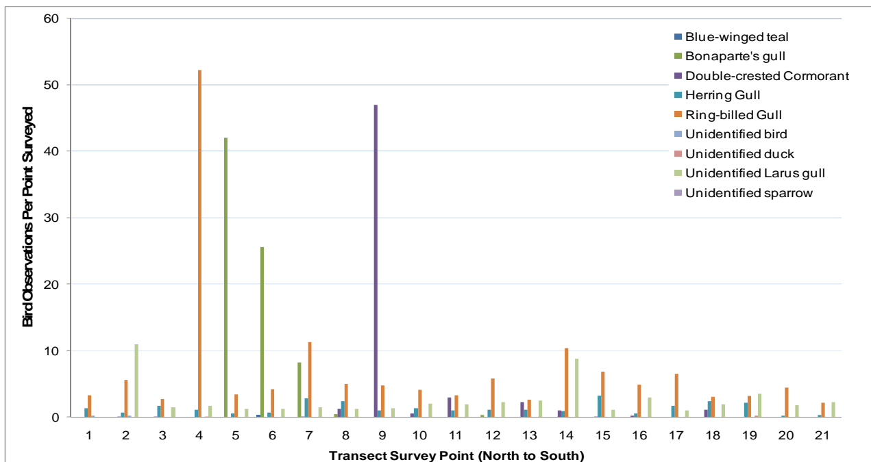
Figure 3.3 Species observation rate per transect survey point location, spring and fall 2010
