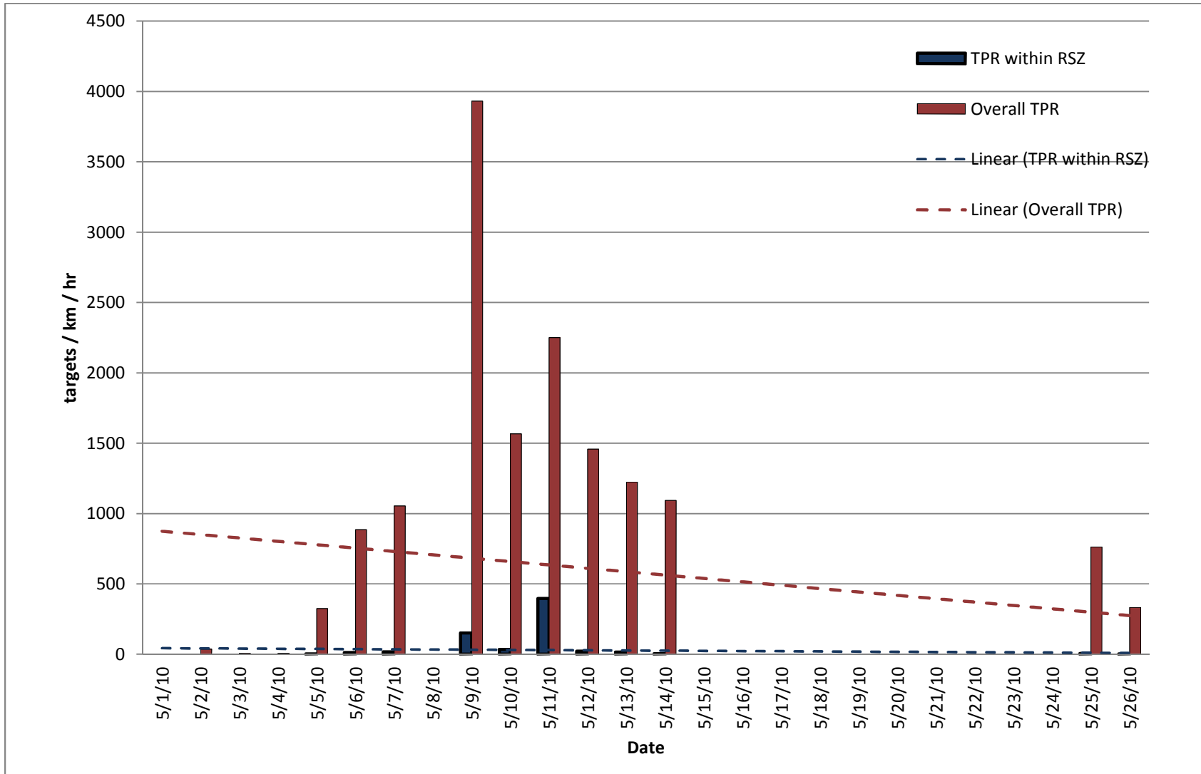
Figure 2.9 Overall offshore TPR and TPR within RSZ during spring 2010
