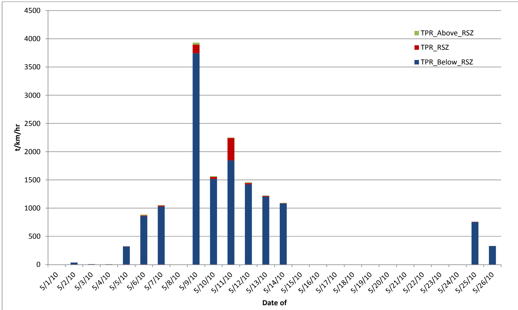
Figure 2.13 Overall spring offshore TPR by date and in relation to the RSZ
