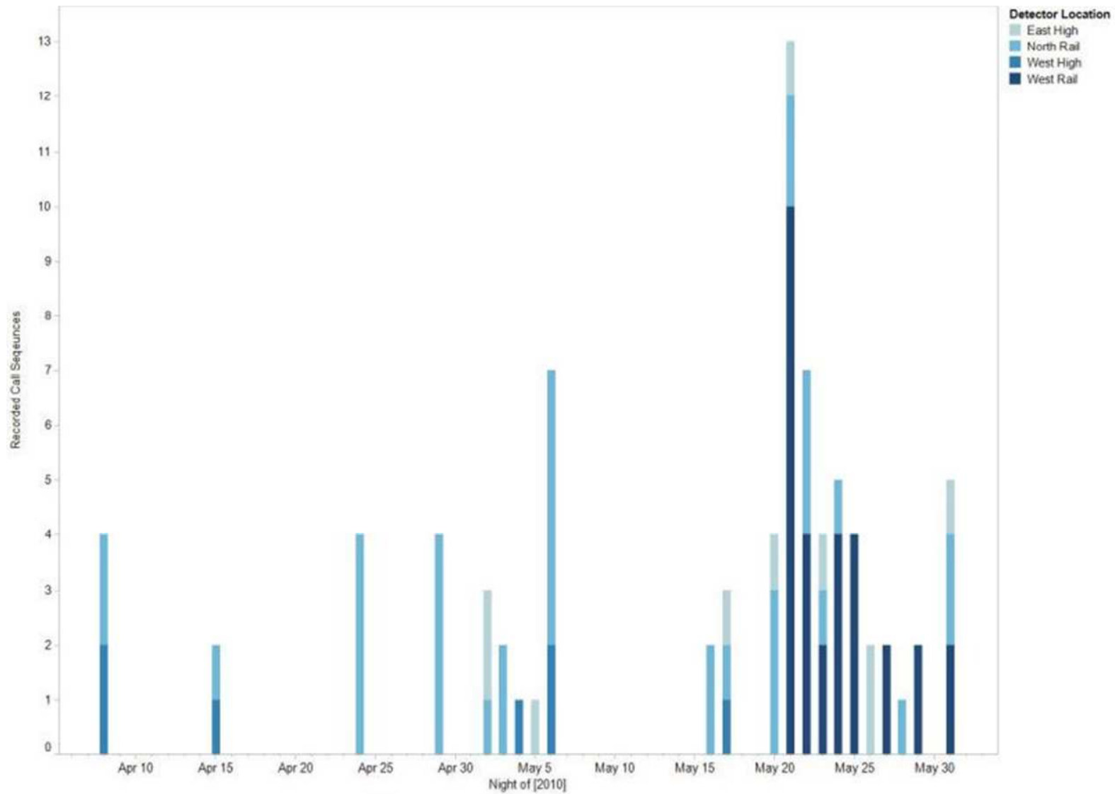
Figure D.10 Total number of bat call sequences recorded per night by the offshore detectors, spring 2010
