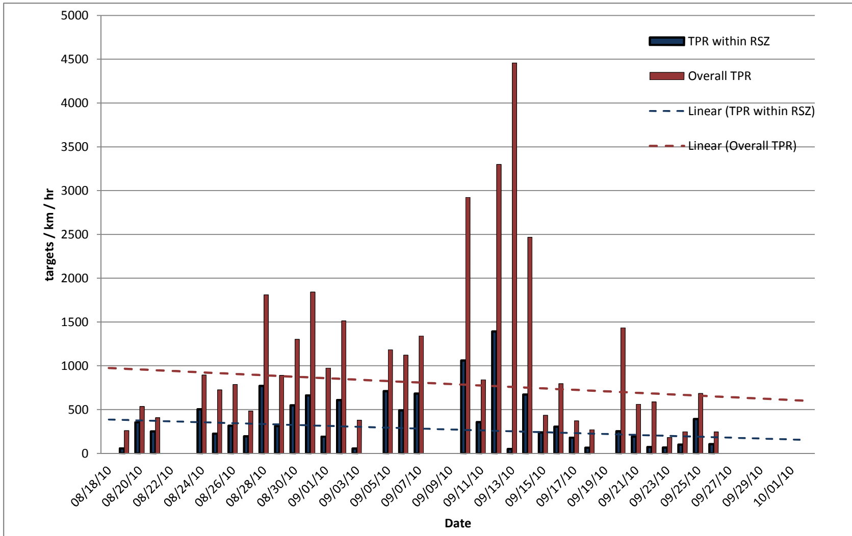
Figure 2.10 Overall offshore TPR and TPR within RSZ during fall
