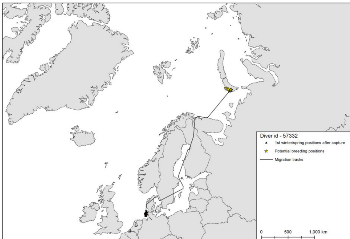
Figure A.4 Migration track of red-throated diver id-52332 covering the period between 11 April 2017 and 30 July 2017.
