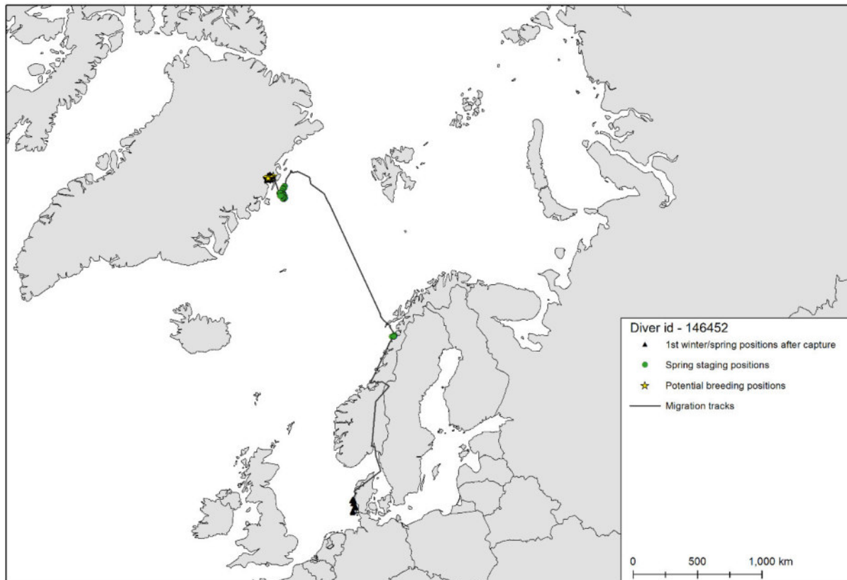
Figure A.18 Migration track of red-throated diver id-146452 covering the period between 04 May 2015 and 04 September 2015.
