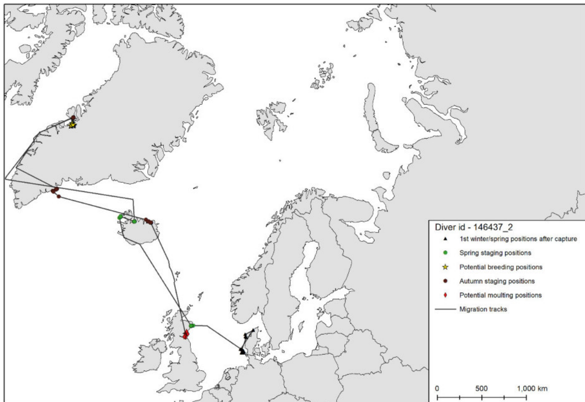
Figure A.9 Migration track of red-throated diver id-146437_2 covering the period between 05 May 2015 and 05 December 2015.
