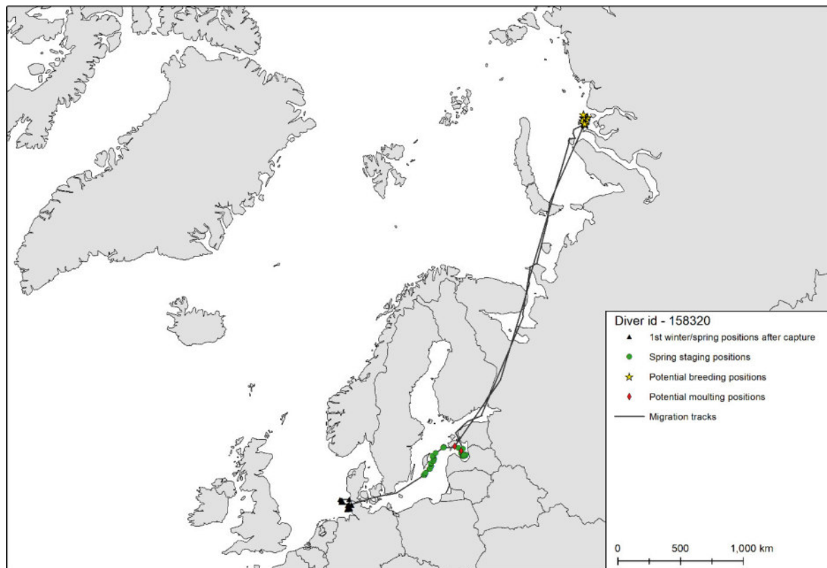
Figure A.23 Migration track of red-throated diver id-158320 covering the period between 27 March 2016 and 07 November 2016.
