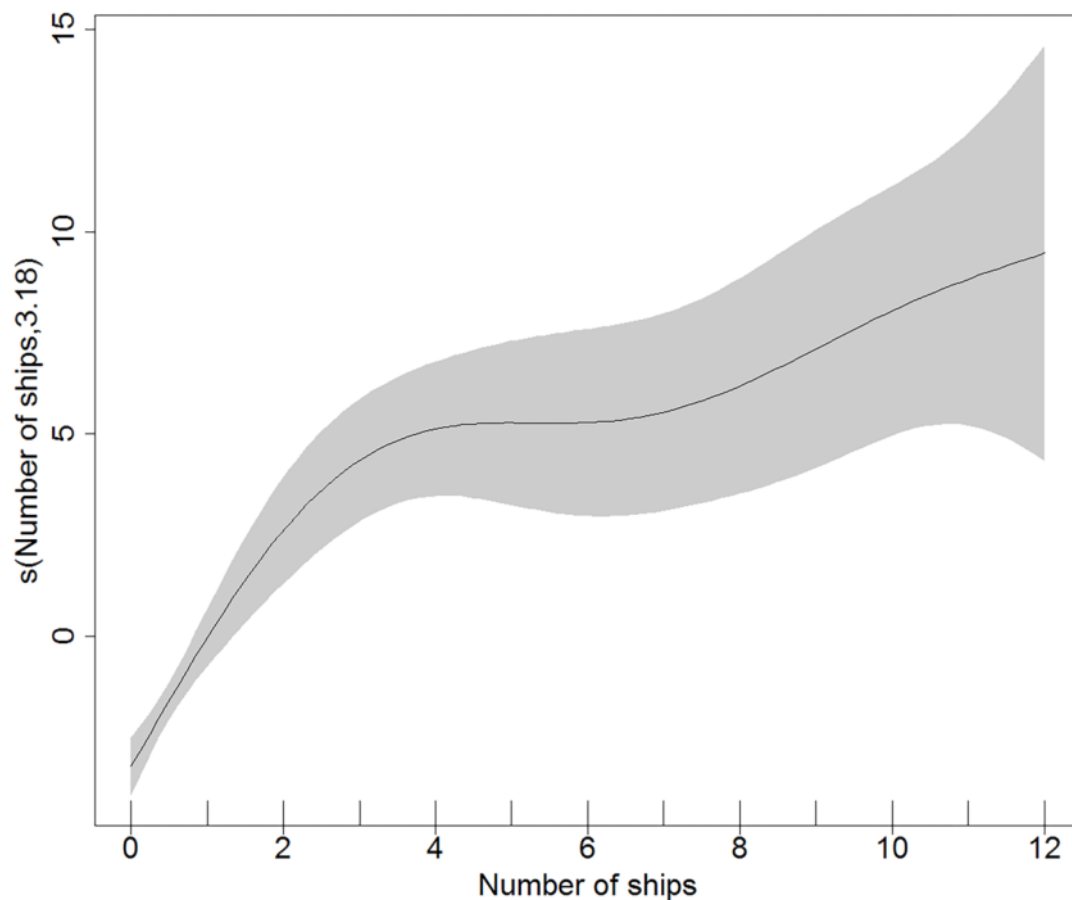
Figure 7.5 Relocation distance of divers relative to the number of ships encountered within a 3 km radius. Smooth curve from fitted GAM with 95% confidence interval (shaded area).
