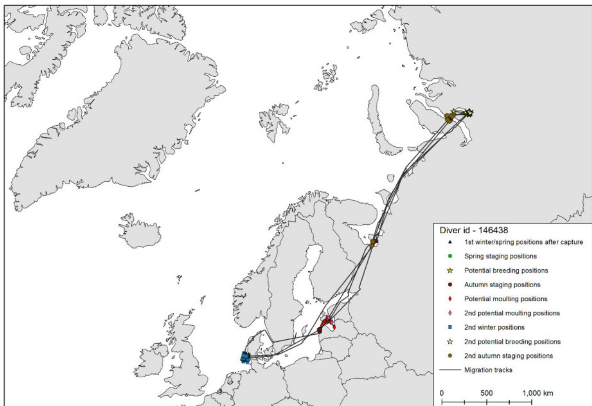
Figure A.10 Migration track of red-throated diver id-146438 covering the period between 05 April 2015 and 17 October 2016.
