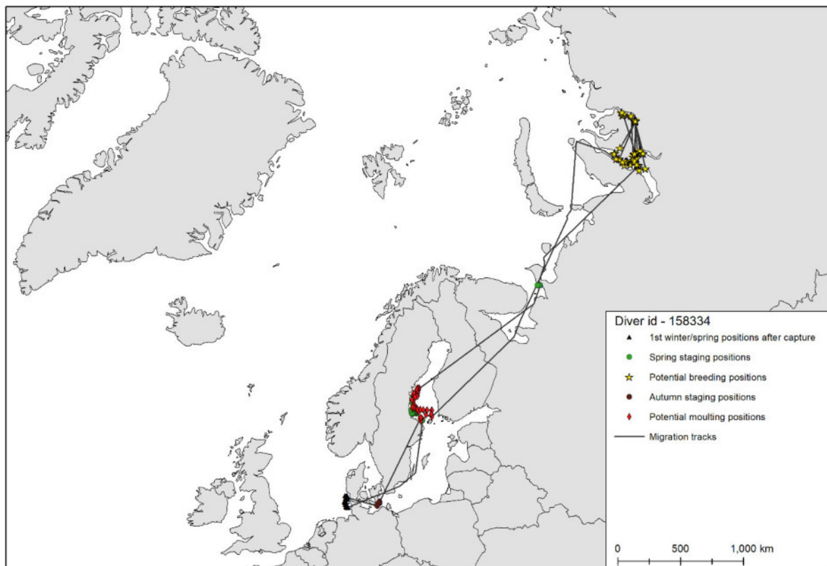
Figure A.34 Migration track of red-throated diver id-158334 covering the period between 27 March 2016 and 13 December 2016.
