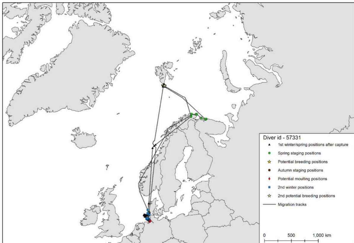
Figure A.3 Migration track of red-throated diver id-52331 covering the period between 12 April 2017 and 06 August 2018.
