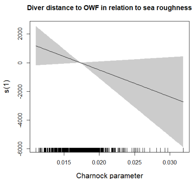
Figure 6.10 GAMM response curve indicating that distance between red-throated divers and OWF has a tendency to decline at higher Charnock parameter values characterising sea surface roughness. This tendency, however, was not statistically significant.
