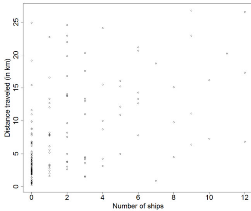
Figure C 9 Bird tracking data: plot of number of ships in a 3 km radius around the bird tracking position and distance travelled by individuals during the subsequent lag.
