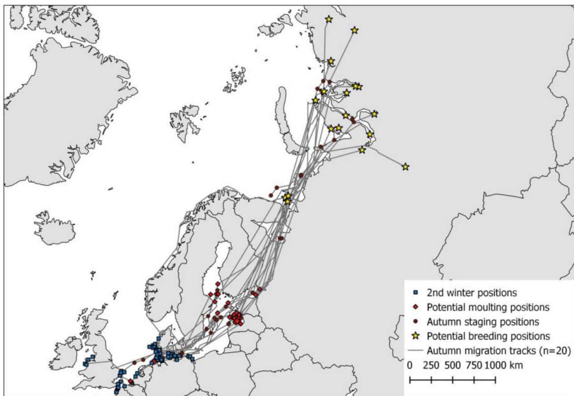
Figure 5.4 Autumn migration tracks and positions of breeding, staging, potential moulting and wintering areas (2 nd winter) of red-throated divers originating from northern Russia. Yellow stars indicate positions in potential breeding areas. Brown dots indicate positions in autumn staging areas, red diamonds indicate positions in potential moulting areas and blue squares indicate positions in wintering areas (2 nd winter). For each identified area of stay the first and last position in the corresponding area is displayed per individual.
