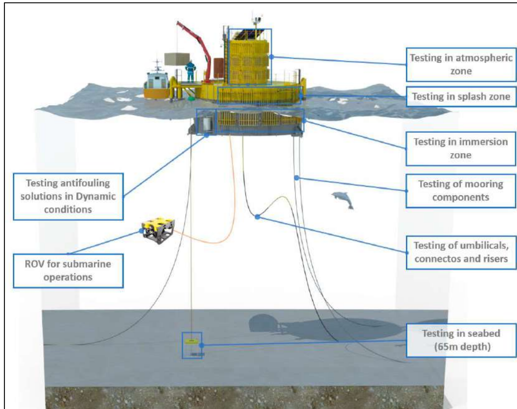
Figure 11. Schematic view of positioning of the mooring system (Source: Tecnalia).
