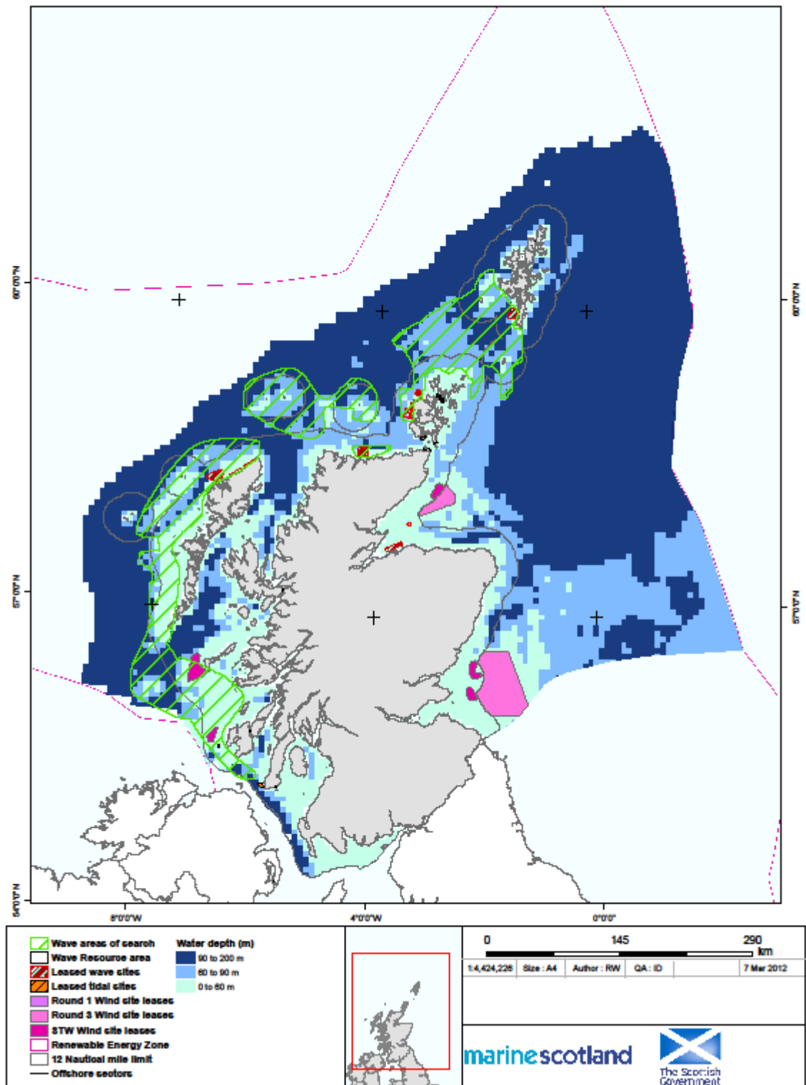
Figure 12 Areas of search for Plan option areas for wave energy development in waters of 0 – 90m depth within the wave power resource area.
