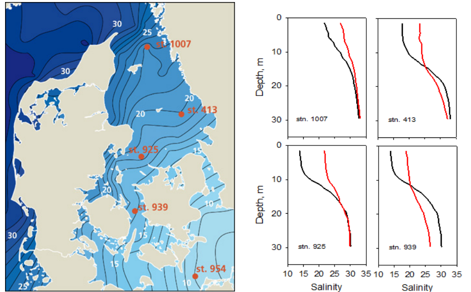
Figure 3.2. Left: Average surface (0-5 m) salinity from January to December. Right: Salinity profiles in winter (red curve) and summer (black curve) at the four monitoring stations marked on the left figure (from Dahl et al., 2003).
