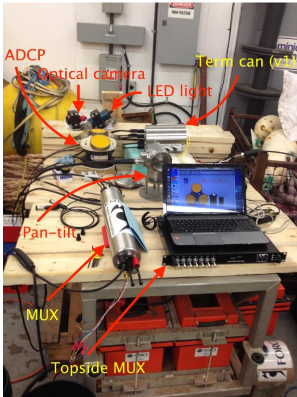
Figure 3: Electrical integration of FAST-EMS. Left: Testing of the sensor suite (Gemini not pictured). Right: Testing with the 1.5 km FO cable and new term can, which houses both power conditioning components and power and fibre connections between the FO cable and MUX.
