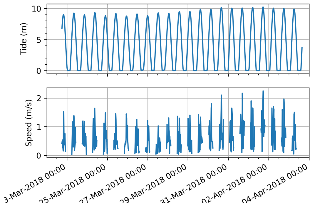
Figure 8: Depth and current speed at 5 metres above seabed, as measured by the AWAC on-board FAST-EMS.
