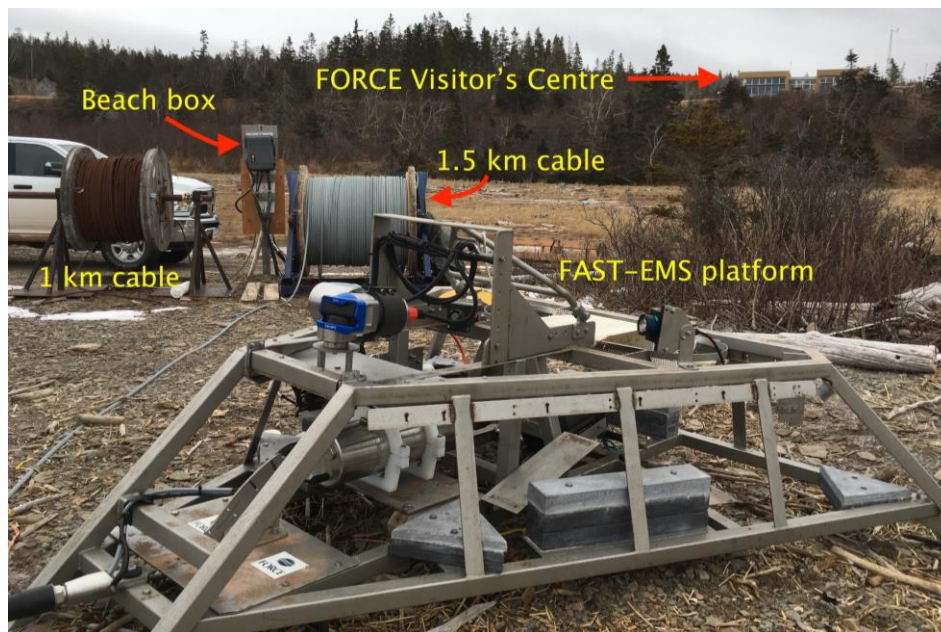
Figure 4: Full FAST-EMS system, including platform and FO cables, connected to the FORCE Shore.
