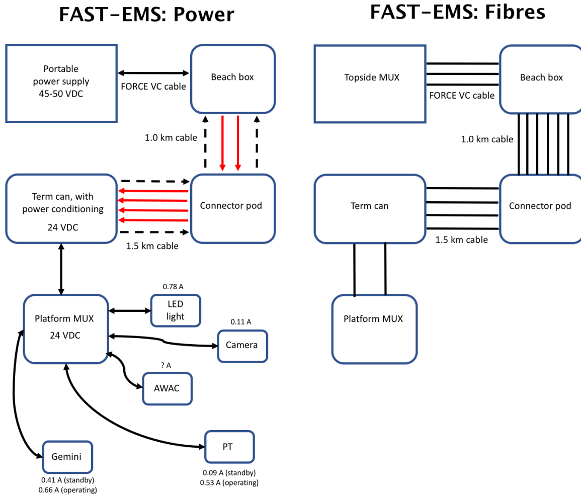
Figure 2: Block diagrams of power and fibre for the FORCE Shore Station-connected FAST-EMS. In the power schematic, current flows through the FO cable's copper cores and returns (ground) through the armour. In the fibre schematic, the number of connecting lines indicates the number of fibre strands (there is one active and one-back up strand for the full system).
