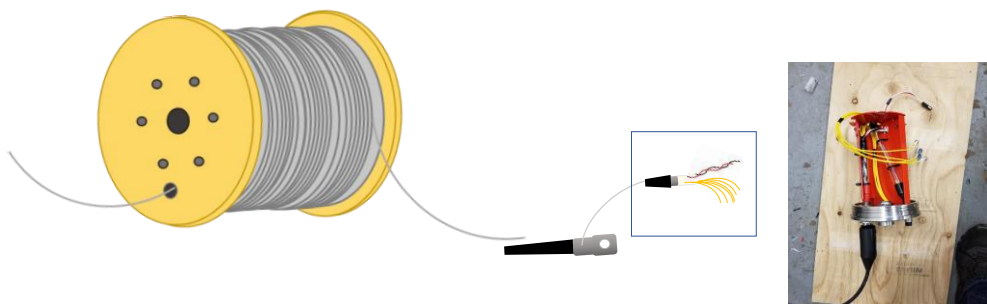
Figure 4: Schematic of cable termination. Left-right: Cable reel, mechanical termination, penetrator with fibre and power broken out (inside of term can, which is not shown), and (photograph of) FORCE's customized fibre termination, capped by ST connectors.
