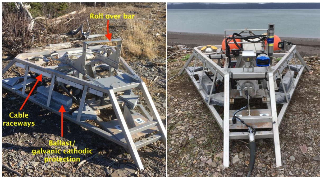
Figure 1: FAST-EMS platform. Left: The 'bare' platform, with ruggedized components. Right: The platform with full sensor suite (cf. Section 3.2). Recovery buoys are the orange spheres in the rear and the Gemini imaging sonar is at front and facing forward.
