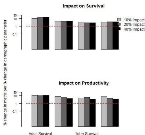
Figure 50. Percentage change in the change in probability of the population declining by 25% per percentage change in adult survival, immature survival, first year survival and productivity for offshore wind farm impacts on survival and productivity from stochastic models. Data tabulated in Tables 35 and 36.
