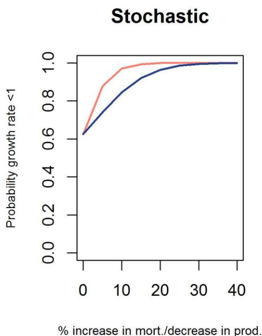
Figure 34. Impact of up to a 40% increase in mortality (red line) or up to a 40% decrease in productivity on the probability (blue line) of the growth rate of a population of seabirds with an r-selected life history strategy and a stable population trajectory.
