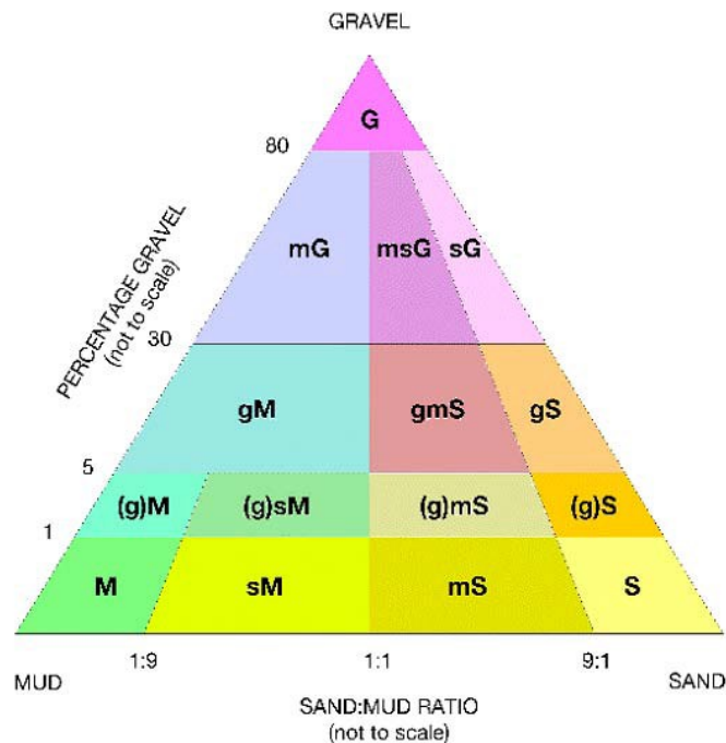
Figure A 11-2. Modified sediment classification scheme used in BGS dataset DiGSBS250k displaying the sand:mud:gravel ratios of sediment types present at the study locations. Abbreviation meanings are given in Table A 11-3.
