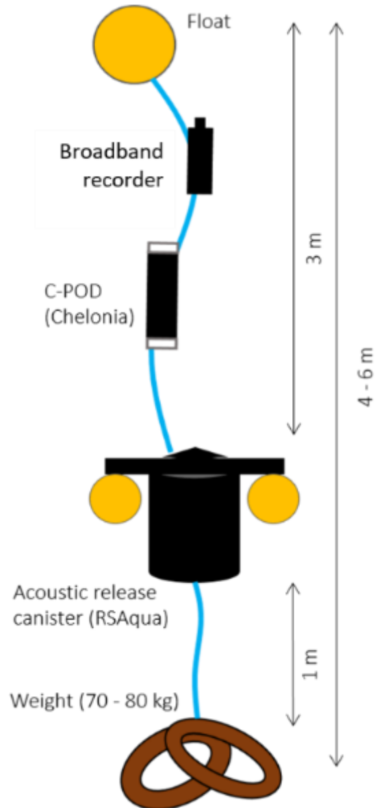
Figure A 10-1. Mooring schematics following the design by Quer et al. (2023).
