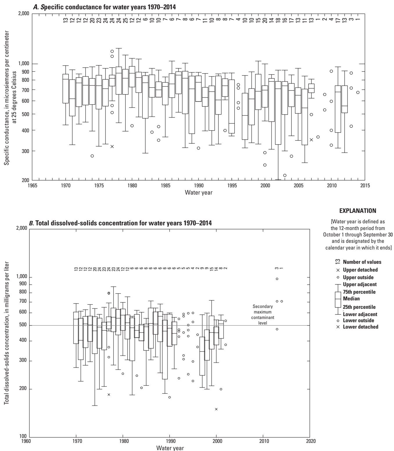
Figure 36. Annual variability in values of constituents for the Yellowstone River near Sidney, Montana (streamgage 06329500), from 1970 to 2014. A , specific conductance, in microsiemens per centimeter at 25 degrees Celsius; B , total dissolved solids, in milligrams per liter; C , pH, in standard units; D , sulfate, in milligrams per liter; and E , chloride, in milligrams per liter.
