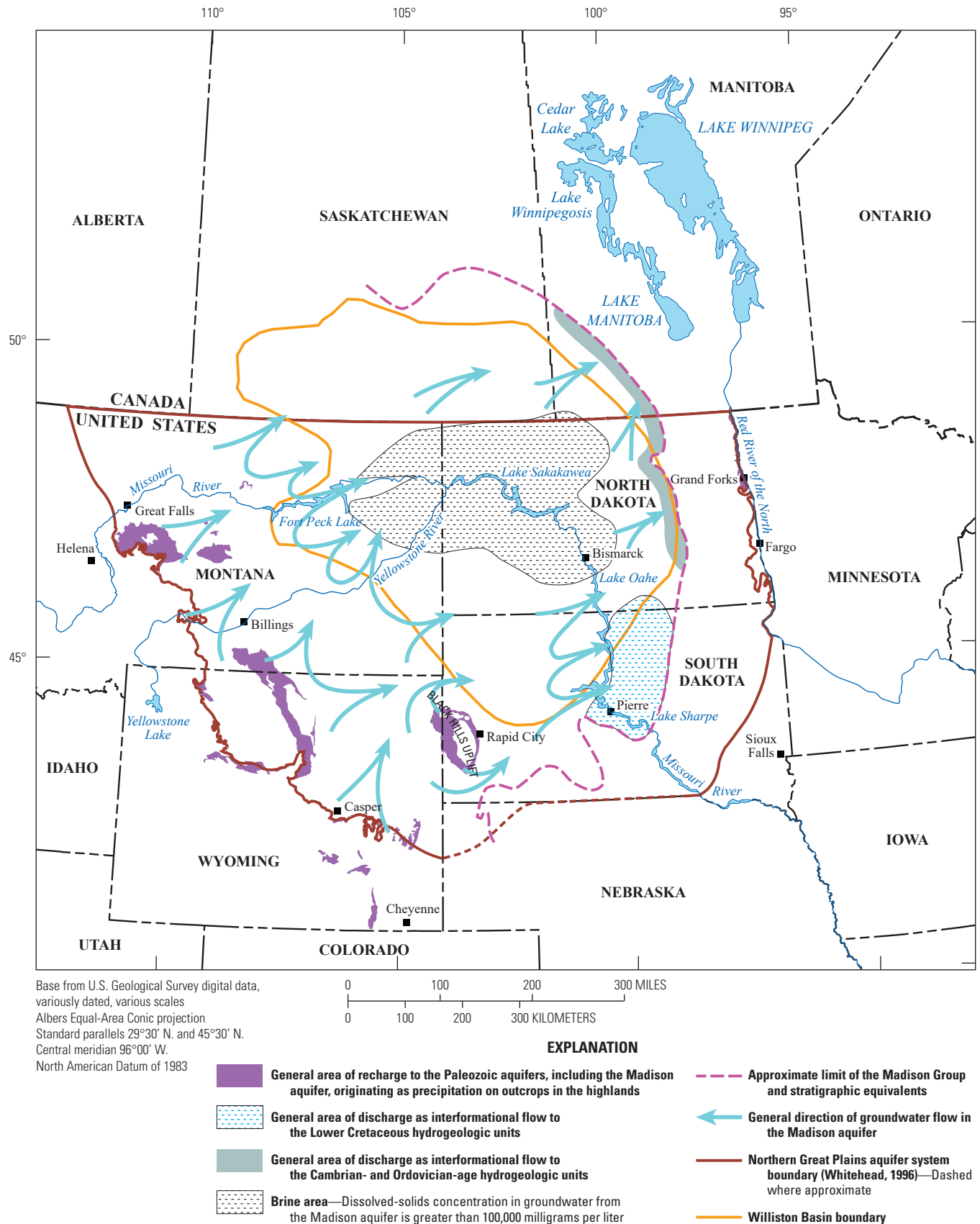
Figure 13. General areas of recharge to the Paleozoic aquifers/aquifer systems, and general direction of groundwater flow in, and discharge from, the Madison aquifer in the Williston Basin and adjacent areas, United States and Canada (modified from Downey and Dinwiddie, 1988).
