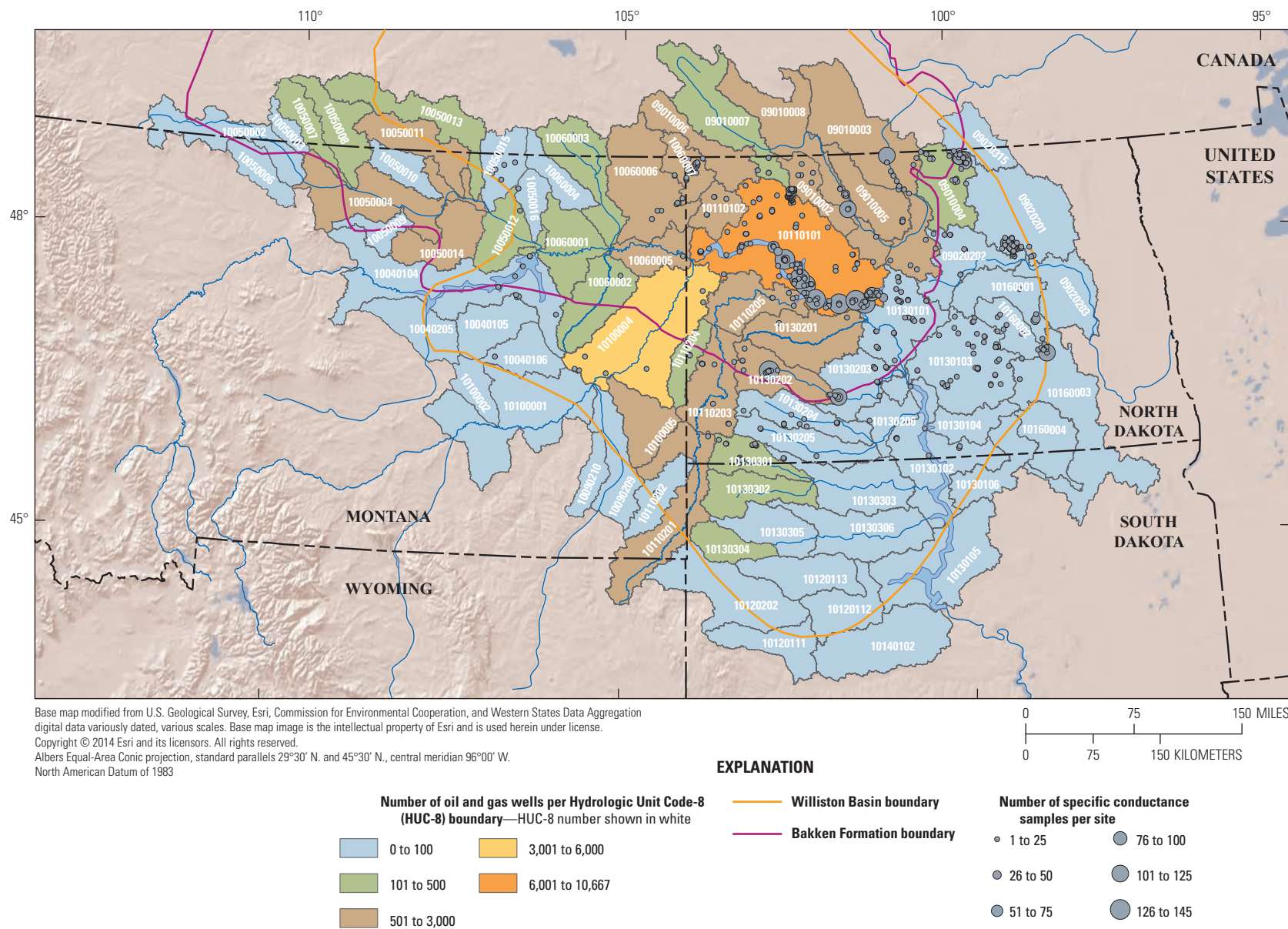
Figure 41. Spatial distribution of specific conductance samples from lakes and reservoirs and numbers of oil and gas wells in hydrologic unit code-8 (HUC-8) watersheds in the Williston Basin in Montana, North Dakota, and South Dakota, from 1970 to 2014.
